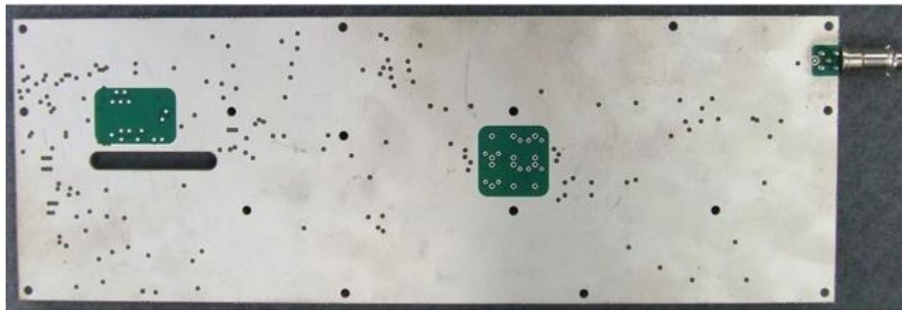
Photograph 20: Receiver Board (RXB) – Bottom
