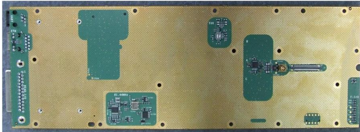
Photograph 17: Reciter Control Board (RCB) – Bottom
