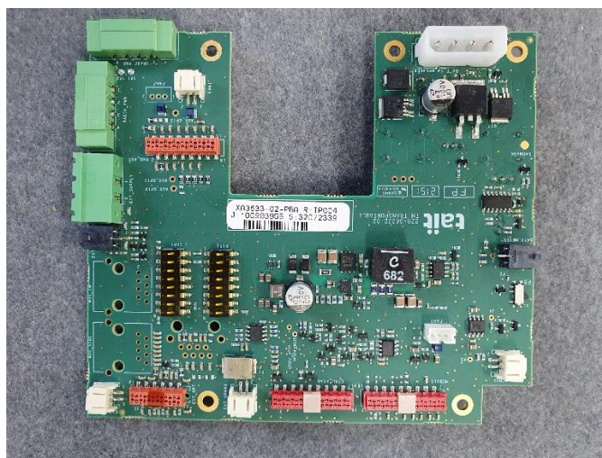
Photograph 23: Interface Board – Front
