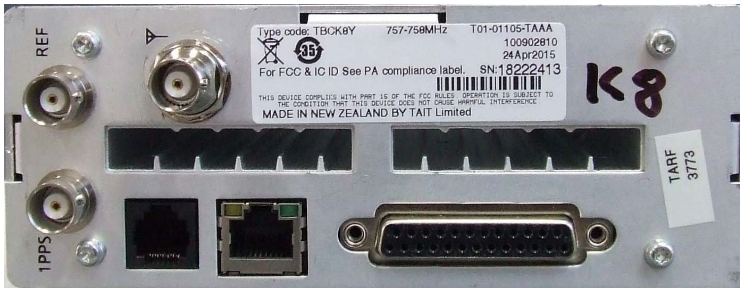
Photograph 03: Reciter module – Rear panel
