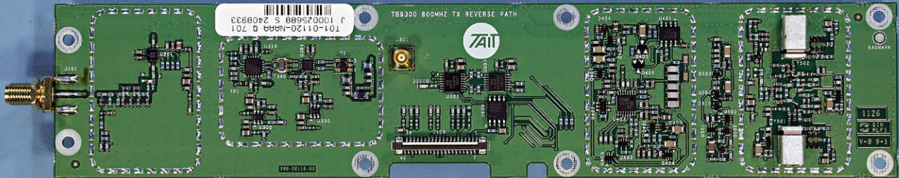
Reciter Transmit Reverse PCB Top View
