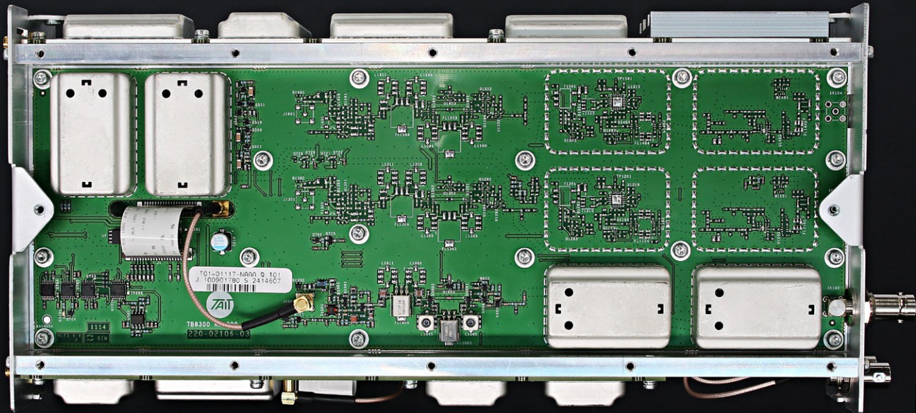
Reciter Rx Single Board Cans On
