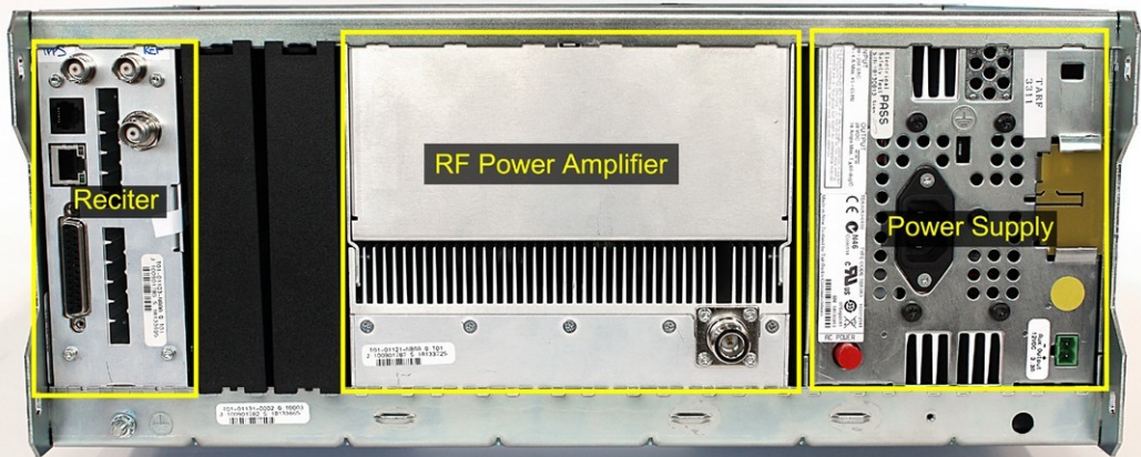
TB9400 Base Station Rear Annotated View
