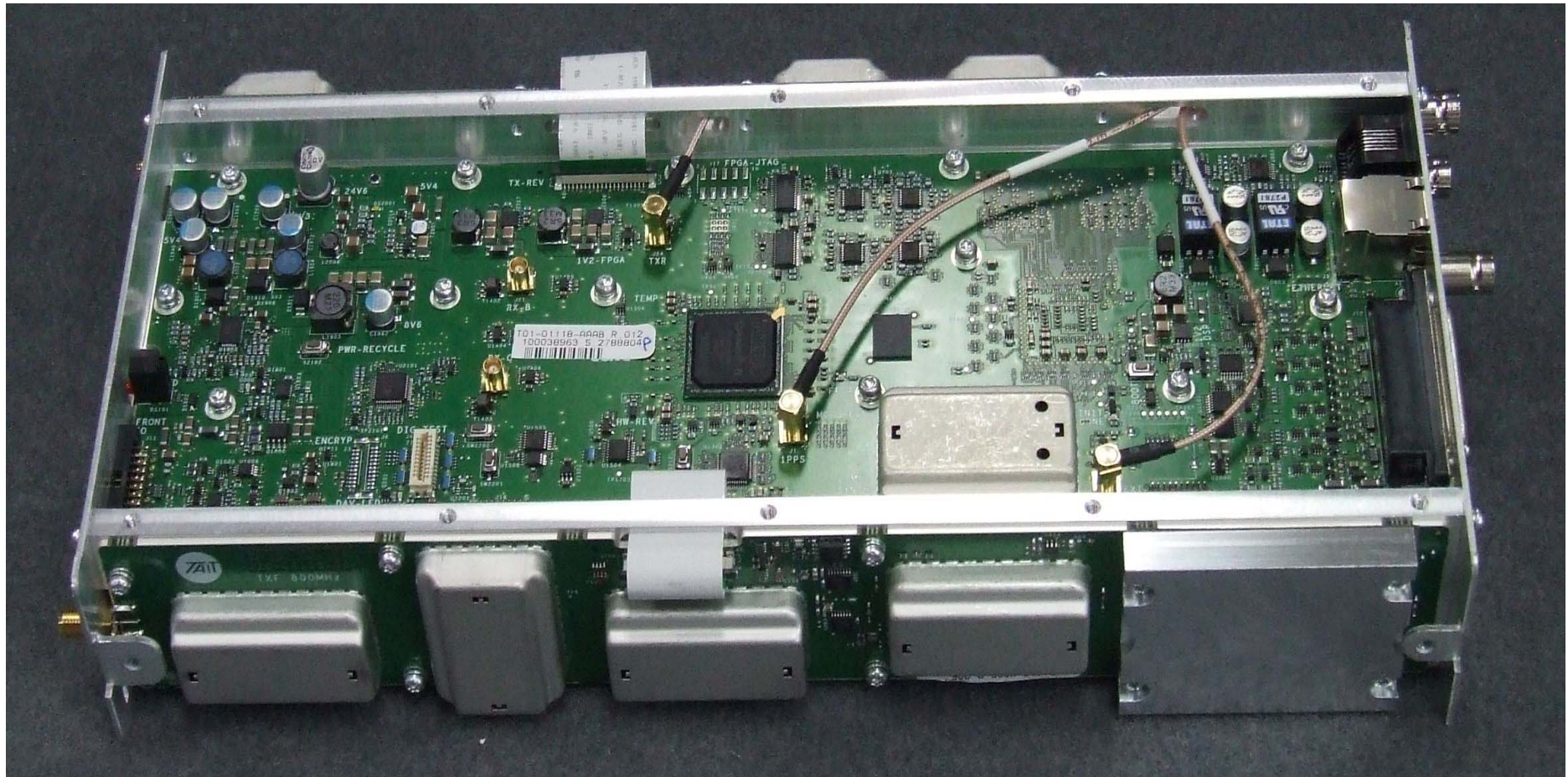
Photograph 07: Control PCB – Top
