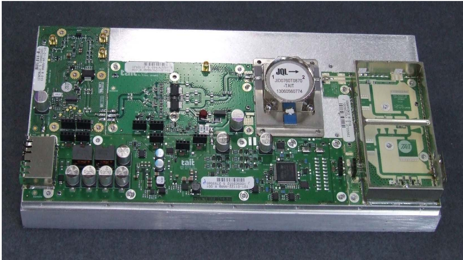
Photograph 02: 50W PA modules – Top. Shields Removed
