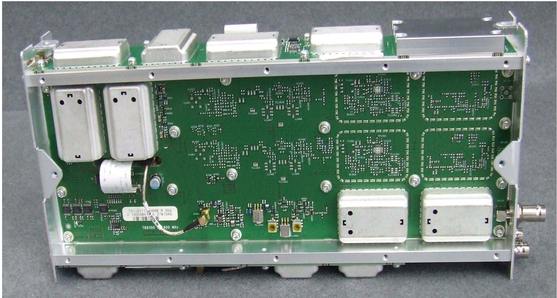
Photograph 04: Rx PCB - Top
