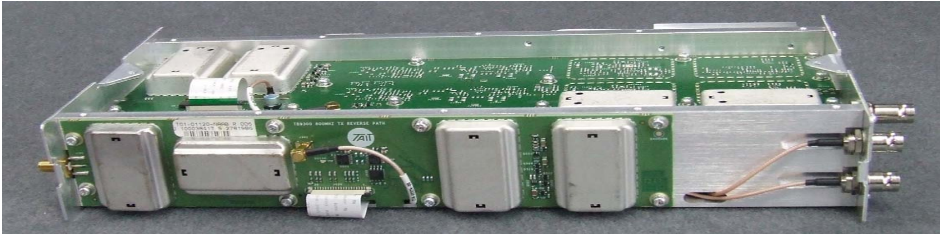
Photograph 13: TXR PCB – Top
