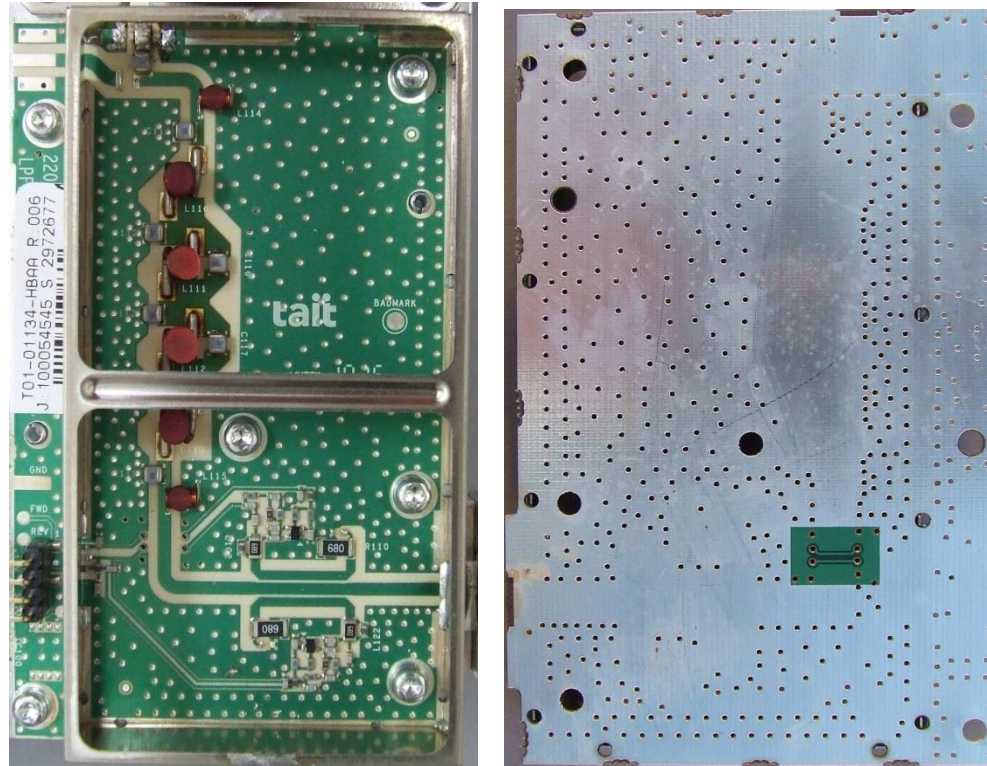
Photograph 29 & 30: Power Amplifier LPF PCB – Top & Bottom
