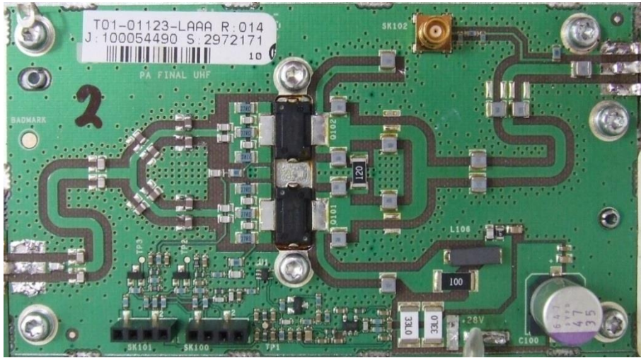
Photograph 23 & 24: Power Amplifier 60W PA 2 PCB – Top & Bottom
