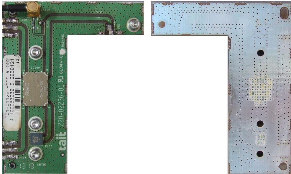
Photograph 25 & 26: Power Amplifier Combiner PCB – Top & Bottom
