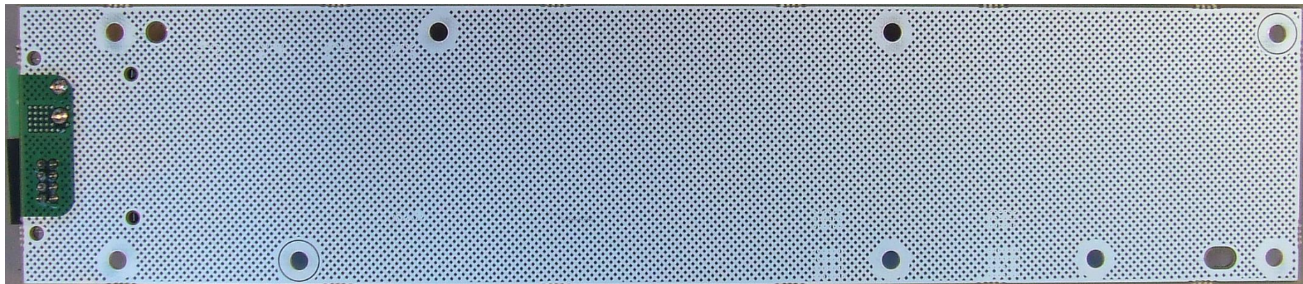
Photograph 31 & 32: Power Amplifier Control PCB – Top & Bottom
