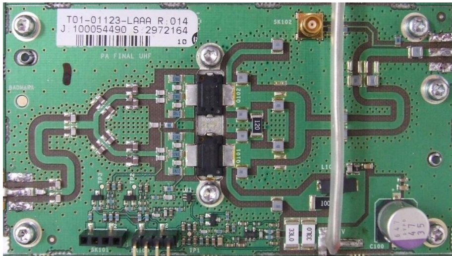
Photograph 21 & 22: Power Amplifier 60W PA 1 PCB – Top & Bottom
