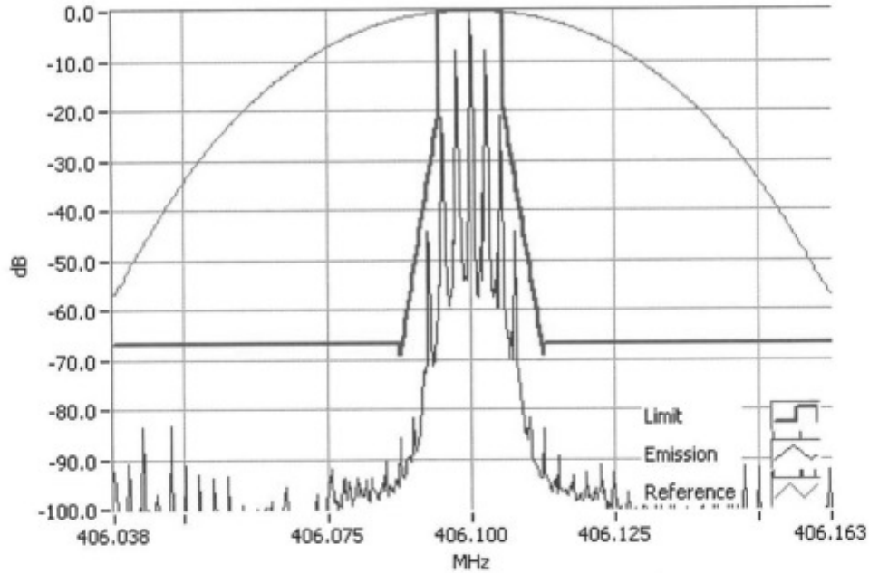
Analogue Modulation 406.1000MHz Mask D 50W RBW=100Hz, VBW=1000Hz, Detector Mode=Peak Result=Pass
