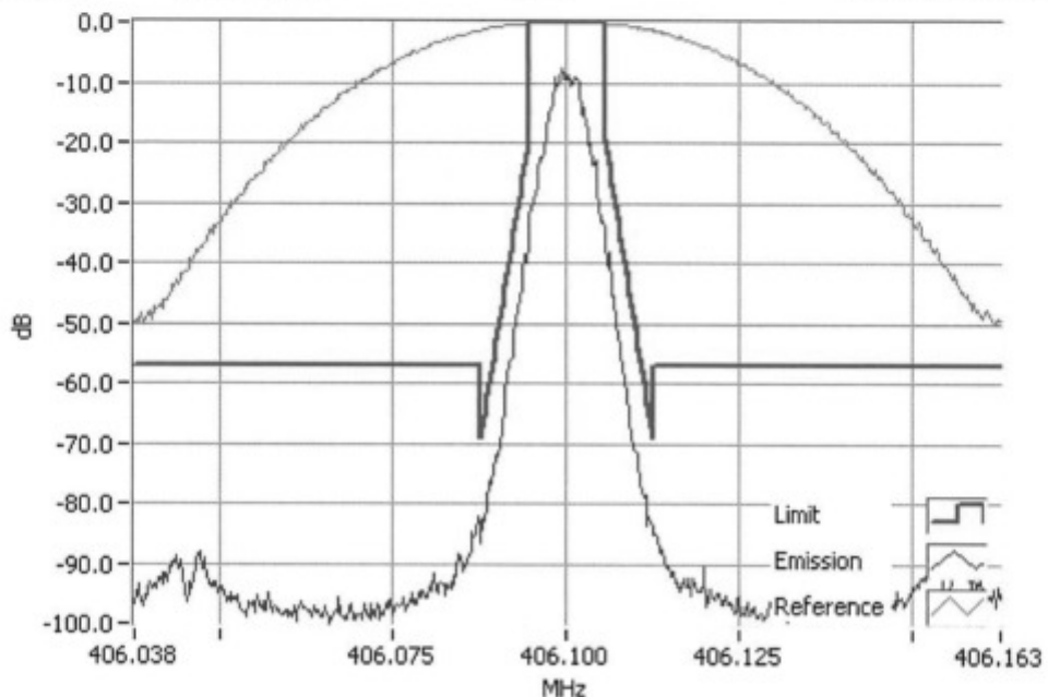
P25 Ph I C4FM 406.1000MHz Mask D 5W RBW=100Hz, VBW=1000Hz, Detector Mode=Peak Result=Pass
