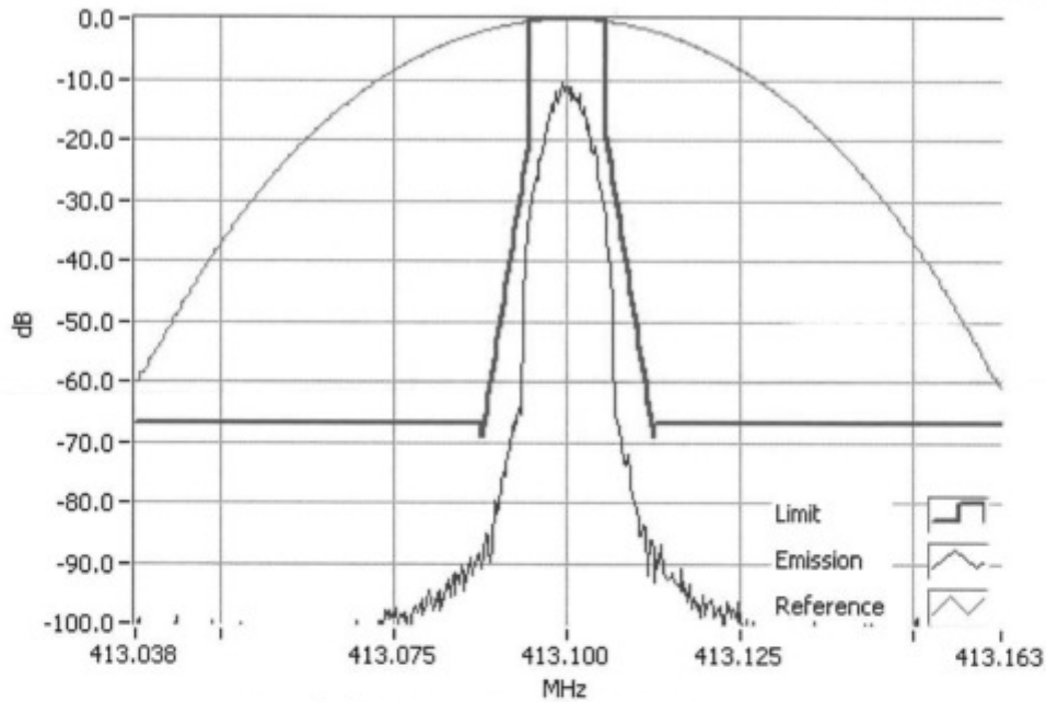
P25 Ph I LSM 413.1000MHz Mask D 50W RBW=100Hz, VBW=1000Hz, Detector Mode=Peak Result=Pass
