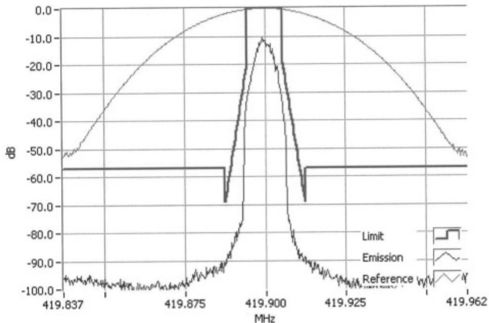
P25 Ph I LSM 419.9000MHz Mask D 5W RBW=100Hz, VBW=1000Hz, Detector Mode=Peak Result=Pass
