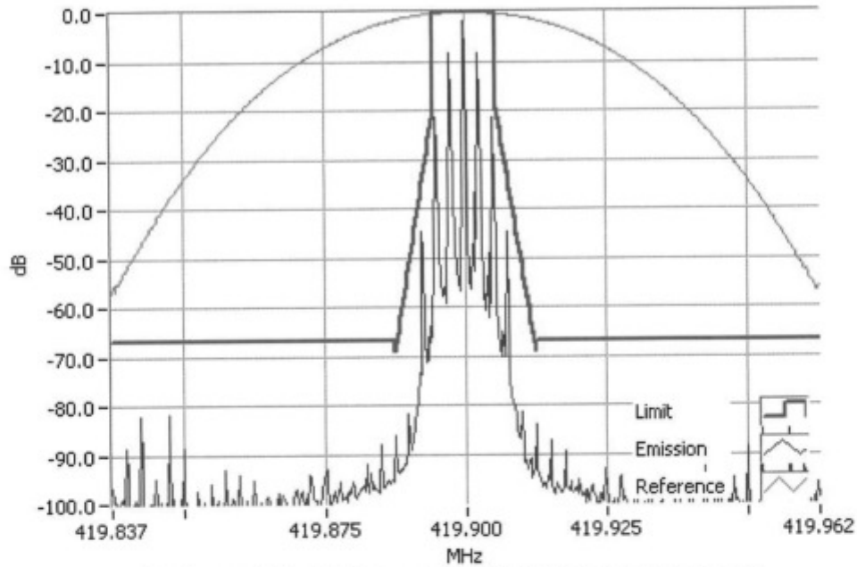
Analogue Modulation 419.9000MHz Mask D 50W RBW=100Hz, VBW=1000Hz, Detector Mode=Peak Result=Pass
