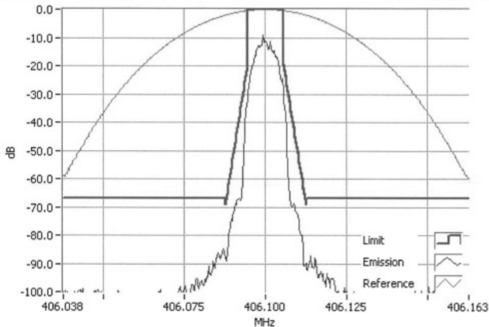
P25 Ph II H-DQPSK 406.1000MHz Mask D 50W RBW=100Hz, VBW=1000Hz, Detector Mode=Peak Result=Pass
