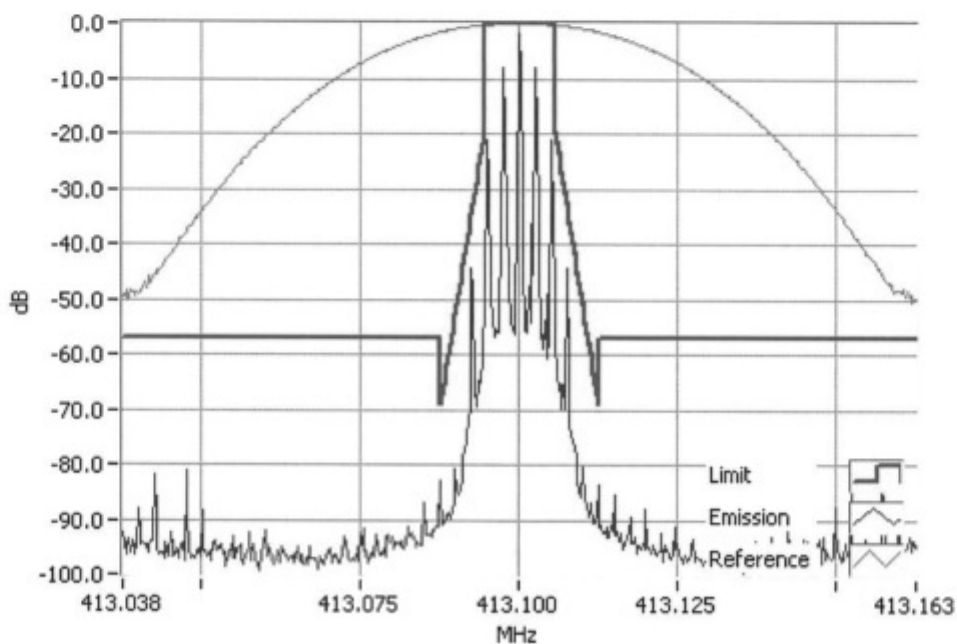
Analogue Modulation 413.1000MHz Mask D 5W RBW=100Hz, VBW=1000Hz, Detector Mode=Peak Result=Pass
