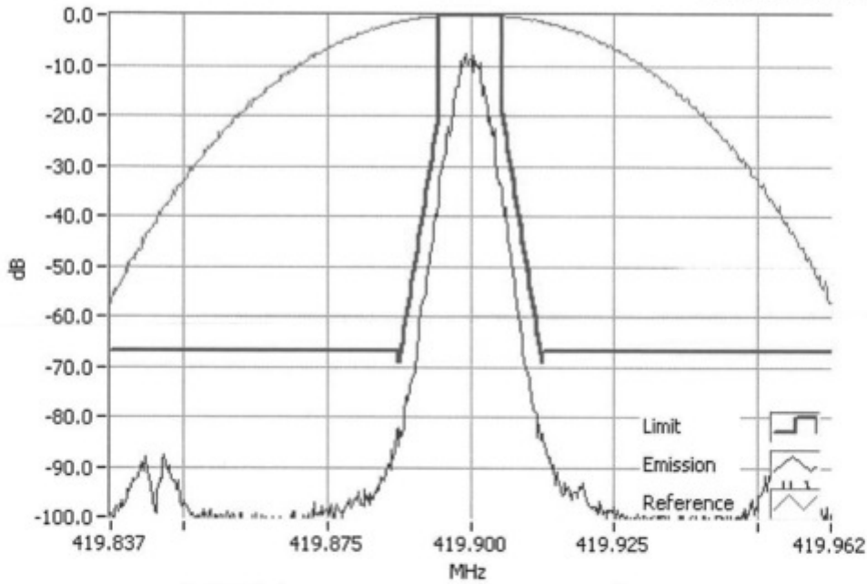
P25 Ph I C4FM 419.9000MHz Mask D 50W RBW=100Hz, VBW=1000Hz, Detector Mode=Peak Result=Pass
