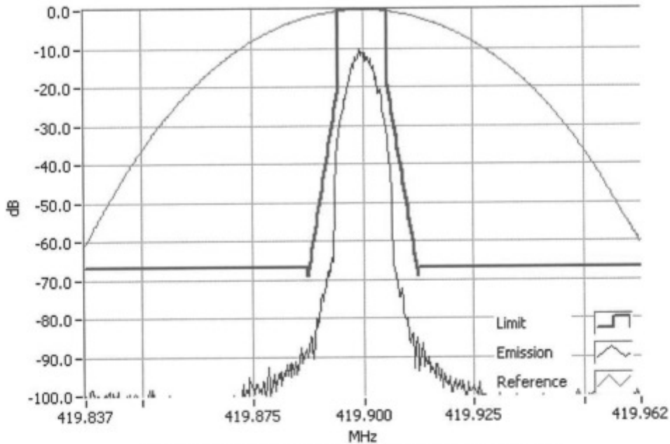
P25 Ph I LSM 419.9000MHz Mask D 50W RBW=100Hz, VBW=1000Hz, Detector Mode=Peak Result=Pass
