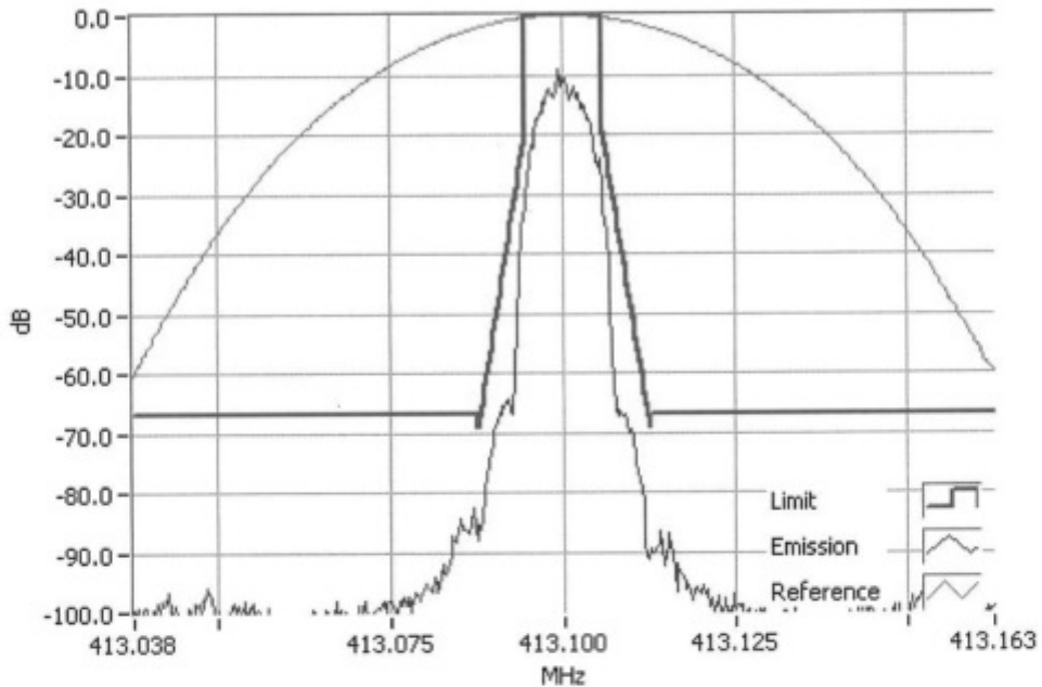
P25 Ph II H-DQPSK 413.1000MHz Mask D 50W RBW=100Hz, VBW=1000Hz, Detector Mode=Peak Result=Pass
