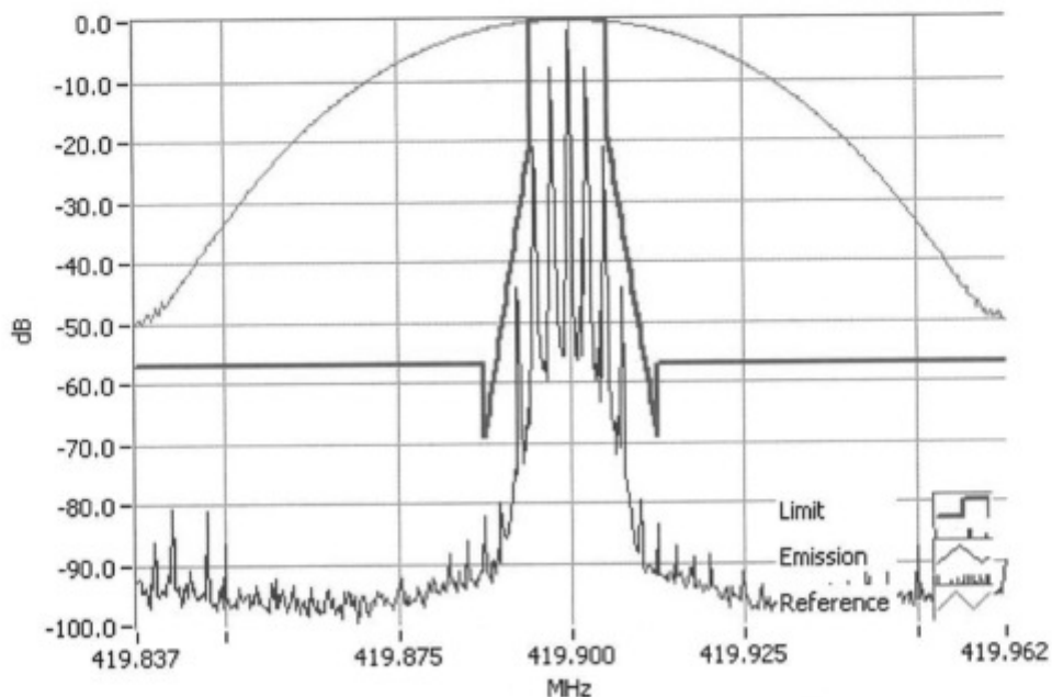
Analogue Modulation 419.9000MHz Mask D 5W RBW=100Hz, VBW=1000Hz, Detector Mode=Peak Result=Pass
