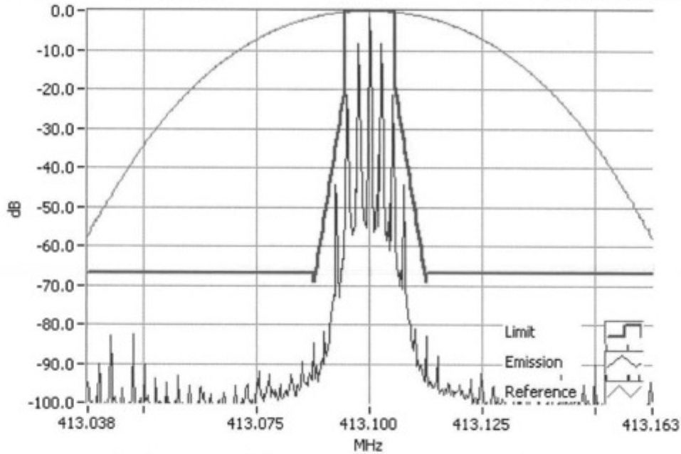
Analogue Modulation 413.1000MHz Mask D 50W RBW=100Hz, VBW=1000Hz, Detector Mode=Peak Result=Pass
