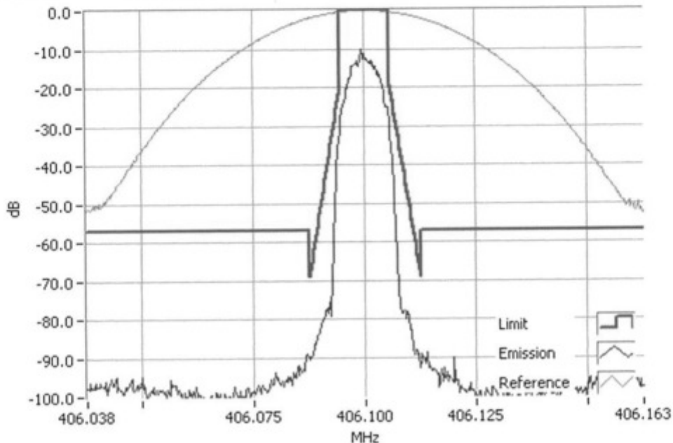
P25 Ph I LSM 406.1000MHz Mask D 5W RBW=100Hz, VBW=1000Hz, Detector Mode=Peak Result=Pass
