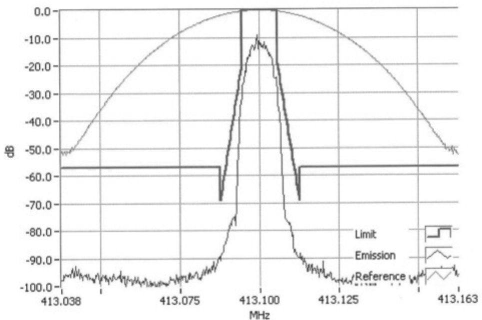
P25 Ph II H-DQPSK 413.1000MHz Mask D 5W RBW=100Hz, VBW=1000Hz, Detector Mode=Peak Result=Pass
