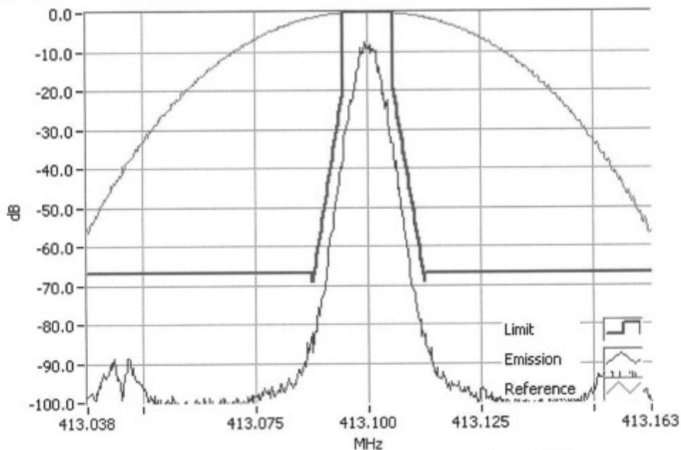
P25 Ph I C4FM 413.1000MHz Mask D 50W RBW=100Hz, VBW=1000Hz, Detector Mode=Peak Result=Pass
