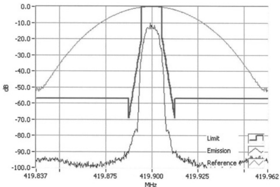
P25 Ph II H-DQPSK 419.9000MHz Mask D 5W RBW=100Hz, VBW=1000Hz, Detector Mode=Peak Result=Pass
