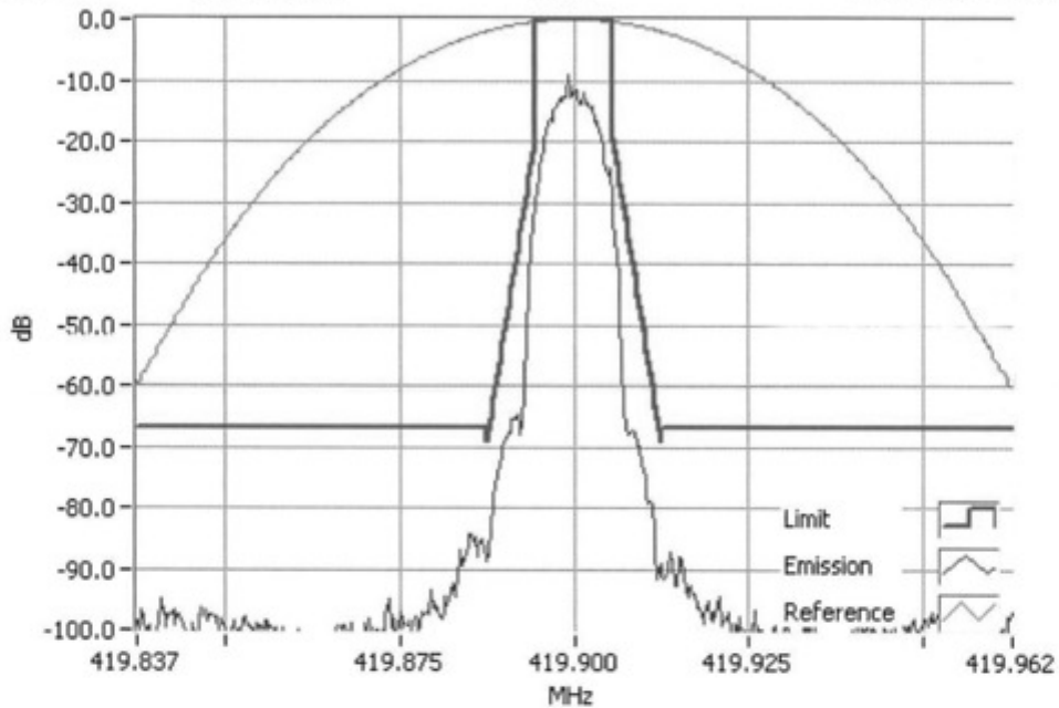
P25 Ph II H-DQPSK 419.9000MHz Mask D 50W RBW=100Hz, VBW=1000Hz, Detector Mode=Peak Result=Pass
