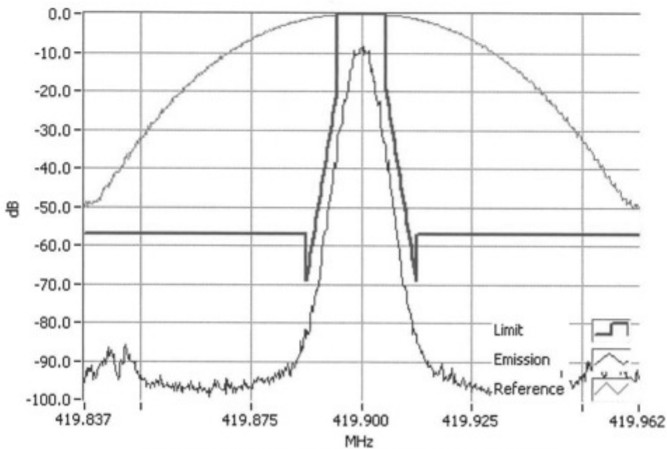
P25 Ph I C4FM 419.9000MHz Mask D 5W RBW=100Hz, VBW=1000Hz, Detector Mode=Peak Result=Pass
