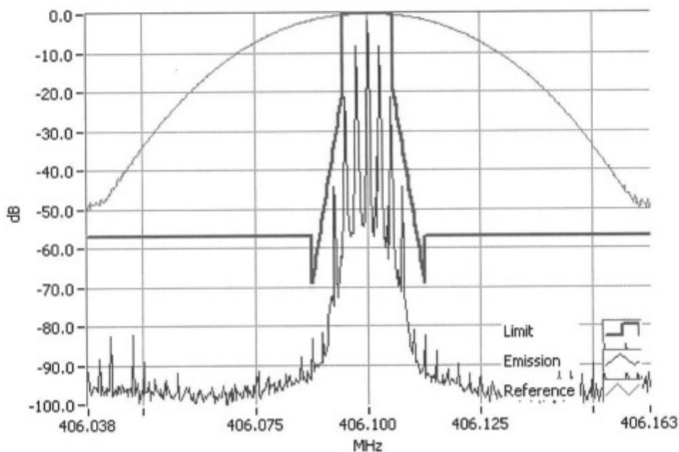
Analogue Modulation 406.1000MHz Mask D 5W RBW=100Hz, VBW=1000Hz, Detector Mode=Peak Result=Pass
