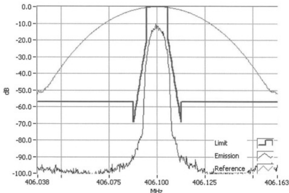
P25 Ph II H-DQPSK 406.1000MHz Mask D 5W RBW=100Hz, VBW=1000Hz, Detector Mode=Peak Result=Pass
