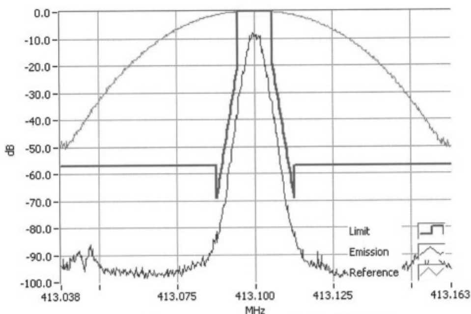
P25 Ph I C4FM 413.1000MHz Mask D 5W RBW=100Hz, VBW=1000Hz, Detector Mode=Peak Result=Pass
