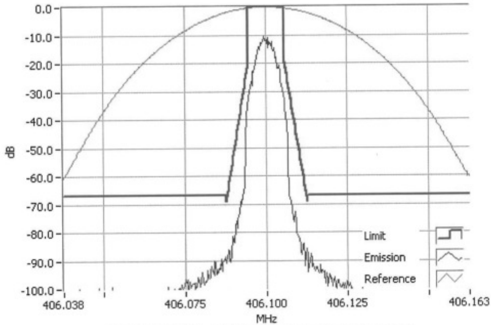
P25 Ph I LSM 406.1000MHz Mask D 50W RBW=100Hz, VBW=1000Hz, Detector Mode=Peak Result=Pass
