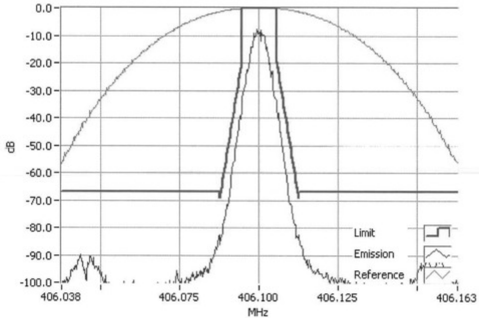
P25 Ph I C4FM 406.1000MHz Mask D 50W RBW=100Hz, VBW=1000Hz, Detector Mode=Peak Result=Pass
