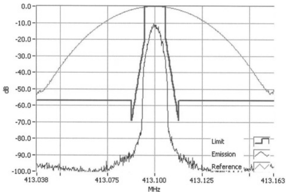
P25 Ph I LSM 413.1000MHz Mask D 5W RBW=100Hz, VBW=1000Hz, Detector Mode=Peak Result=Pass
