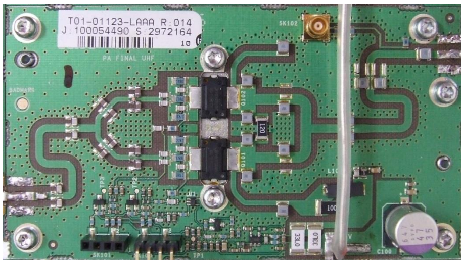
Photograph 1 & 2: Power Amplifier 60W PA PCB – Top & Bottom
