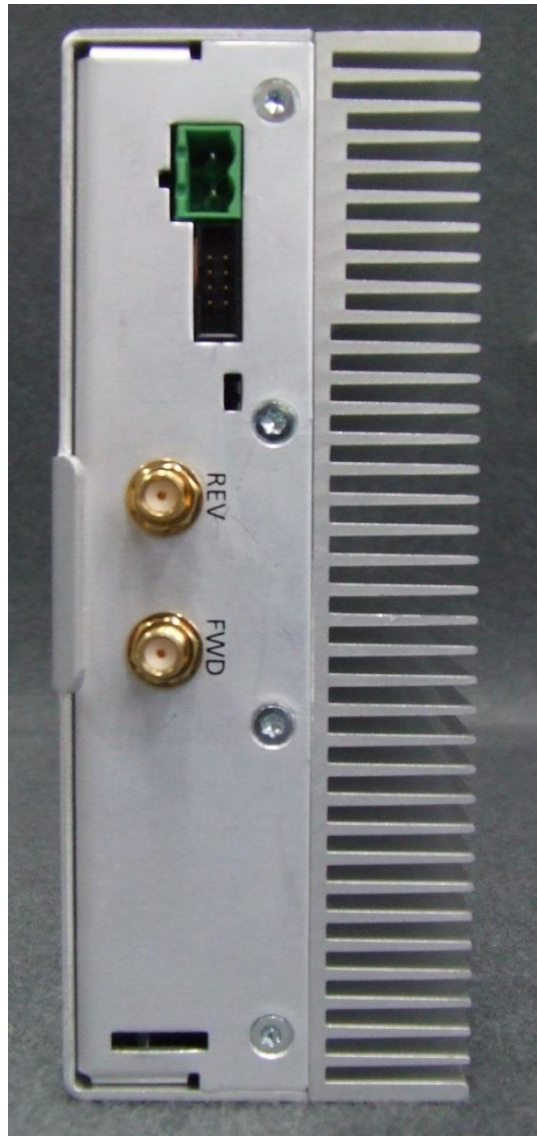
Photograph 09: Power Amplifier – Front panel
