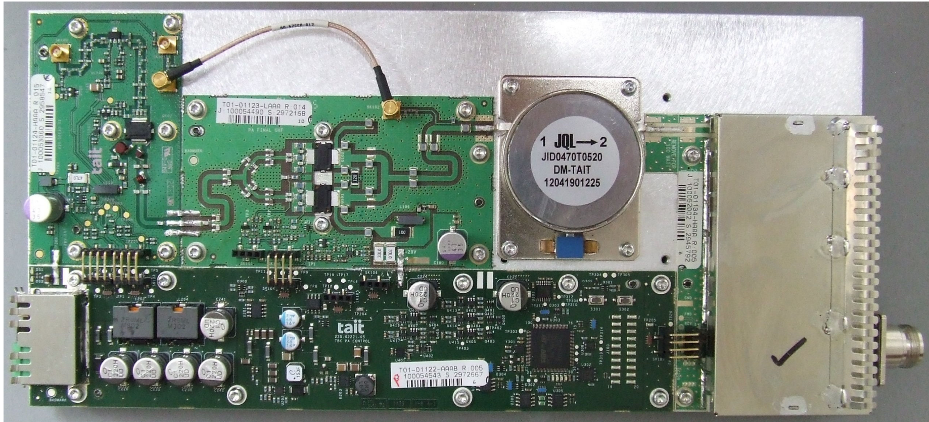
Photograph 15: 50 Watt Power Amplifier – Internal
