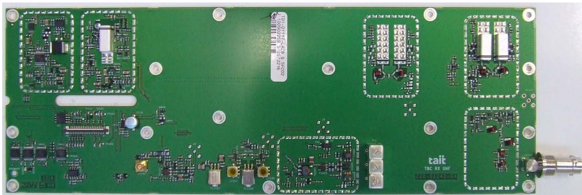
Photograph 12: H2 Reciter Receiver PCB – Top (without shields)
