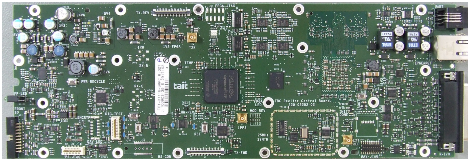
Photograph 07: H1 & H2 Reciter Control PCB – Top (without shields)
