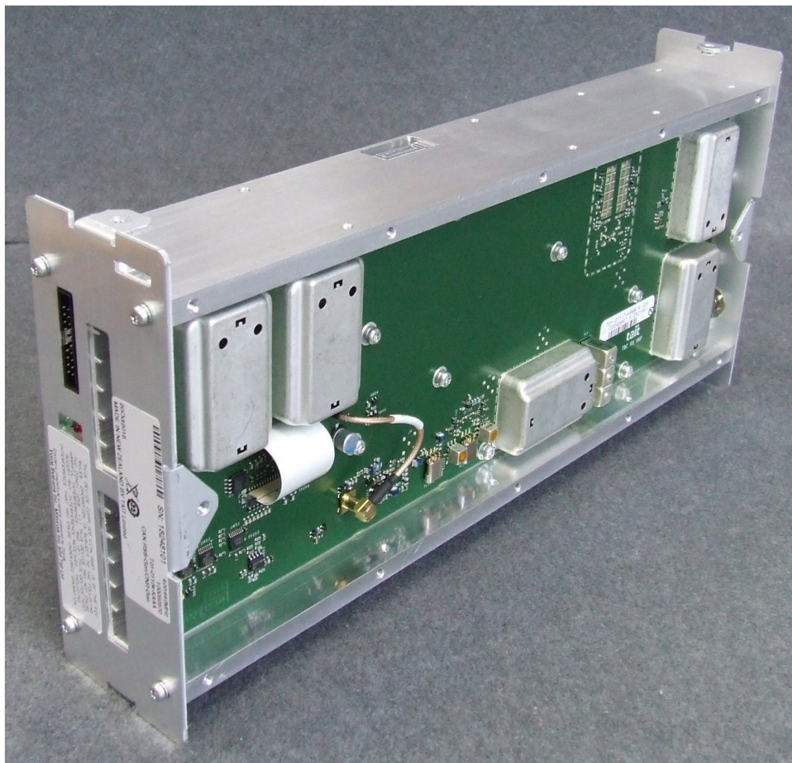
Photograph 01: H1 Reciter module – Internal (Receiver PCB side)
