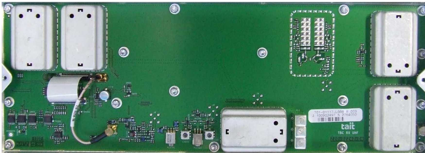
Photograph 11: H2 Reciter Receiver PCB – Top (with shields)
