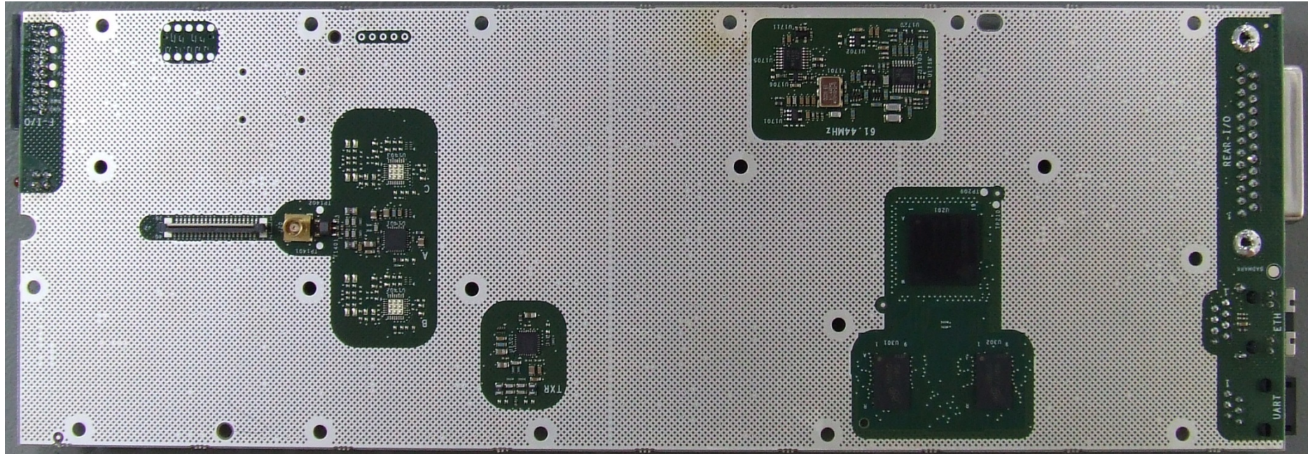
Photograph 08: H1 & H2 Reciter Control PCB – Bottom
