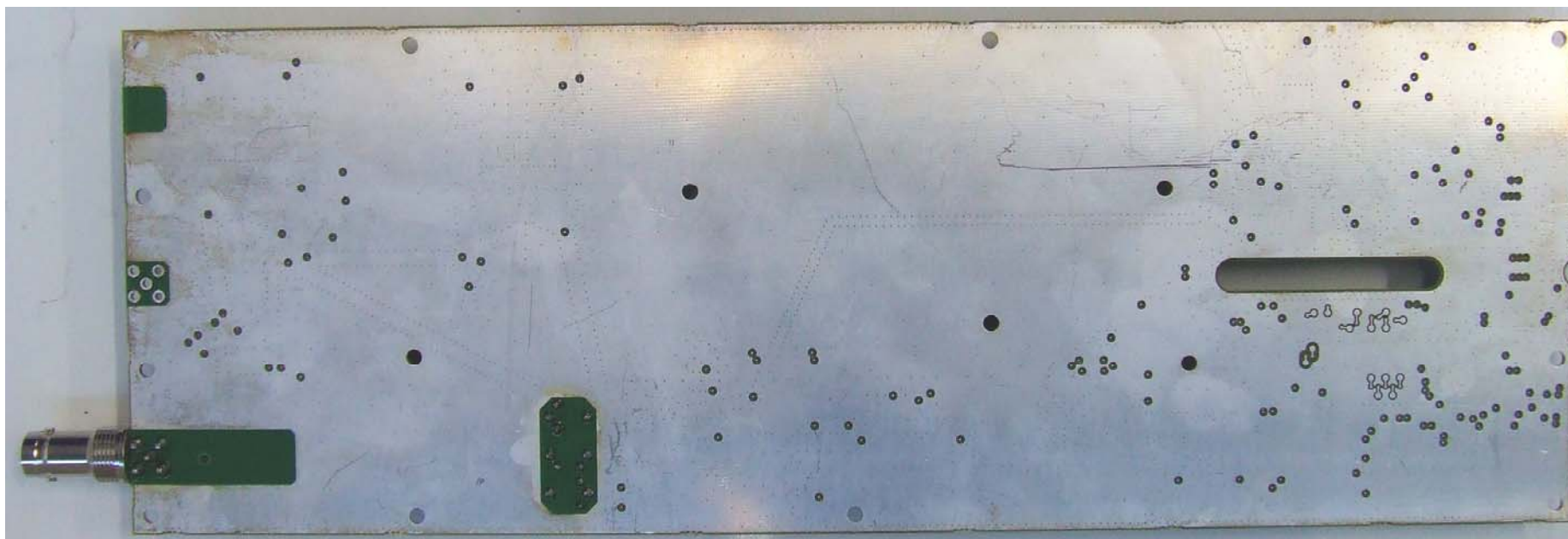
Photograph 13: H2 Reciter Receiver PCB – Bottom
