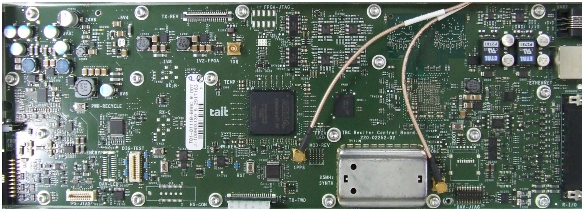
Photograph 06: H1 & H2 Reciter Control PCB – Top (with shields)
