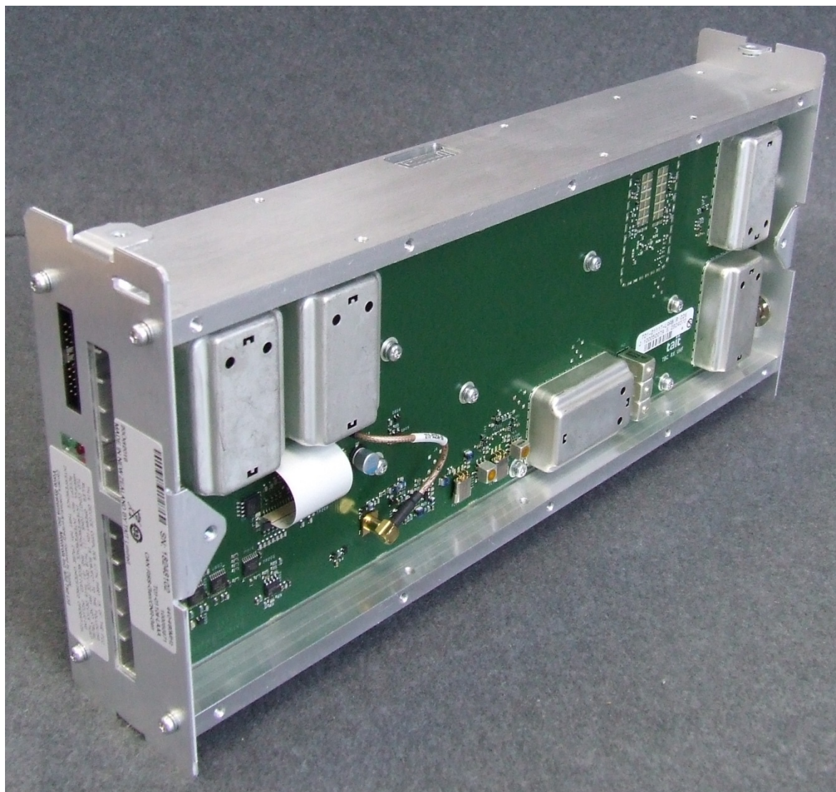
Photograph 09: H2 Reciter module – Internal (Receiver PCB side)
