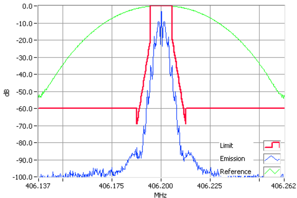
FFSK1200 406.2000MHz Mask D 10W RBW=100Hz, VBW=1000Hz, Detector Mode=Peak Result=Pass
