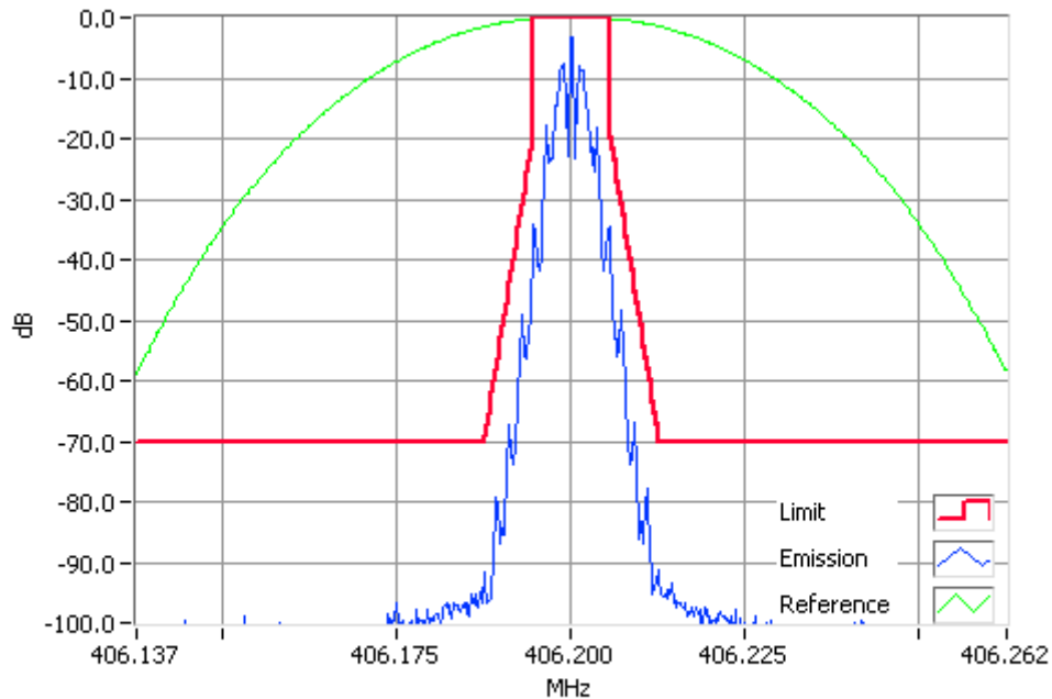
FFSK1200 406.2000MHz Mask D 100W RBW=100Hz, VBW=1000Hz, Detector Mode=Peak Result=Pass
