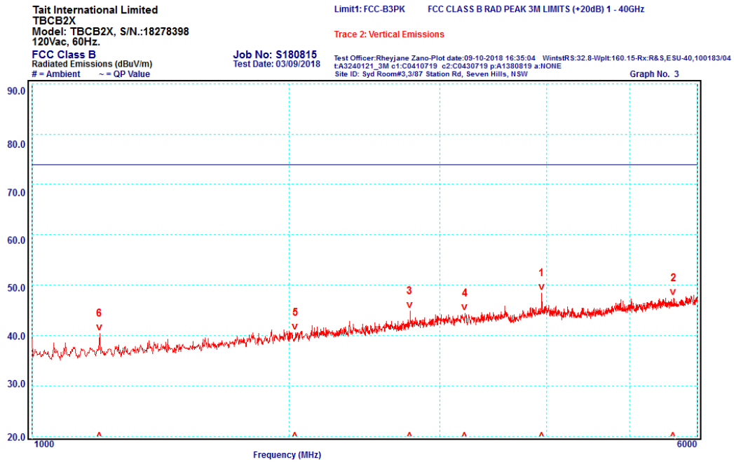
Graph 3: Vertical Polarisation 1000 to 6000MHz
