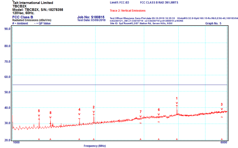
Graph 5: Vertical Polarisation 1000 to 6000MHz
