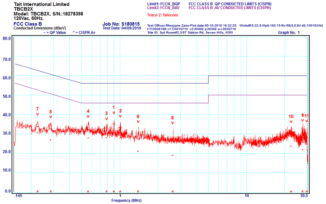
Graph 1 Telecom Line 0.145 to 30.5MHz
