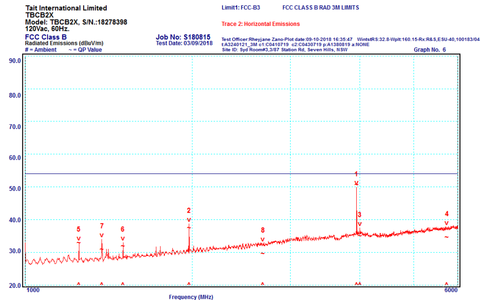
Graph 6: Horizontal Polarisation 1000 to 6000MHz
