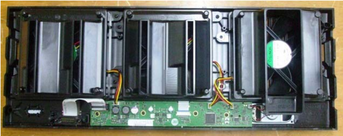
Fan assembly including the fan electronics
