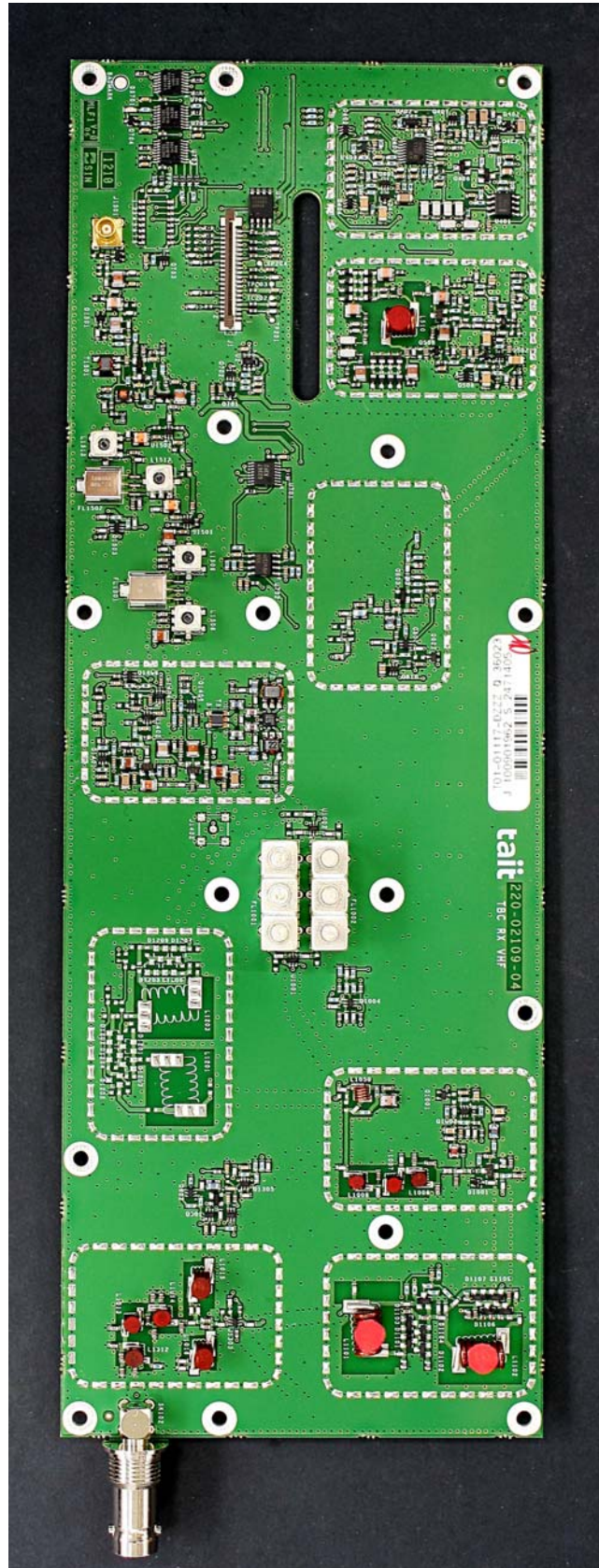
Receiver boards with RF shield removed and with shields attached
