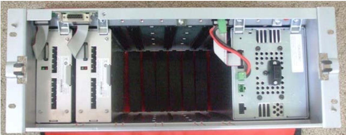
Front of base station with the fans removed
