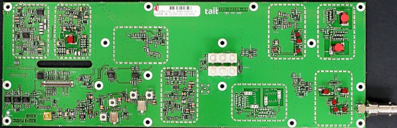
Reciter Internal 'Receiver' Board Top View - No Cans Fitted
