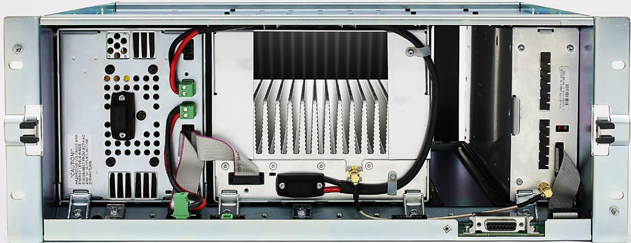
100W Digital Subrack Front View - No Front Panel
