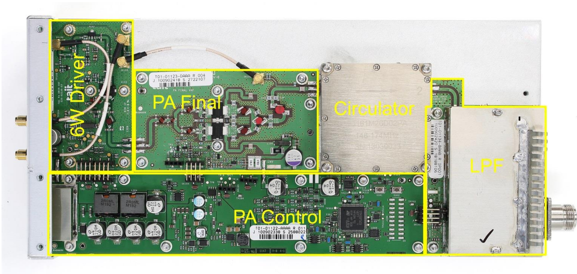
Photograph 01: PA module – Internal view
