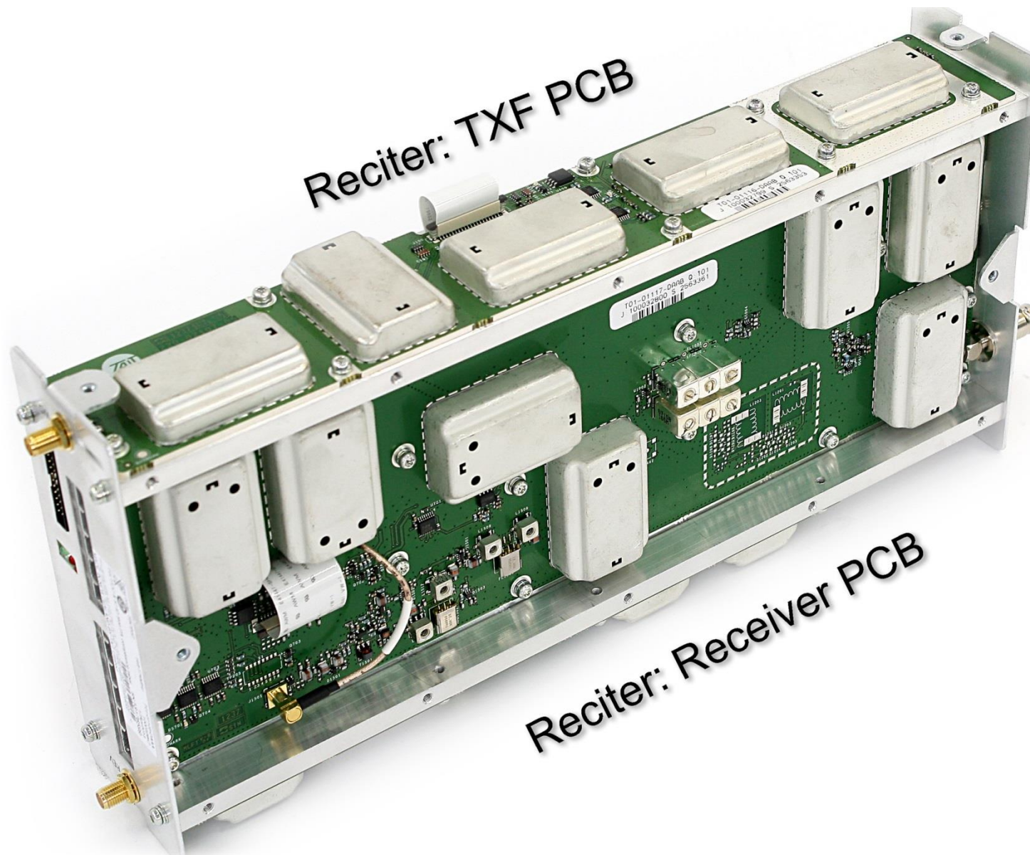
Photograph 10: Reciter module – Internal (Receiver PCB side)
