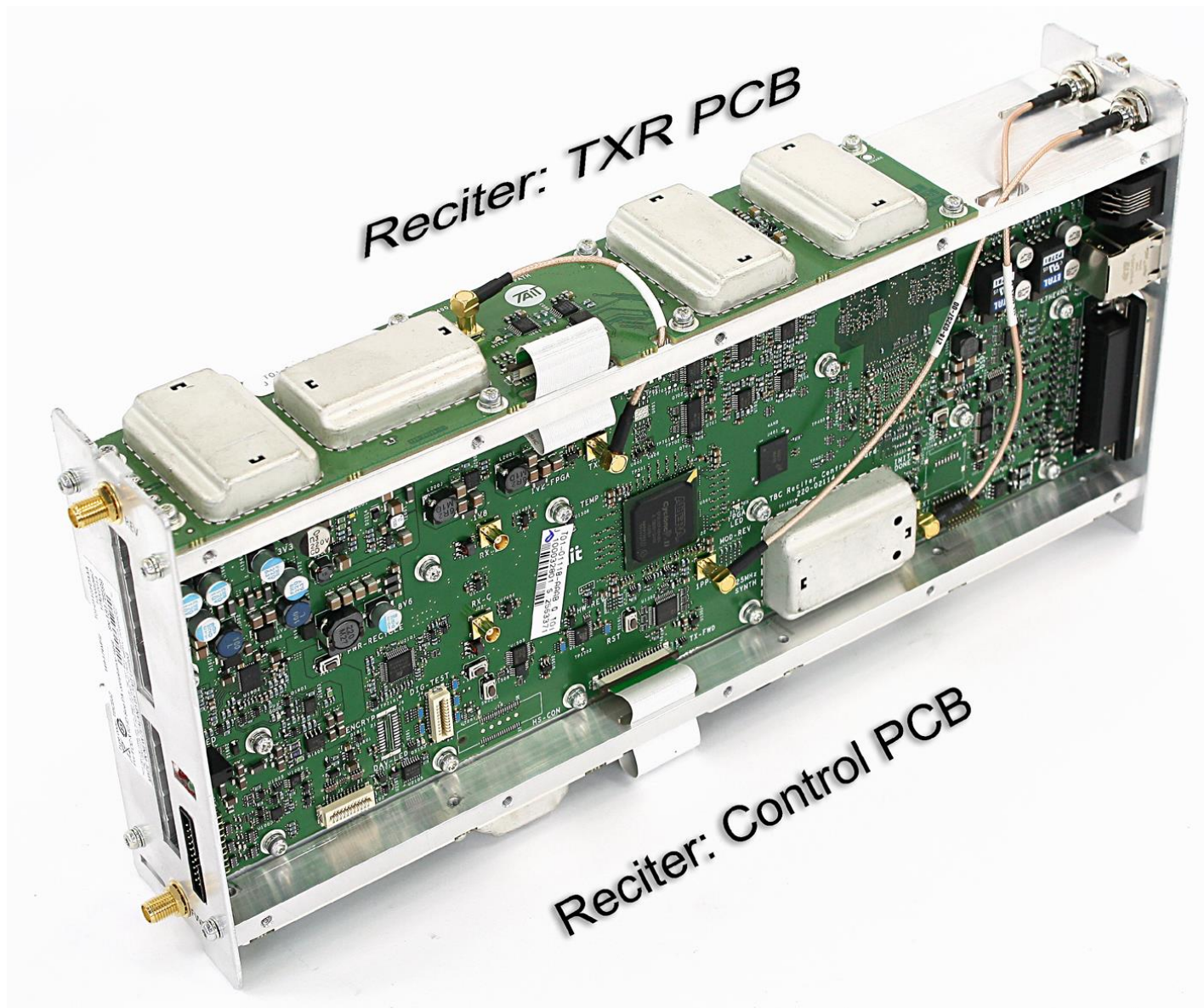
Photograph 11: Reciter module – Internal (Control PCB side)
