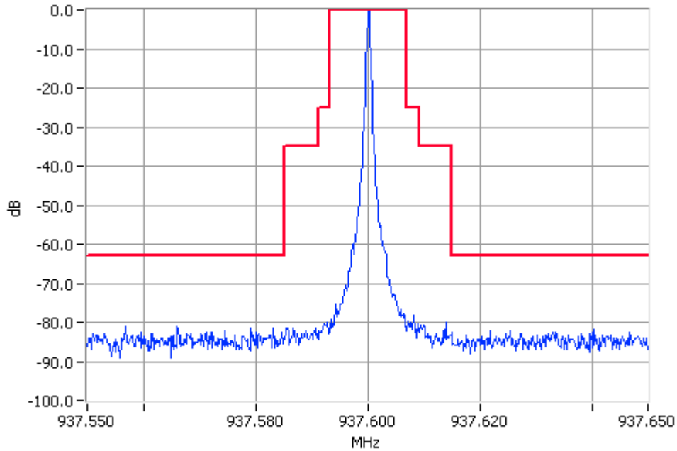
Unmodulated 937.600MHz Mask I 100W Pass RBW=300Hz VBW=3000Hz
