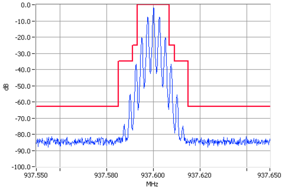
Analogue Modulation 937.600MHz Mask I 100W Pass RBW=300Hz VBW=3000Hz
