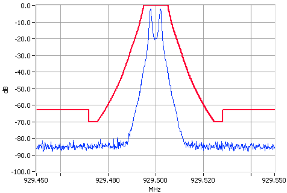
Paging Modulation 929.500MHz Mask G 100W Pass RBW=300Hz VBW=3000Hz
