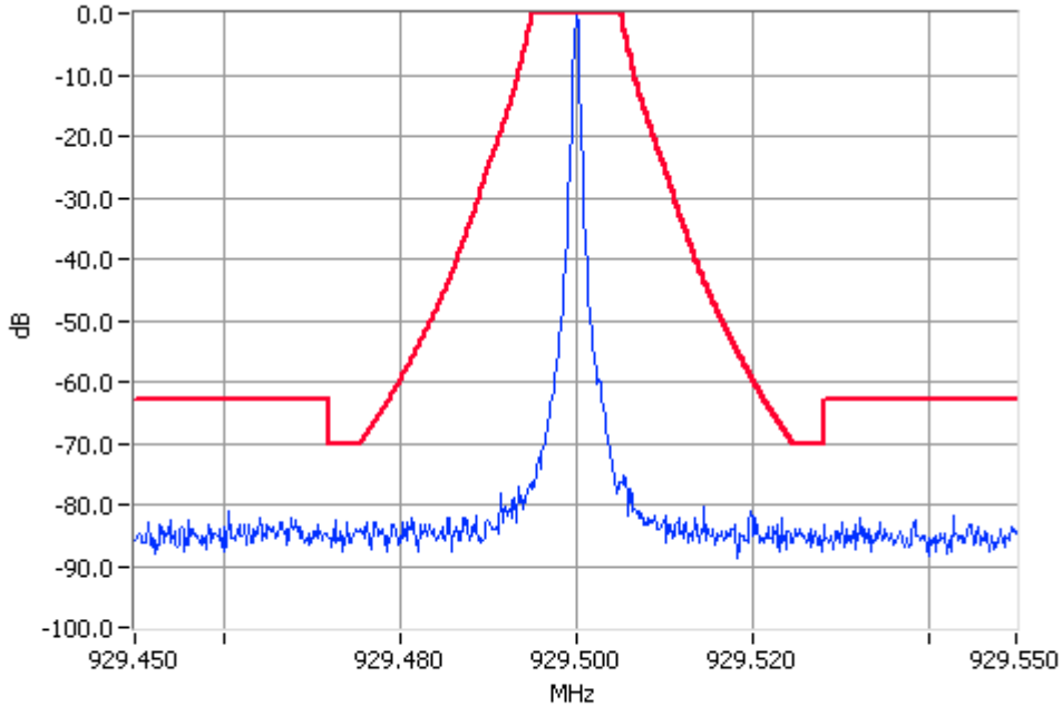
Unmodulated 929.500MHz Mask G 100W Pass RBW=300Hz VBW=3000Hz
