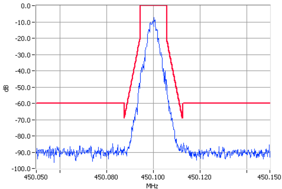
TSM 450.1000MHz Mask D 10W Pass RBW=100Hz VBW=1000Hz
