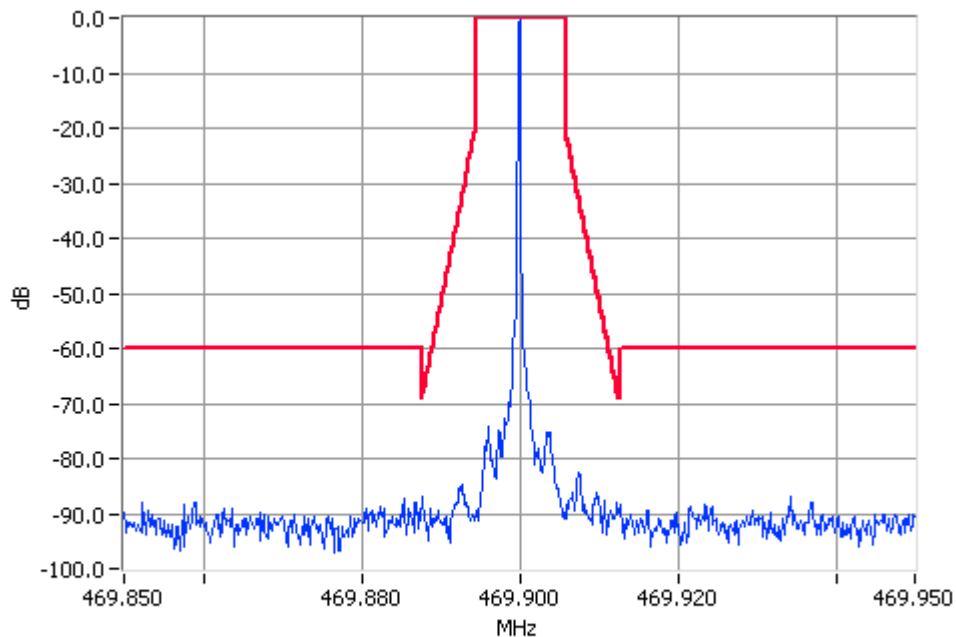
Unmodulated 469.9000MHz Mask D 10W Pass RBW=100Hz VBW=1000Hz
