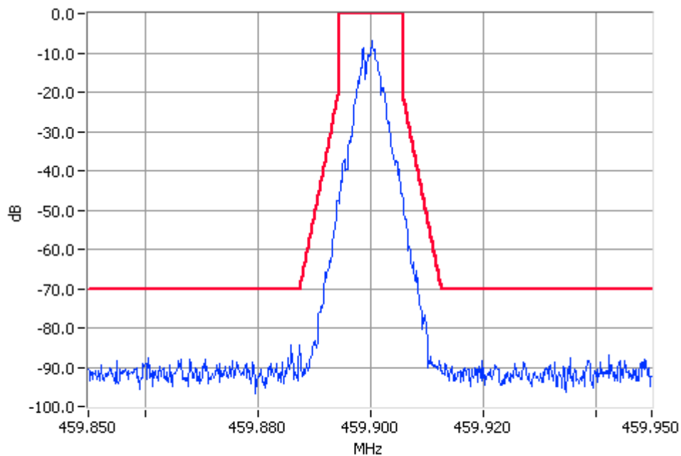
TSM 459.9000MHz Mask D 100W Pass RBW=100Hz VBW=1000Hz
