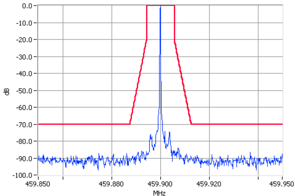
Unmodulated 459.9000MHz Mask D 100W Pass RBW=100Hz VBW=1000Hz
