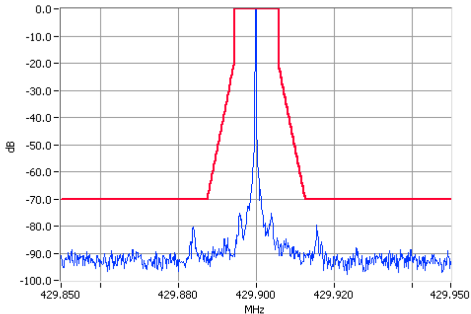
Unmodulated 429.9000MHz Mask D 100W Pass RBW=100Hz VBW=1000Hz
