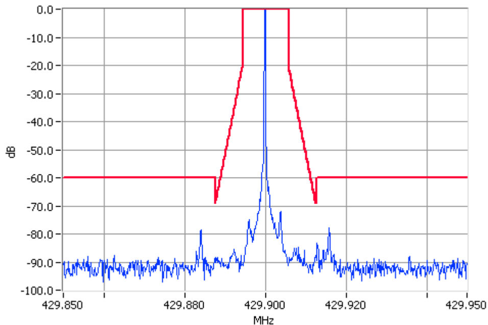
Unmodulated 429.9000MHz Mask D 10W Pass RBW=100Hz VBW=1000Hz
