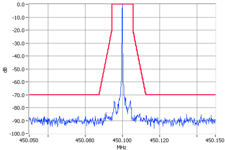
Unmodulated 450.1000MHz Mask D 100W Pass RBW=100Hz VBW=1000Hz
