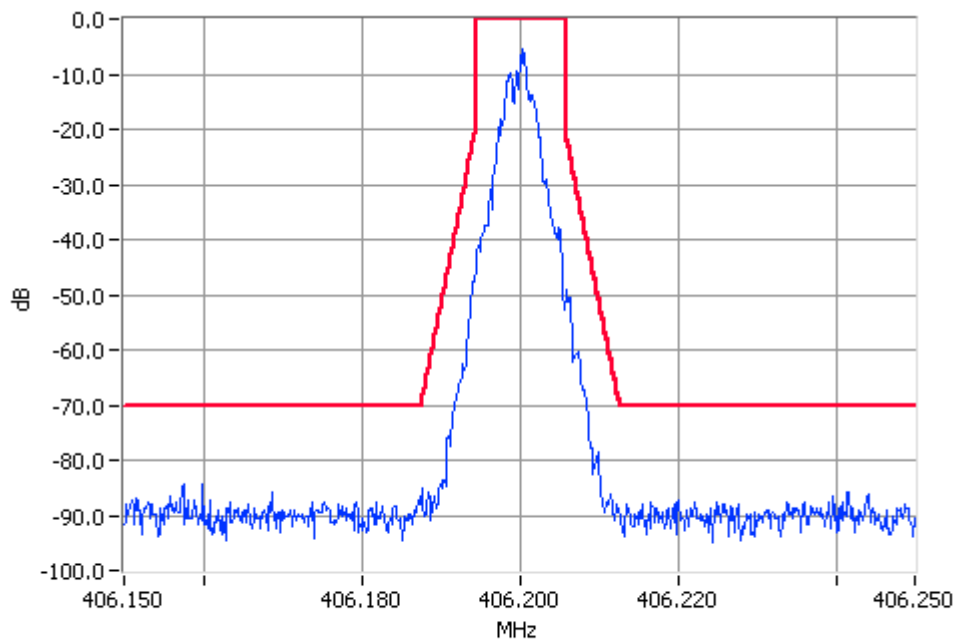
TSM 406.2000MHz Mask D 100W Pass RBW=100Hz VBW=1000Hz
