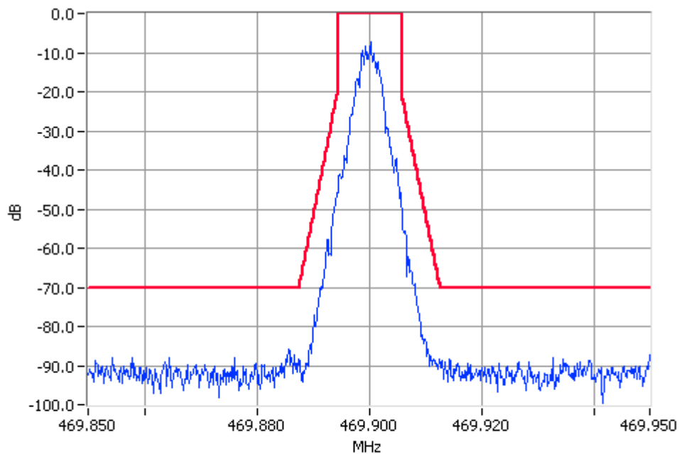
TSM 469.9000MHz Mask D 100W Pass RBW=100Hz VBW=1000Hz
