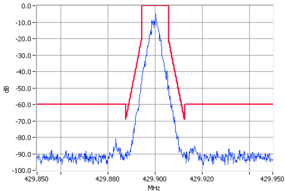
TSM 429.9000MHz Mask D 10W Pass RBW=100Hz VBW=1000Hz
