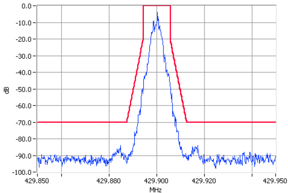
TSM 429.9000MHz Mask D 100W Pass RBW=100Hz VBW=1000Hz
