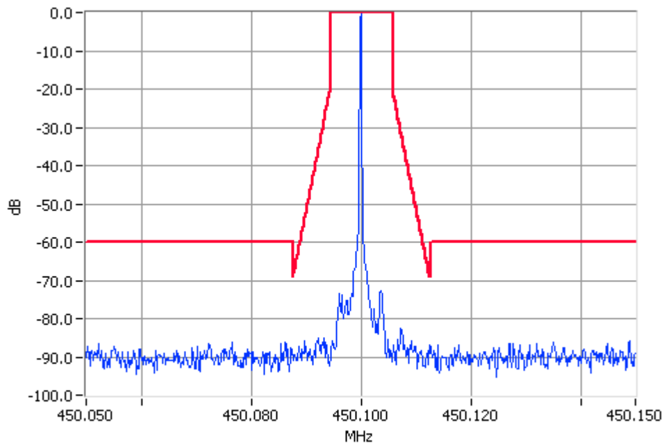
Unmodulated 450.1000MHz Mask D 10W Pass RBW=100Hz VBW=1000Hz
