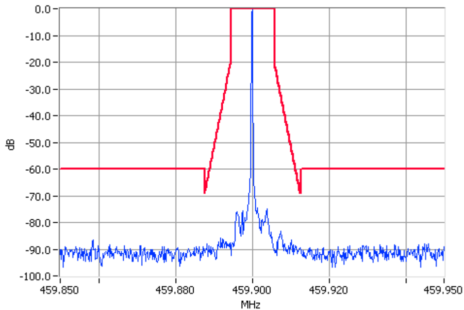
Unmodulated 459.9000MHz Mask D 10W Pass RBW=100Hz VBW=1000Hz
