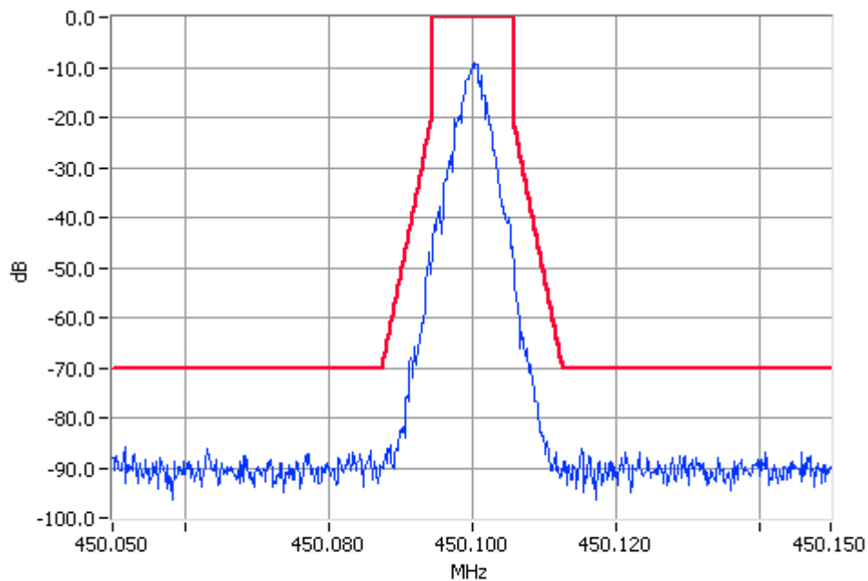
TSM 450.1000MHz Mask D 100W Pass RBW=100Hz VBW=1000Hz
