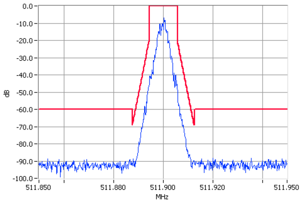
TSM 511.9000MHz Mask D 10W Pass RBW=100Hz VBW=1000Hz
