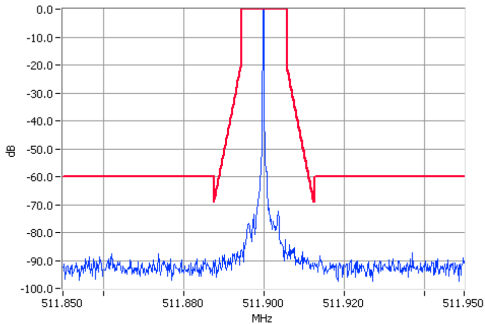
Unmodulated 511.9000MHz Mask D 10W Pass RBW=100Hz VBW=1000Hz
