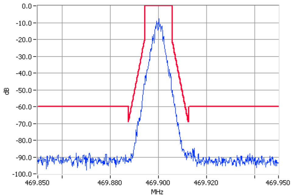
TSM 469.9000MHz Mask D 10W Pass RBW=100Hz VBW=1000Hz
