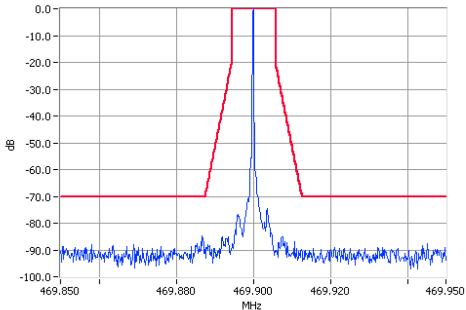
Unmodulated 469.9000MHz Mask D 100W Pass RBW=100Hz VBW=1000Hz
