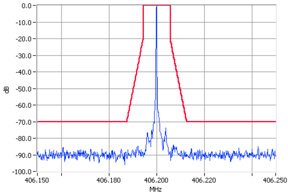
Unmodulated 406.2000MHz Mask D 100W Pass RBW=100Hz VBW=1000Hz
