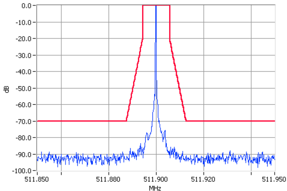
Unmodulated 511.9000MHz Mask D 100W Pass RBW=100Hz VBW=1000Hz
