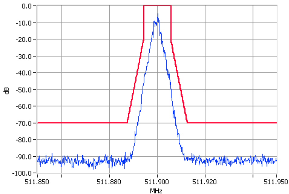
TSM 511.9000MHz Mask D 100W Pass RBW=100Hz VBW=1000Hz
