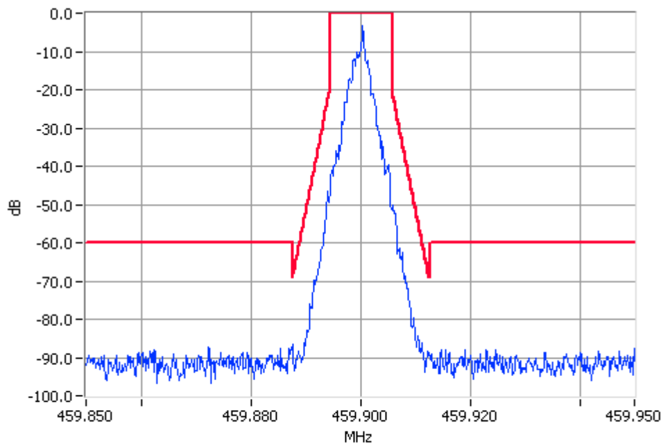
TSM 459.9000MHz Mask D 10W Pass RBW=100Hz VBW=1000Hz
