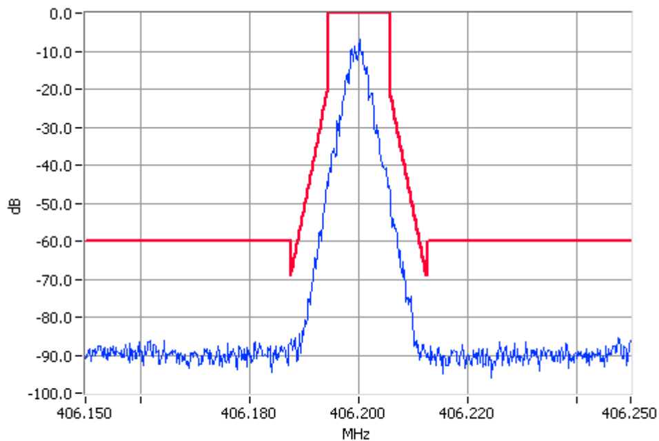
TSM 406.2000MHz Mask D 10W Pass RBW=100Hz VBW=1000Hz
