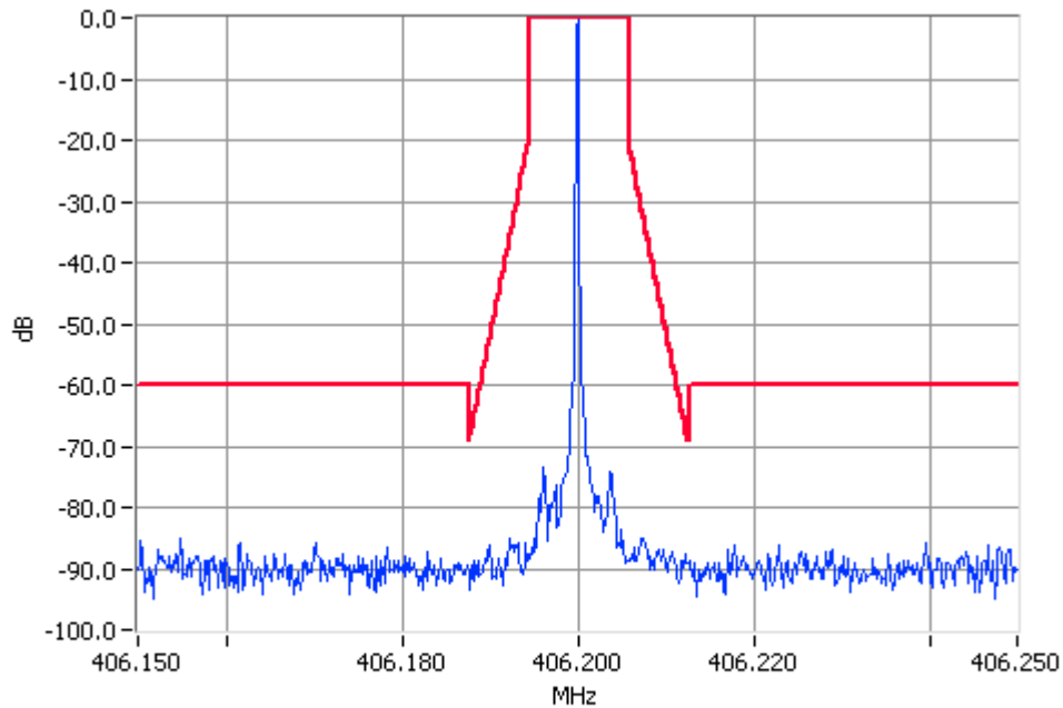
Unmodulated 406.2000MHz Mask D 10W Pass RBW=100Hz VBW=1000Hz
