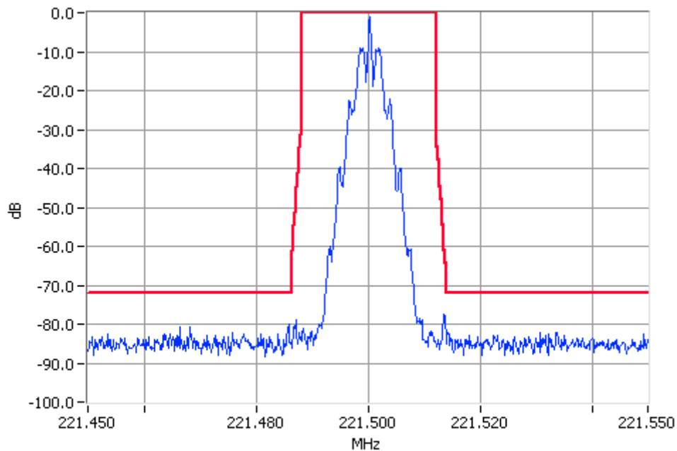
Digital Modulation 221.500MHz Mask Fx5 50W Pass RBW=300Hz VBW=3000Hz
