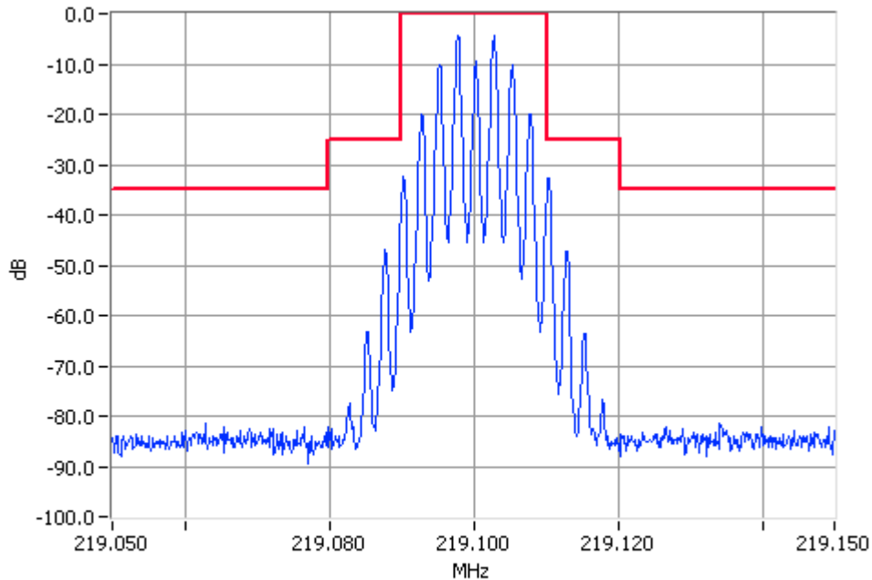
Analogue Modulation 219.100MHz Mask B 50W Pass RBW=300Hz VBW=3000Hz
