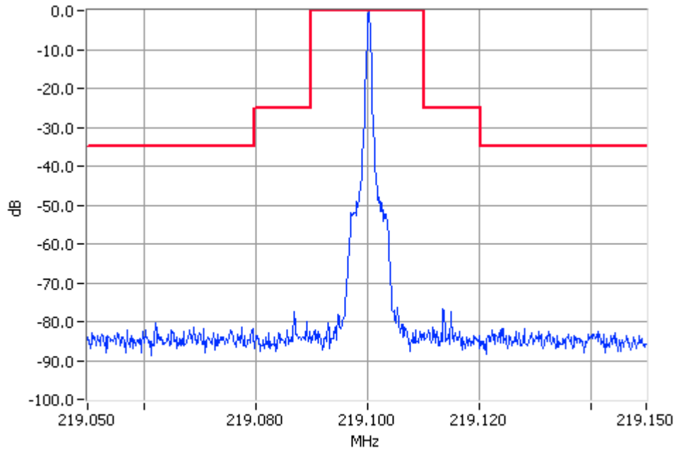
Unmodulated 219.100MHz Mask B 50W Pass RBW=300Hz VBW=3000Hz
