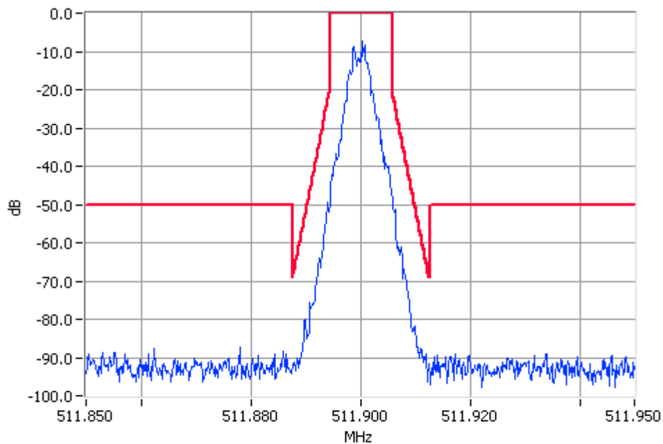
TSM 511.9000MHz Mask D 1W Pass RBW=100Hz VBW=1000Hz
