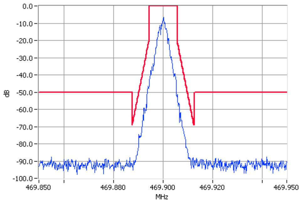
TSM 469.9000MHz Mask D 1W Pass RBW=100Hz VBW=1000Hz
