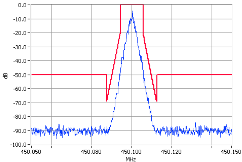
TSM 450.1000MHz Mask D 1W Pass RBW=100Hz VBW=1000Hz
