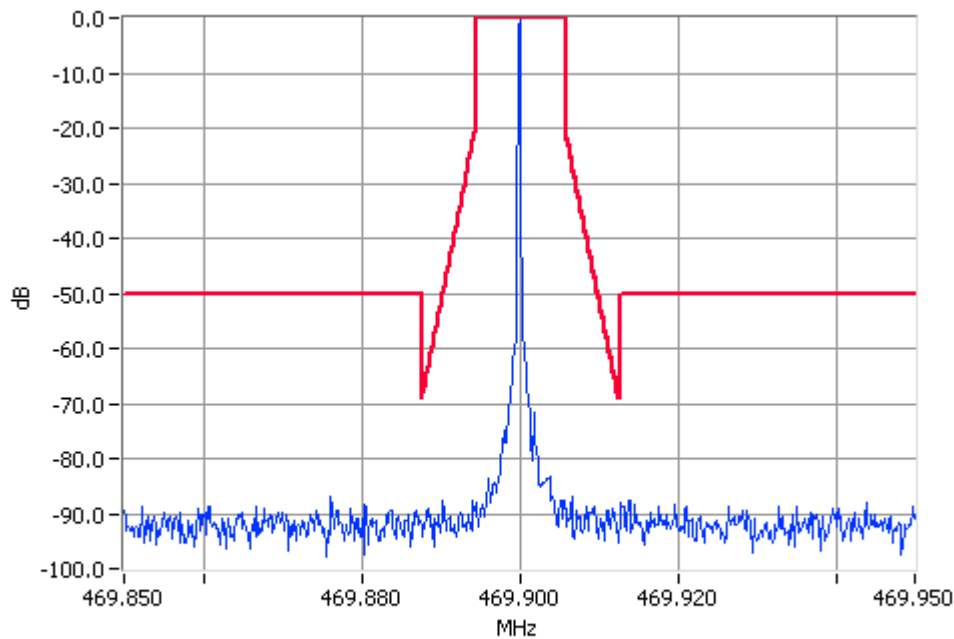
Unmodulated 469.9000MHz Mask D 1W Pass RBW=100Hz VBW=1000Hz
