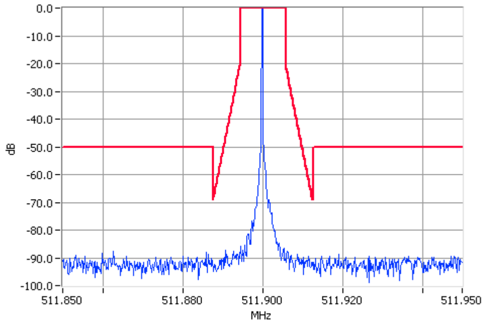
Unmodulated 511.9000MHz Mask D 1W Pass RBW=100Hz VBW=1000Hz
