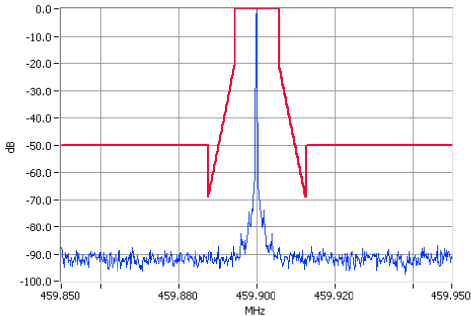
Unmodulated 459.9000MHz Mask D 1W Pass RBW=100Hz VBW=1000Hz
