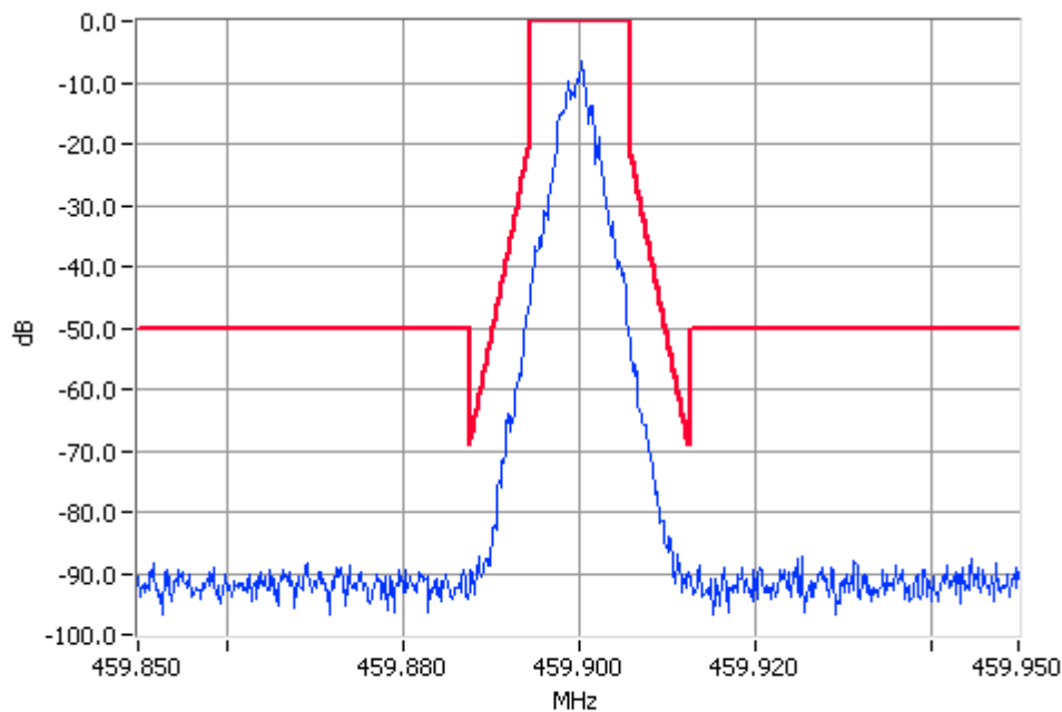
TSM 459.9000MHz Mask D 1W Pass RBW=100Hz VBW=1000Hz
