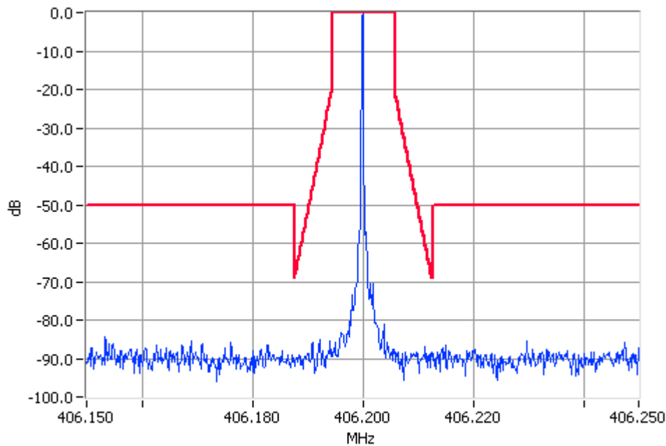
Unmodulated 406.2000MHz Mask D 1W Pass RBW=100Hz VBW=1000Hz
