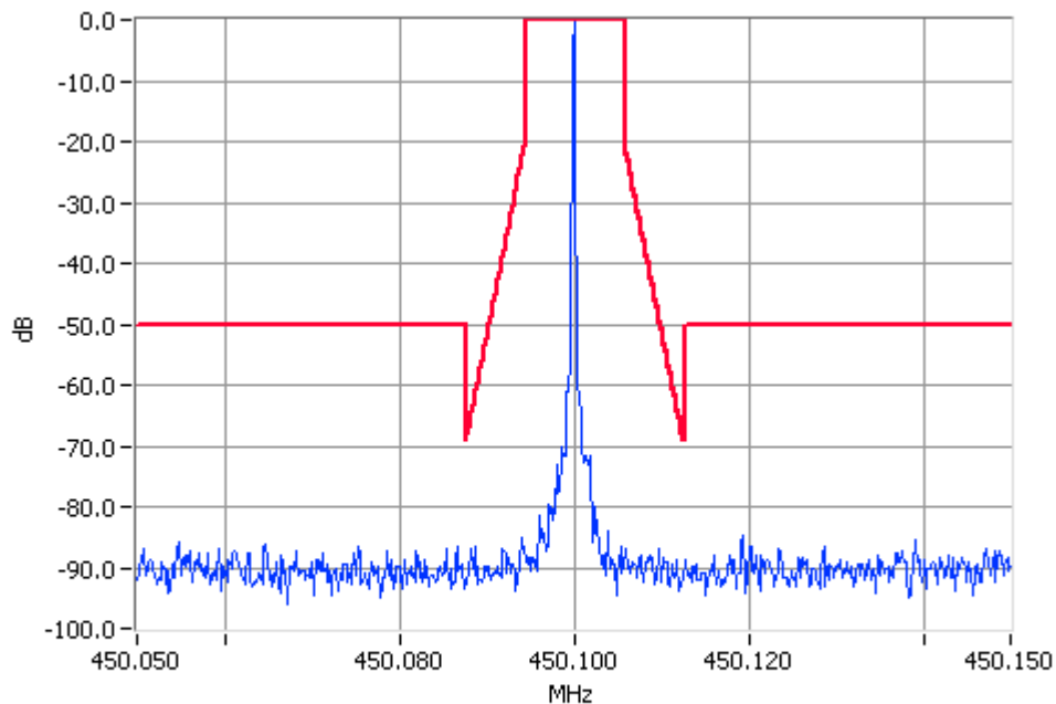
Unmodulated 450.1000MHz Mask D 1W Pass RBW=100Hz VBW=1000Hz
