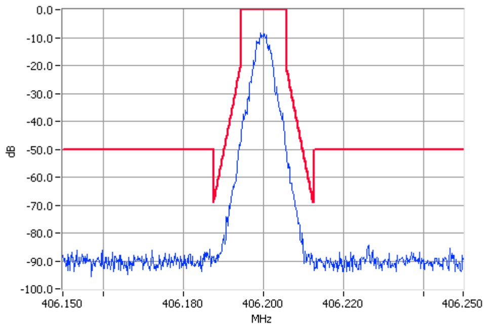
TSM 406.2000MHz Mask D 1W Pass RBW=100Hz VBW=1000Hz
