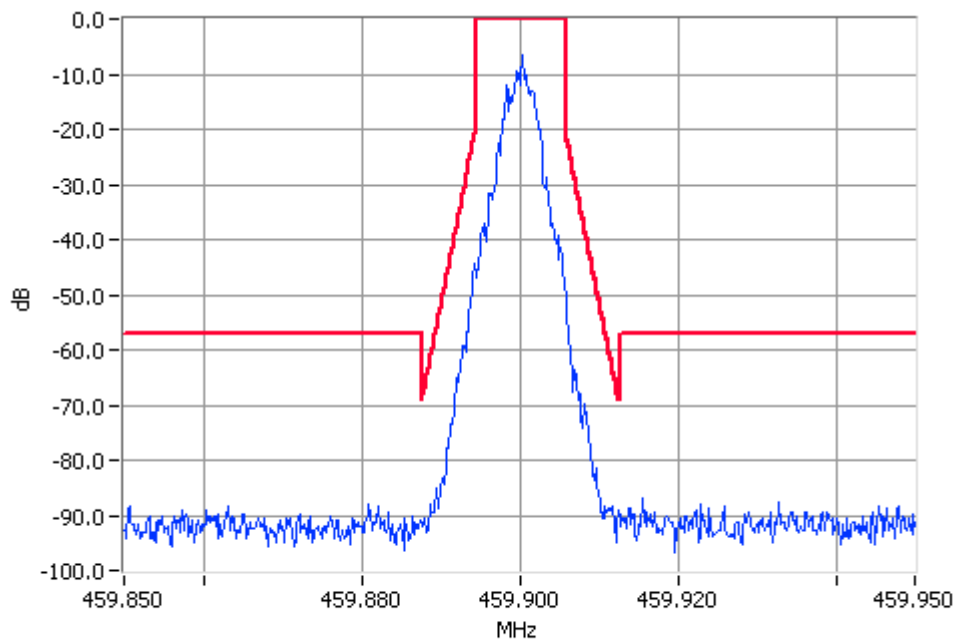
TSM 459.9000MHz Mask D 5W Pass RBW=100Hz VBW=1000Hz
