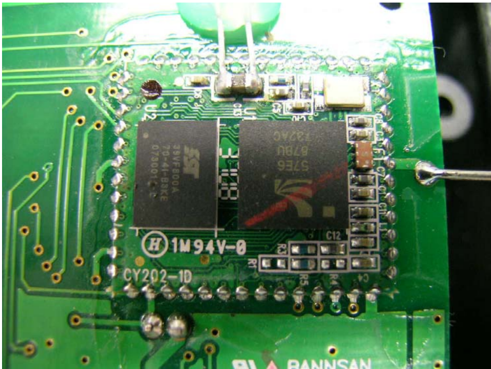
Bluetooth Cellular Gateway RF PCB comp side
