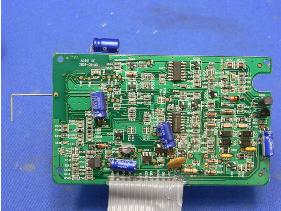
Bluetooth Cellular Gateway Main PCB solder side
