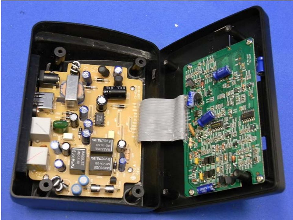
Bluetooth Cellular Gateway assembly
