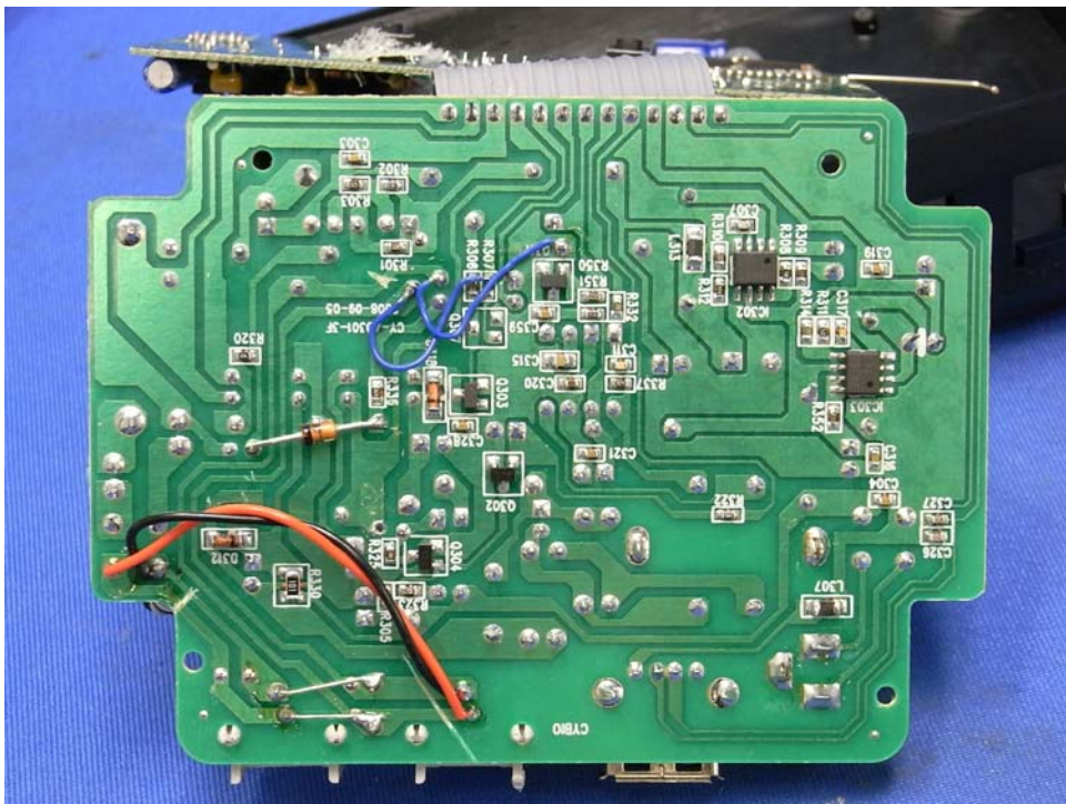
Bluetooth Cellular Gateway another Main PCB comp side
