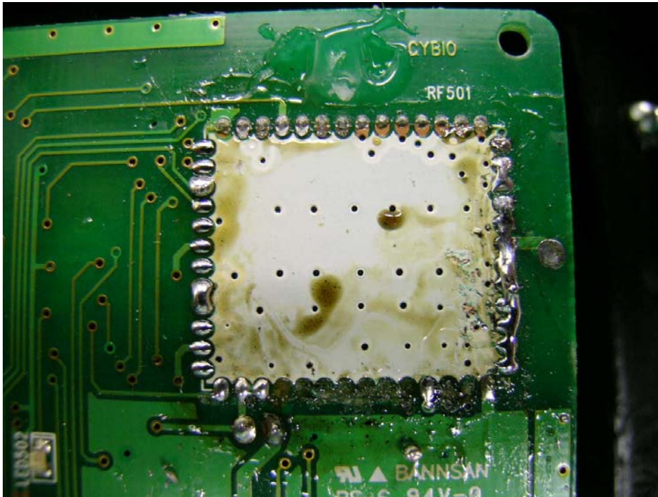
Bluetooth Cellular Gateway RF PCB solder side
