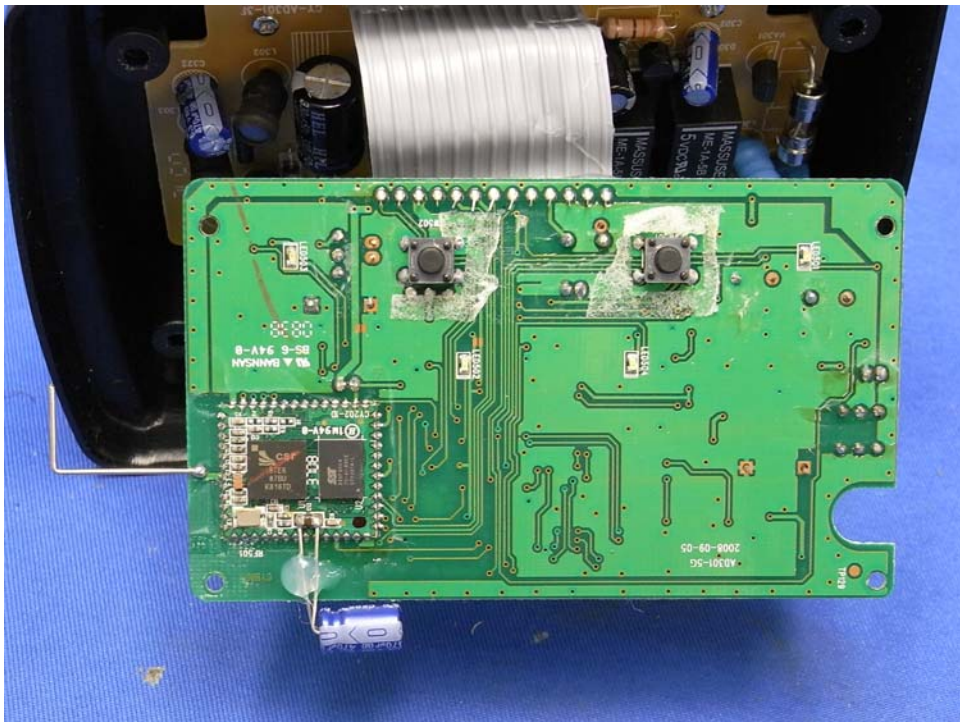
Bluetooth Cellular Gateway Main PCB comp side
