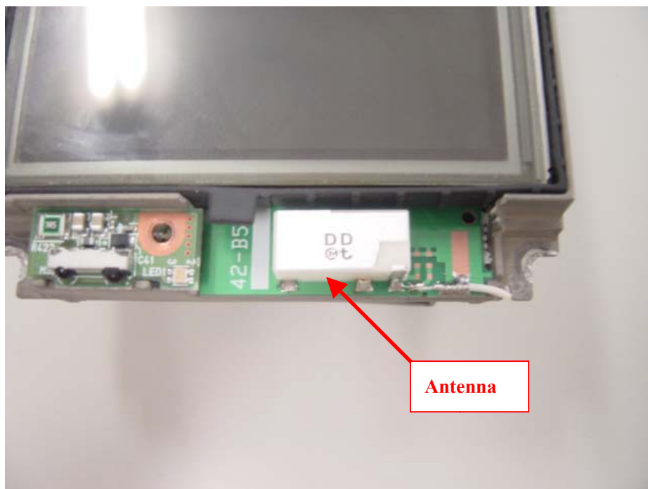
WLAN Antenna
