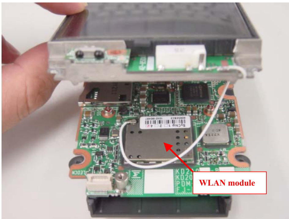
Installation description of WLAN module
