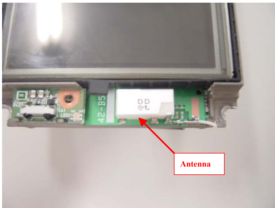
WLAN Antenna
