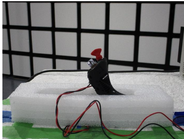
Z-ORIENTATION (worst-case)
