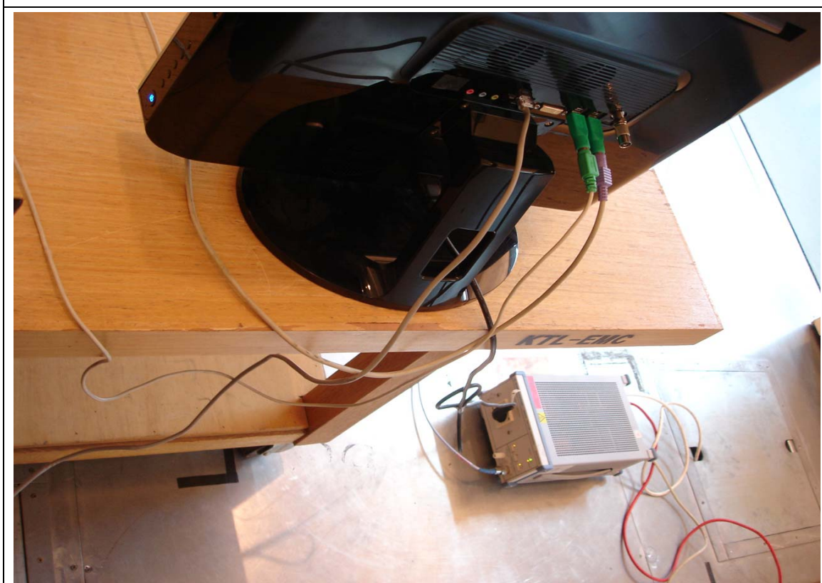
<Conducted emission Test >
