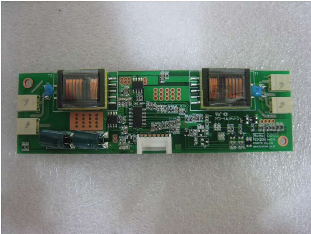
Inverter board
