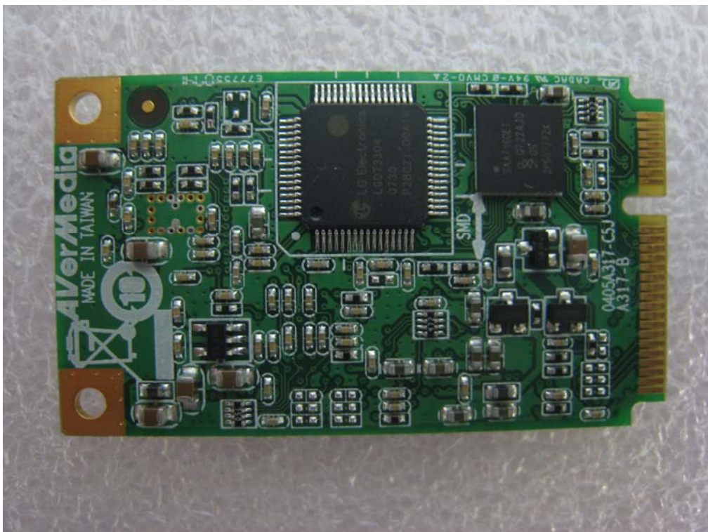
TV card
