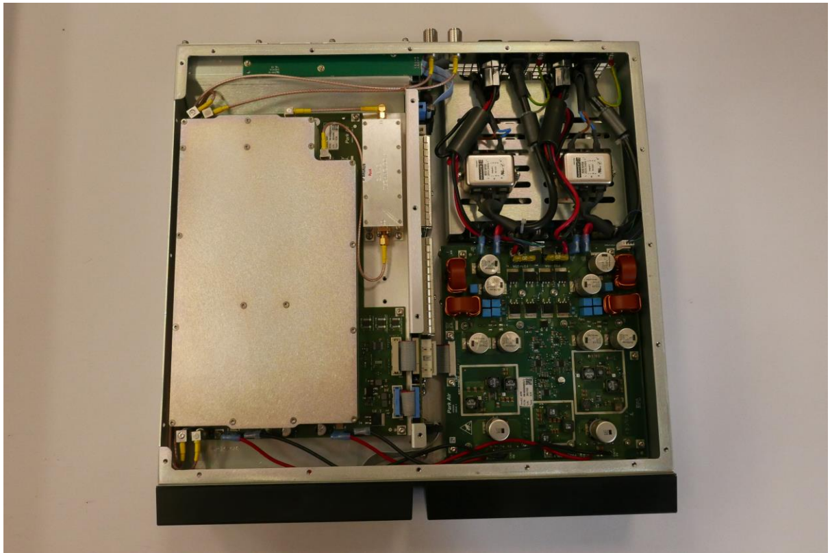
Internal photo of the T6-AV100
