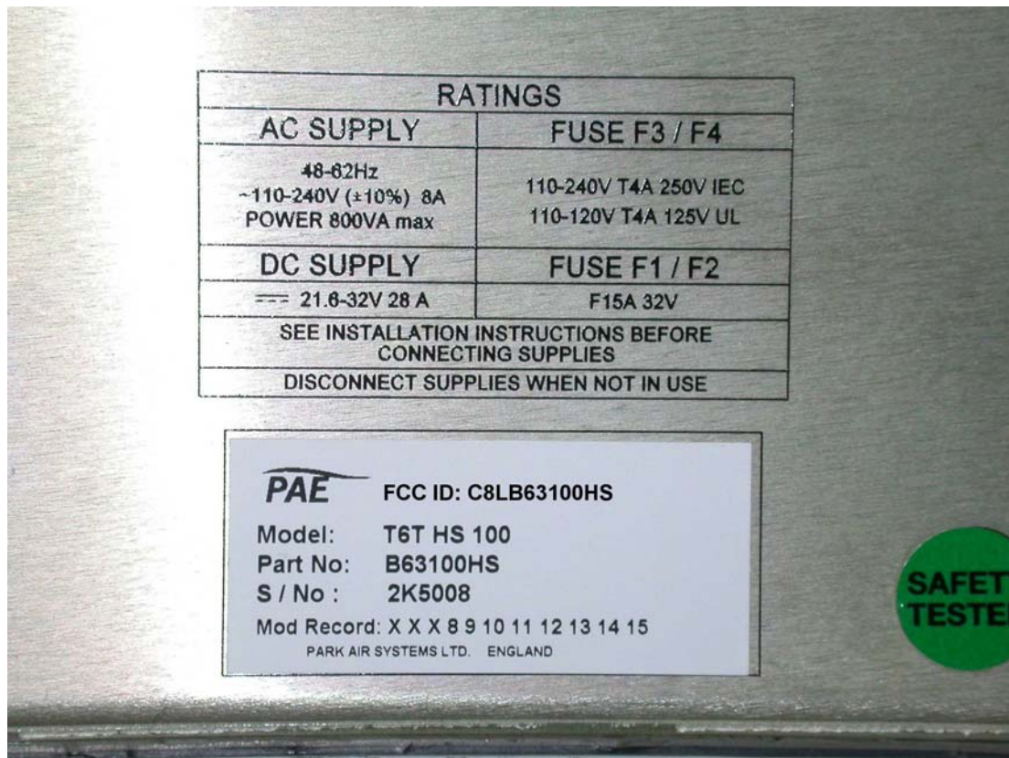
Park Air Systems T6T HS 100 Example label and label position
