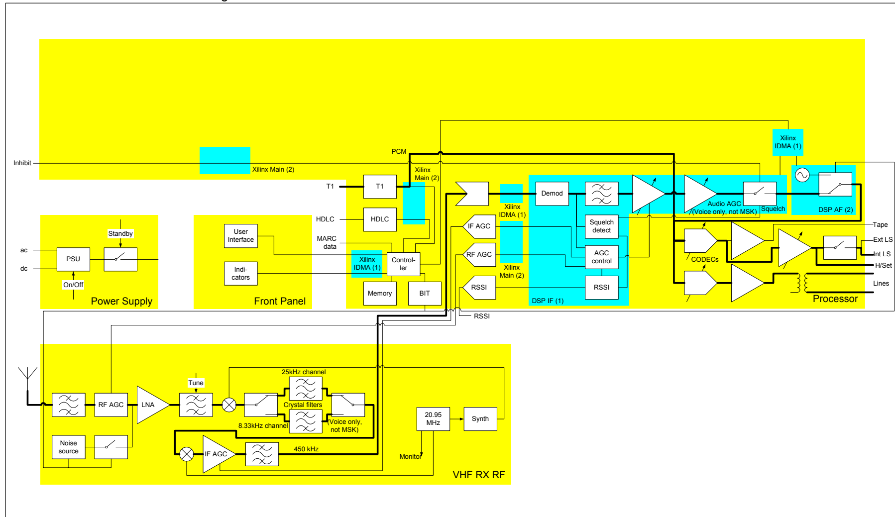
T6R - AM Voice / AM MSK Block Diagram
