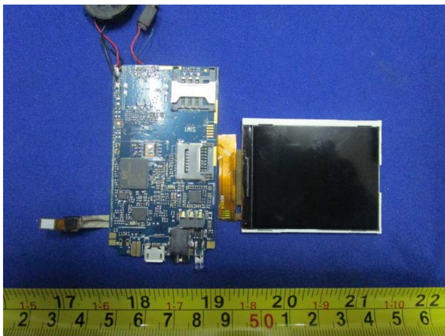
EUT –Main Board & Screen Top View
