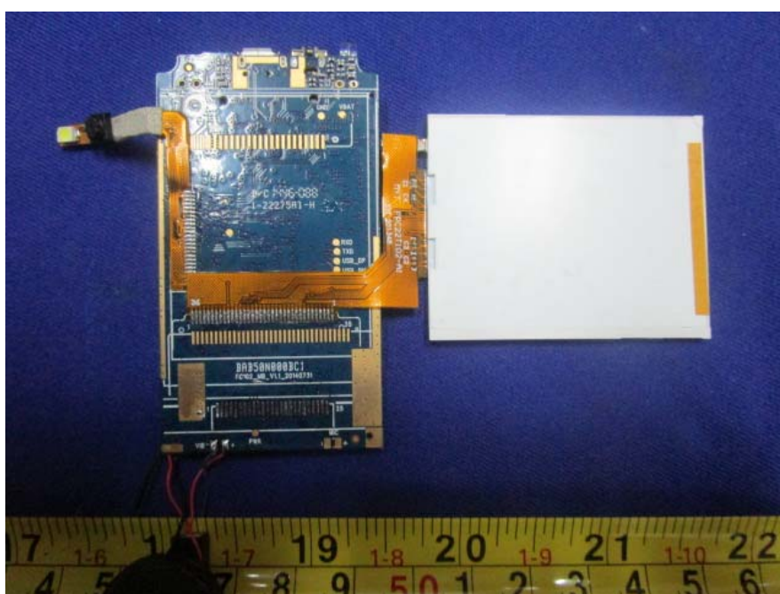
EUT –Main Board & Screen Bottom View
