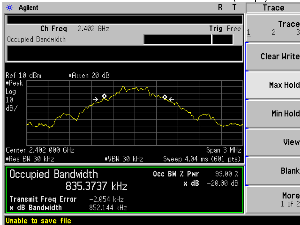
TEST PLOT OF BANDWIDTH FOR LOW CHANNEL(1Mbps)
