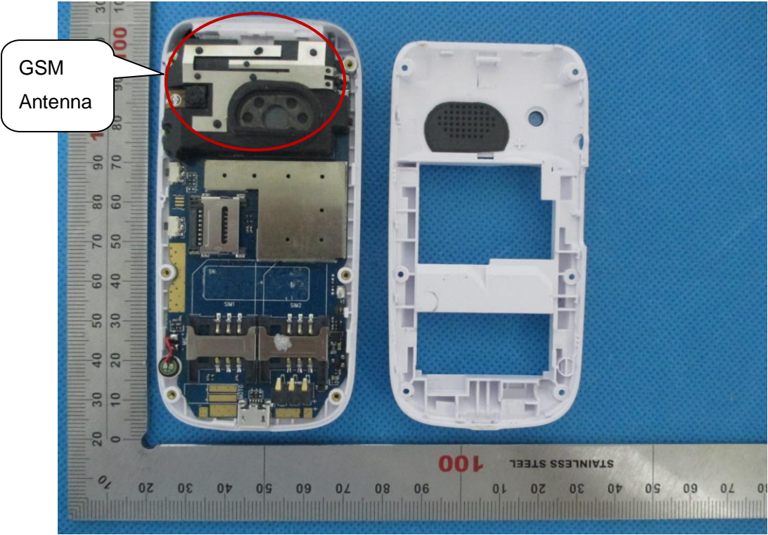
BACK-OPEN VIEW OF EUT-2
