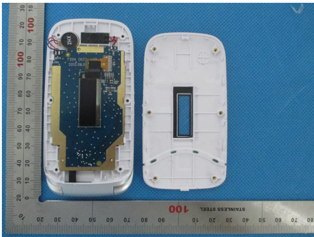
FRONT-OPEN VIEW OF EUT-1
