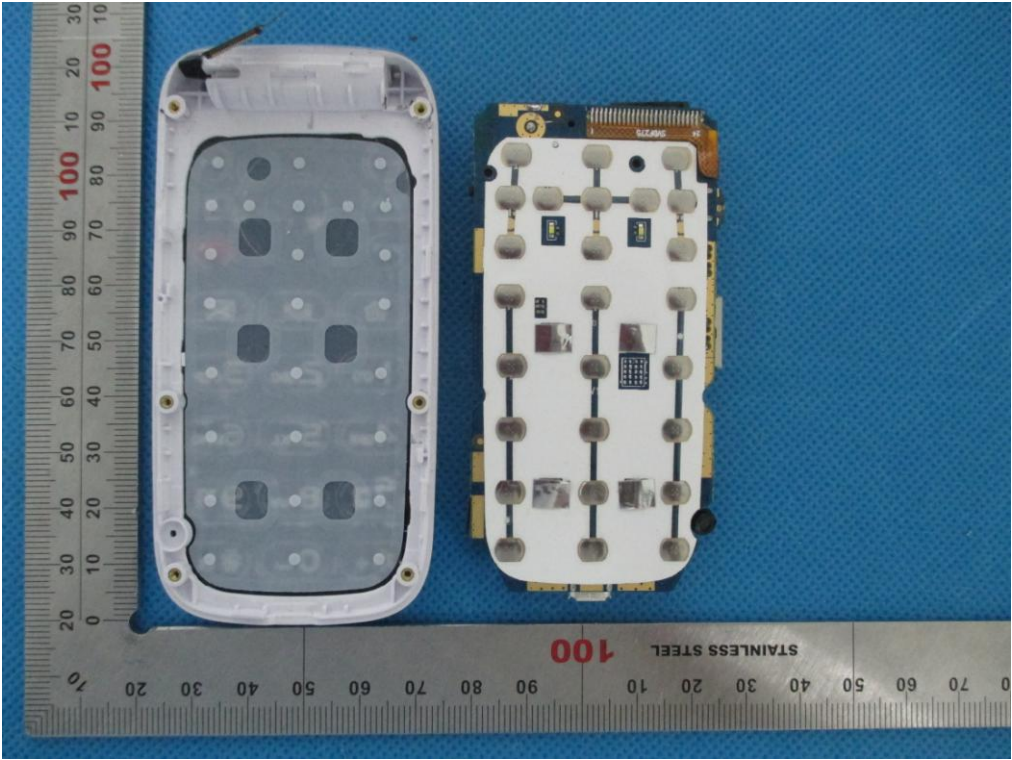
BACK-OPEN VIEW OF EUT-3
