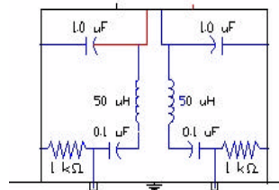
Figure 5. LISN Schematic Diagram
