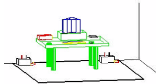
Figure 3. Line Conducted Emission Test Set-Up
