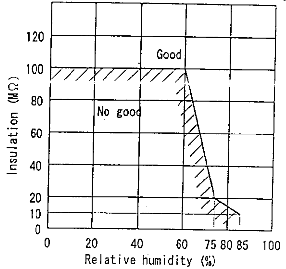
INSULATION
