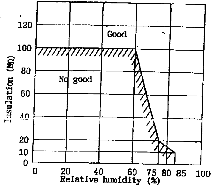
INSULATION
