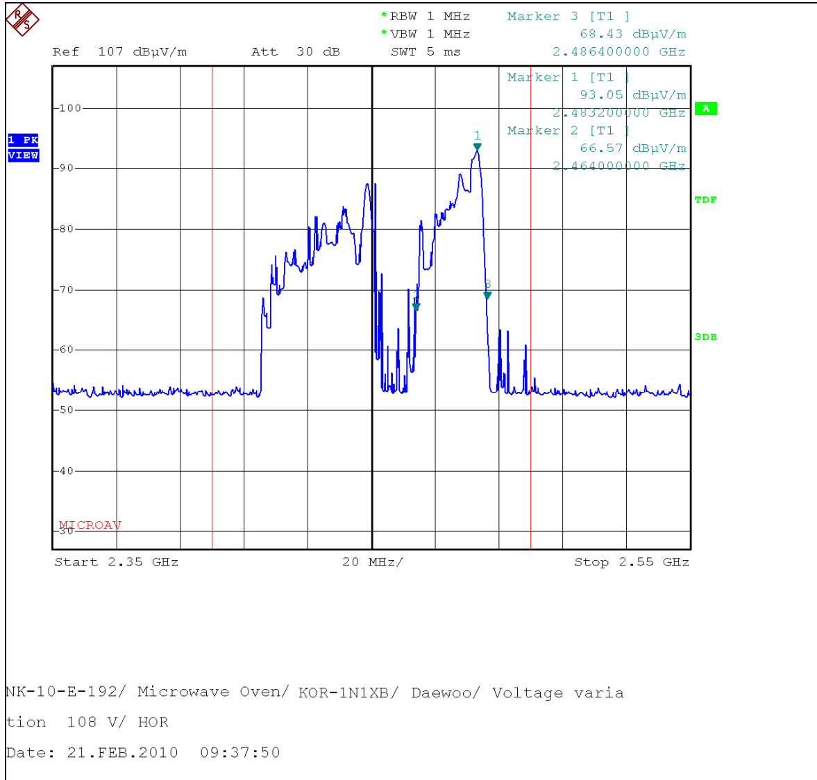
Magnetron : RM259_Horizontal (108 V, 1000 ml)
