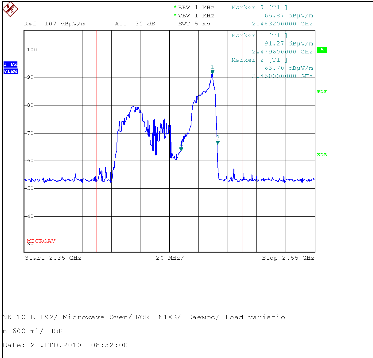
Magnetron : RM259_Horizontal (120 V, 600 ml)
