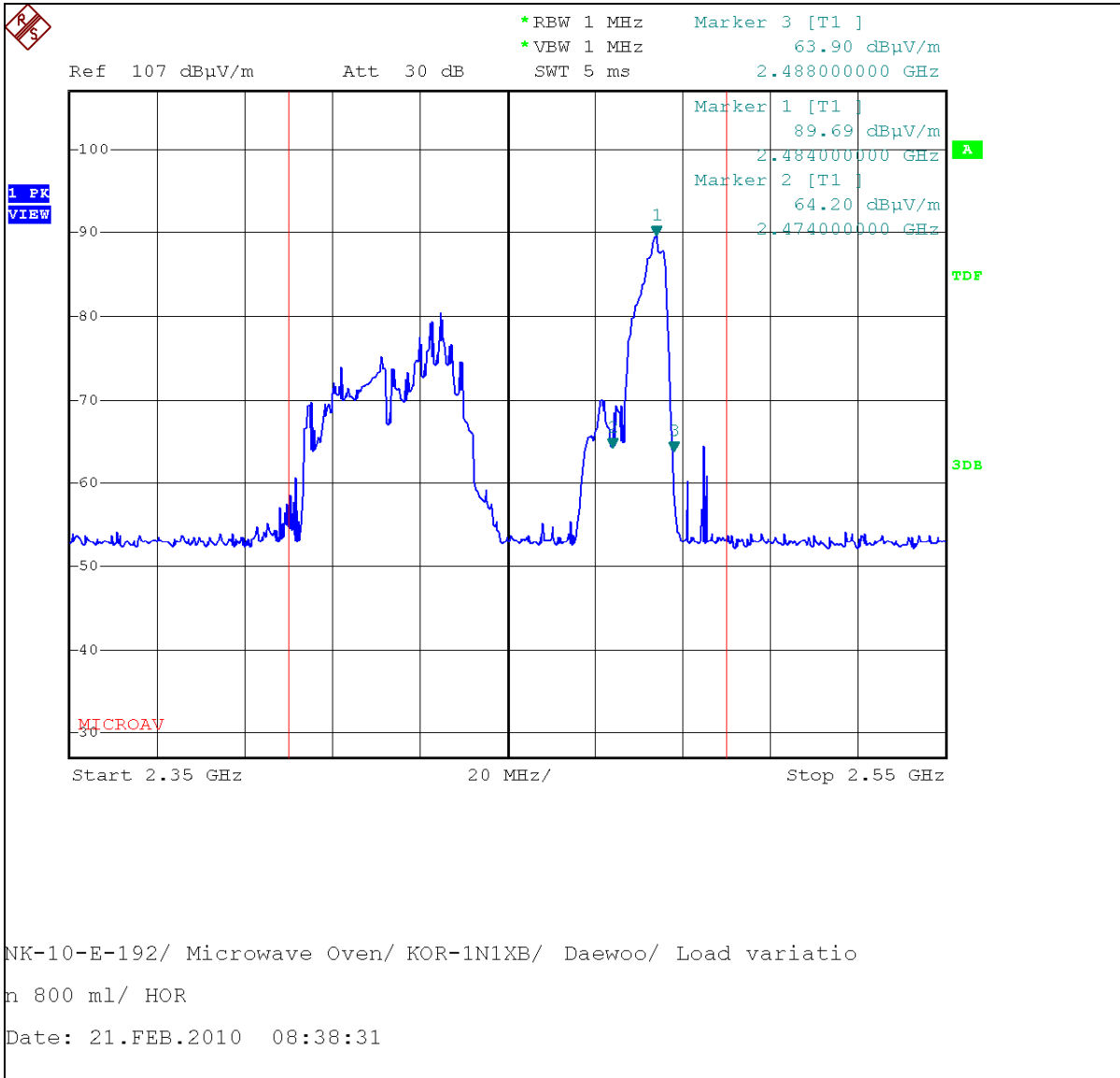
Magnetron : RM259_Horizontal (120 V, 800 ml)
