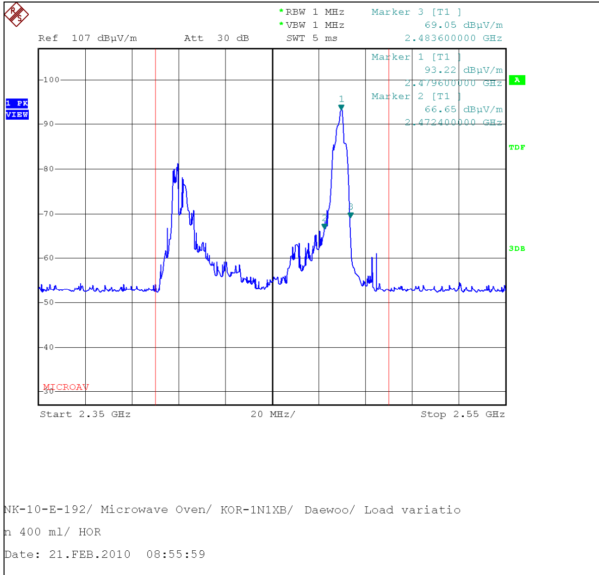
Magnetron : RM259_Horizontal (120 V, 400 ml)
