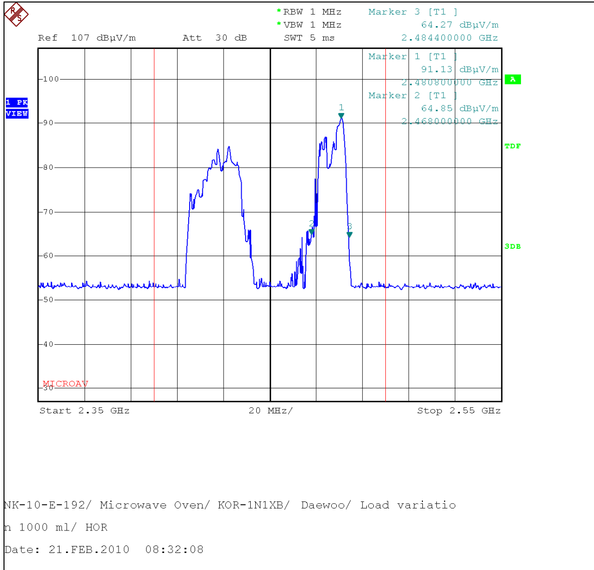
Magnetron : RM259_Horizontal (120 V, 1000 ml)
