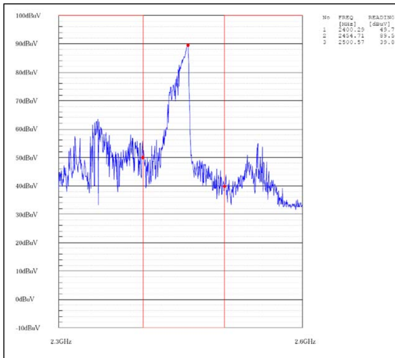
Vertical (132V, 1000cc)
