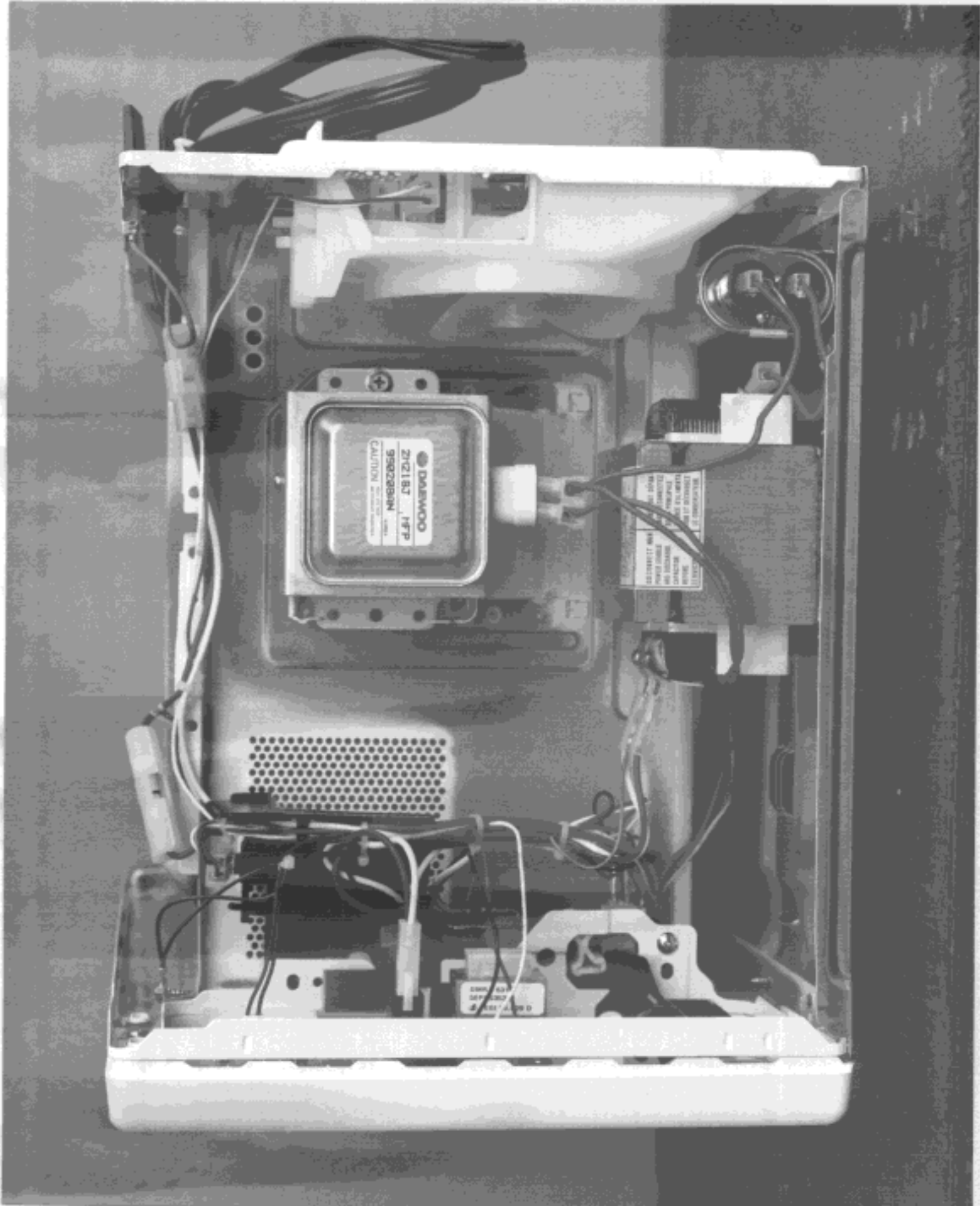
SIDE VIEW ( RIGHT ) - DAEWOO M.G.T ( KOR-1A1G )
