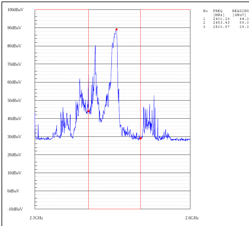
Vertical (120V, 400cc)
