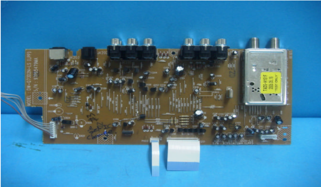
LPP Panel PCB Parts View
