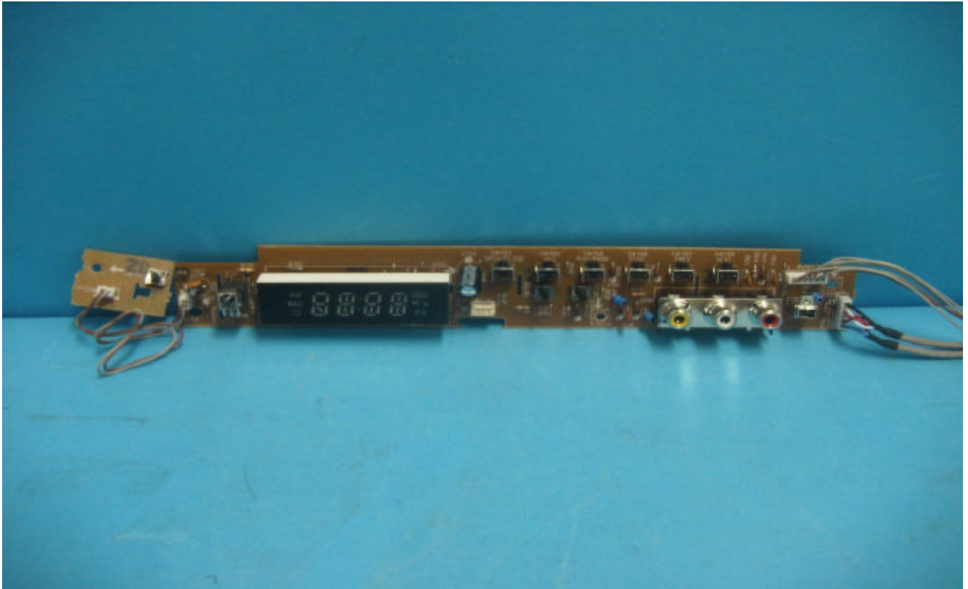
AUX front Input, Control Board PCB Parts View
