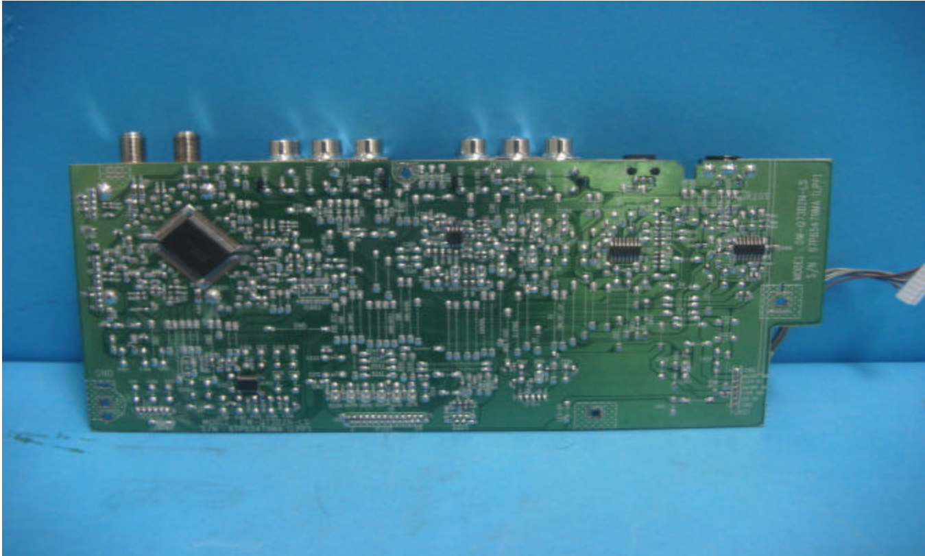
LPP Panel PCB Copper View
