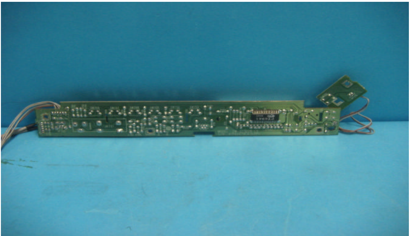
AUX front Input, Control Board PCB Copper View
