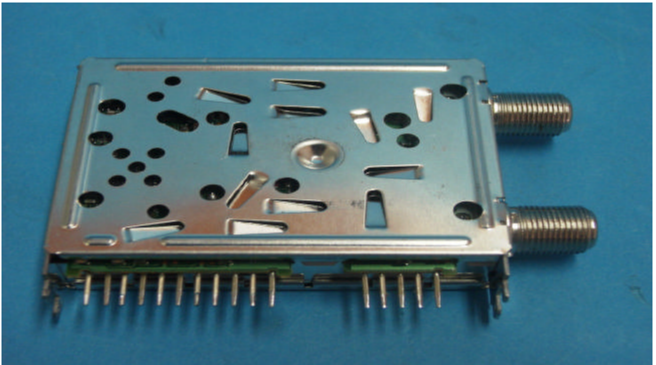
Rear View
