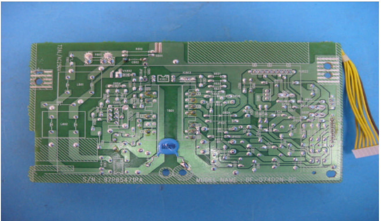
Power Board PCB Copper View
