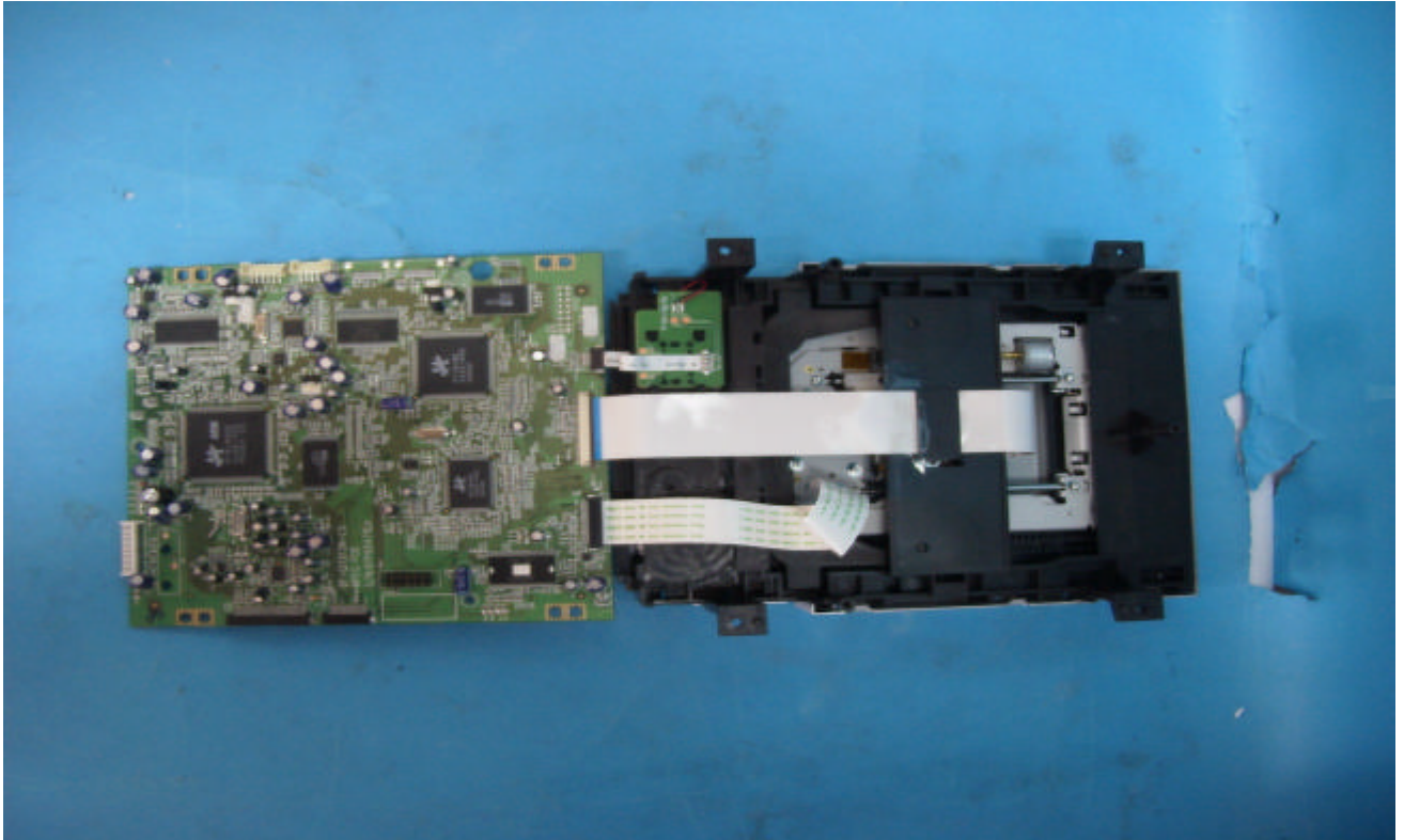
DVD Deck Top View
