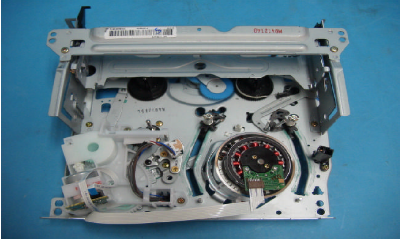
VCR Deck Top View
