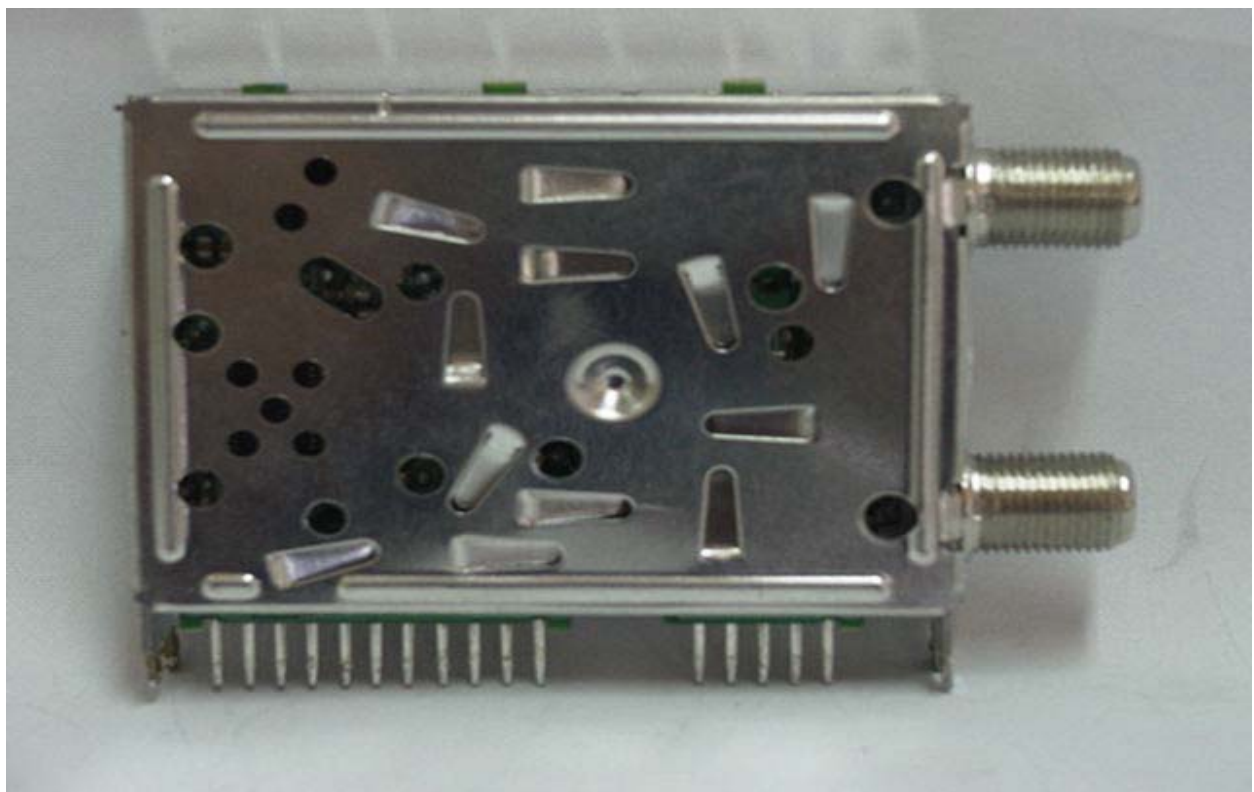
Side View
