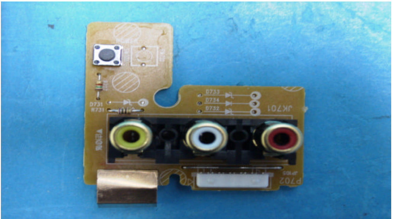
AUX front Input Panel PCB Parts View
