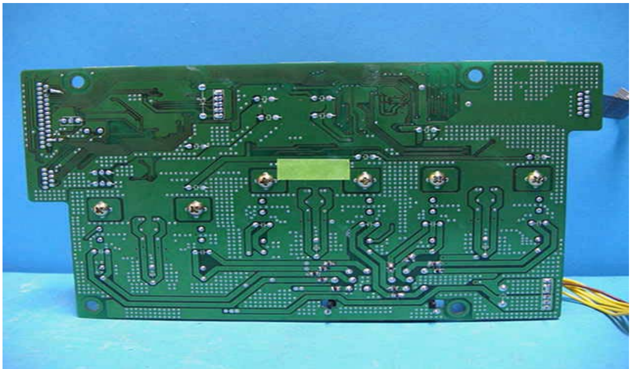
Digital Amp Panel PCB Copper View
