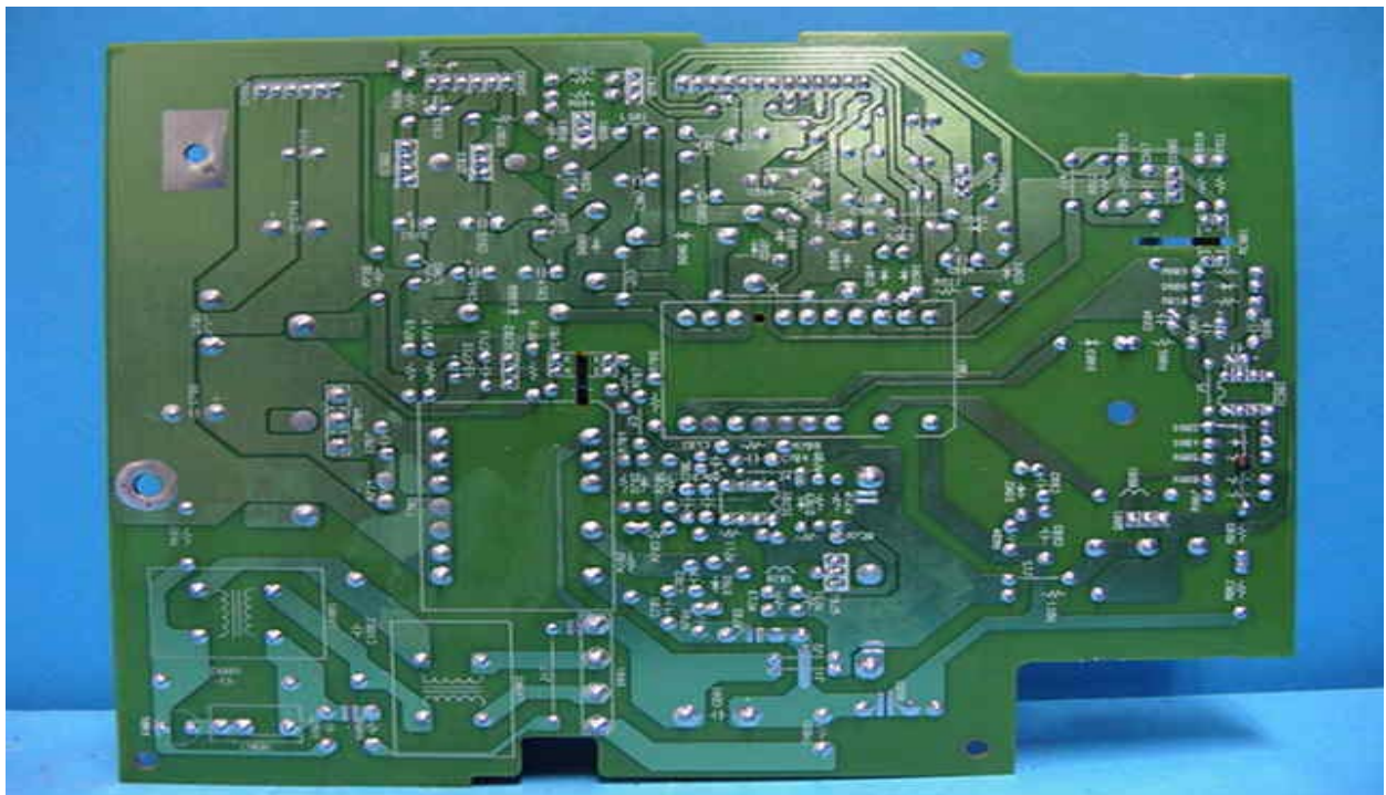
Power Board PCB Copper View
