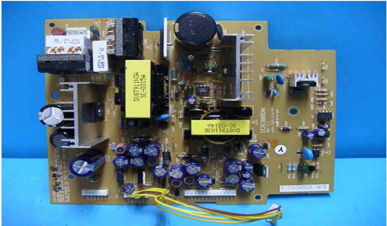
Power Board PCB Parts View
