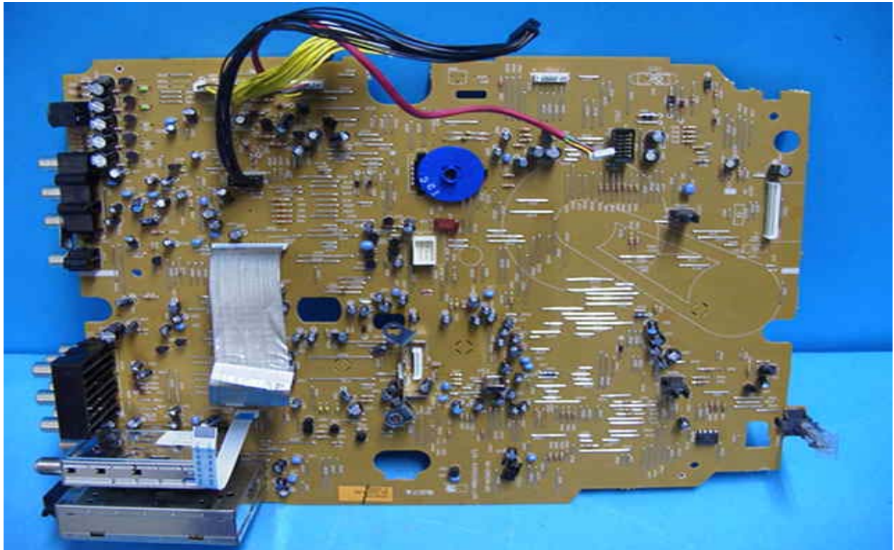
Main Board PCB Parts View
