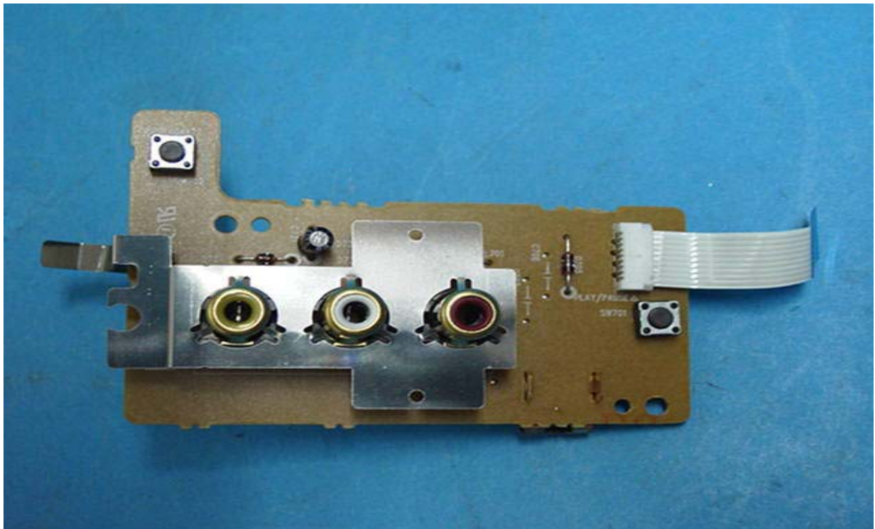
AUX front Input Panel PCB Parts View
