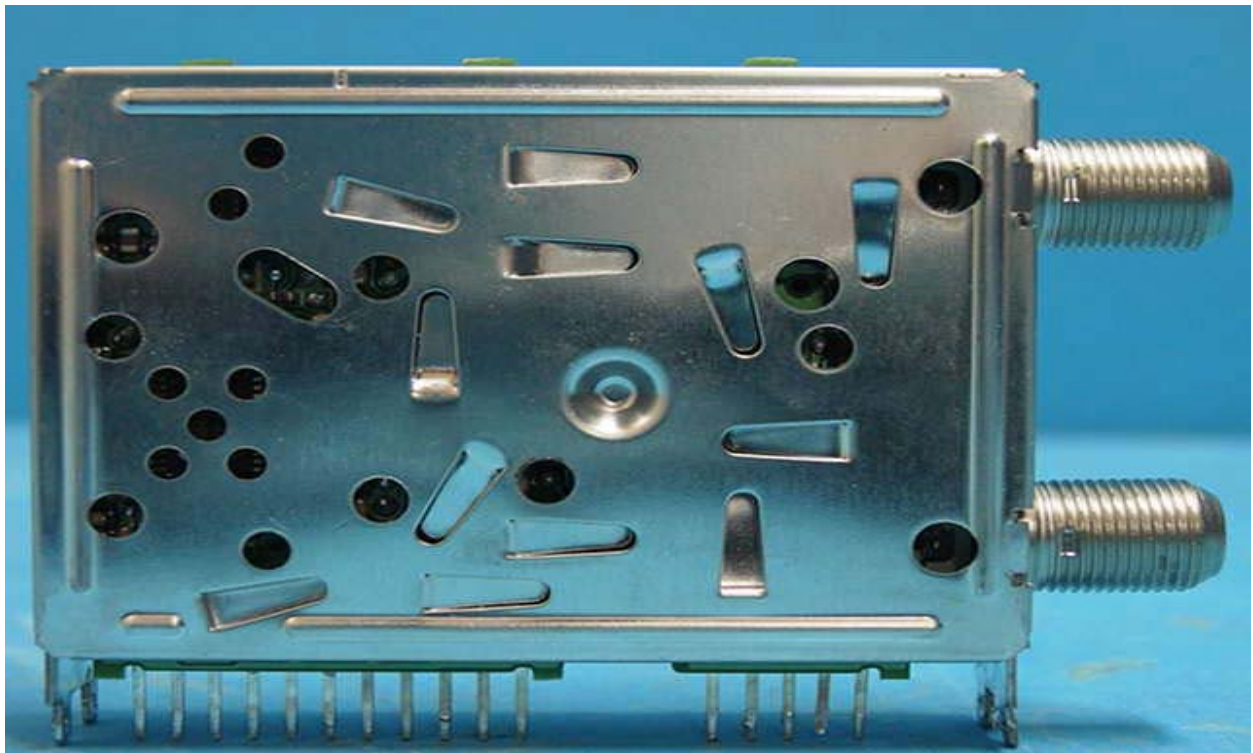
Rear View
