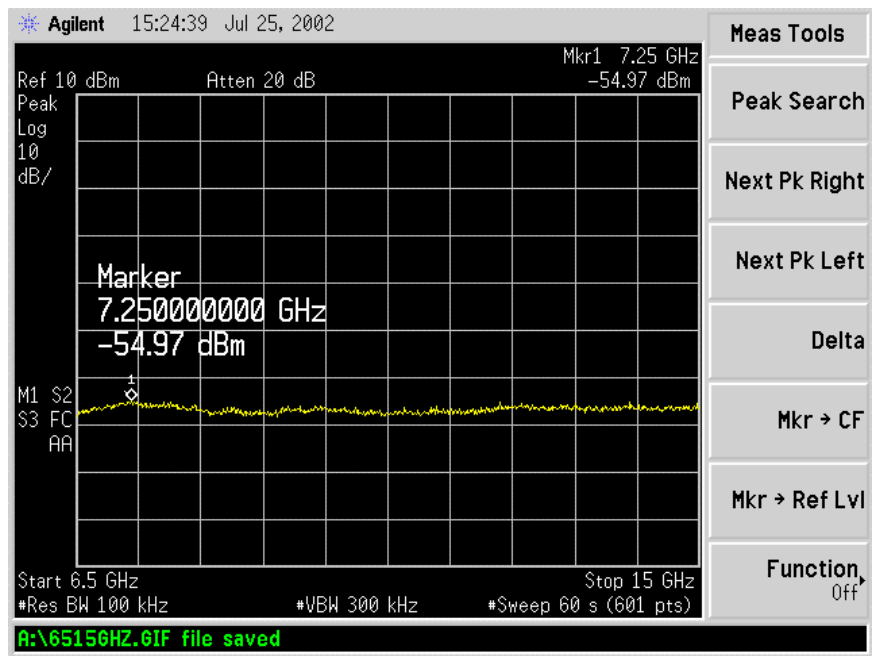
Figure 6.7-7: 6.5 – 15.0GHz Spectrum
