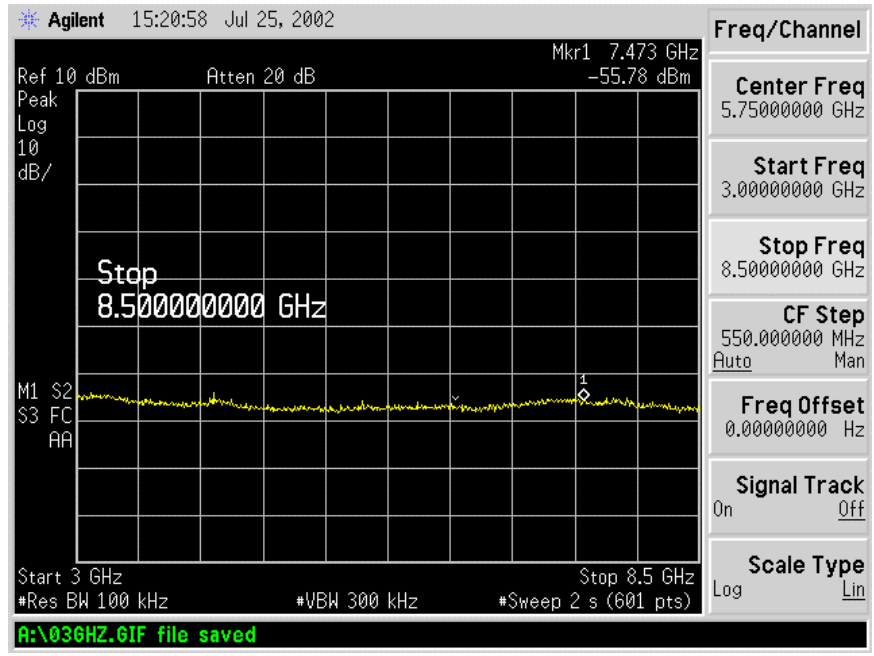
Figure 6.7-6: 3.0 – 8.5GHz Spectrum
