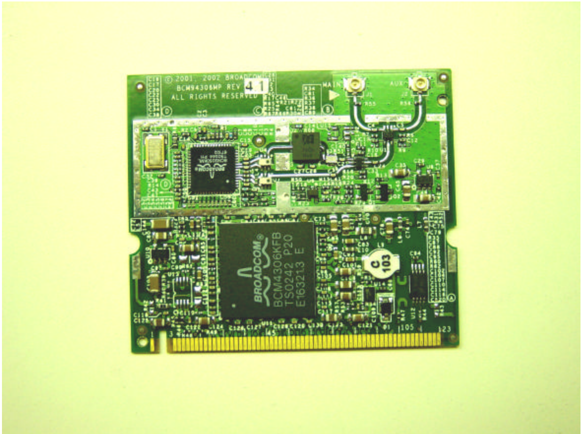
PCB WLAN - Top view
