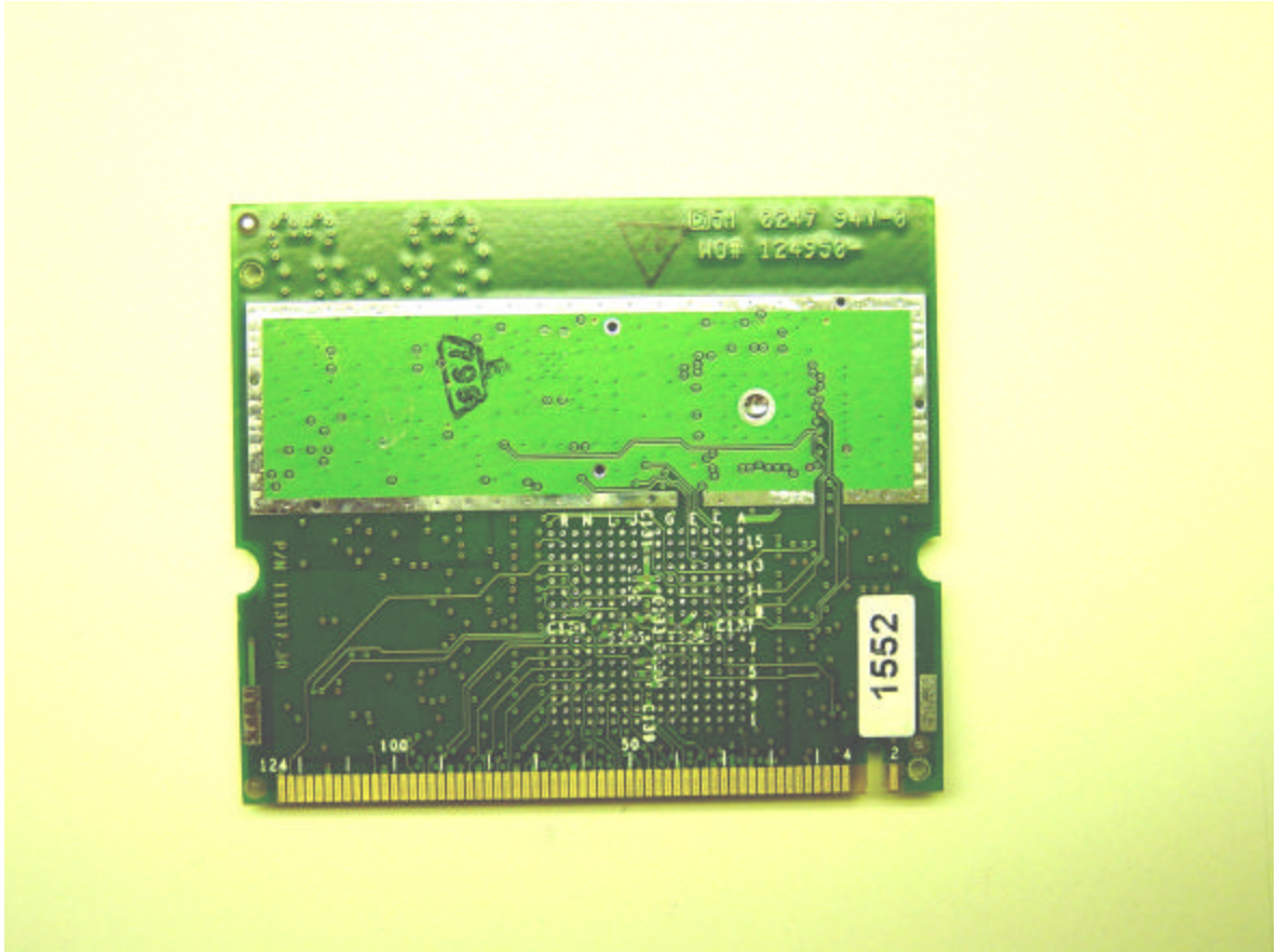
PCB WLAN - Bottom view
