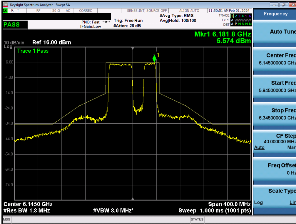
Plot 7-376. In-Band Emission Plot MIMO ANT2 (80MHz BW 802.11be (484+242 Tone) (UNII Band 5) – Ch. 39) - SP
