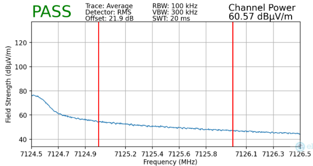
Plot 7-419. Radiated Upper Band Edge Plot MIMO (Average – UNII Band 8 – 242T)
