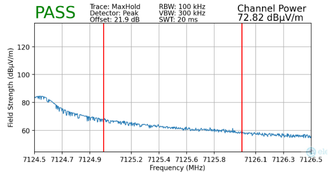
Plot 7-416. Radiated Upper Band Edge Plot MIMO (Peak – UNII Band 8 – 106T)
