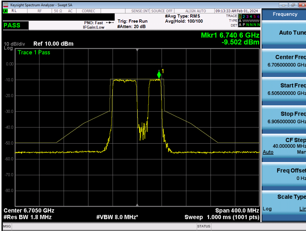
Plot 7-352. In-Band Emission Plot MIMO ANT2 (80MHz BW 802.11be (484+242 Tone) (UNII Band 7) – Ch. 151) - LPI
