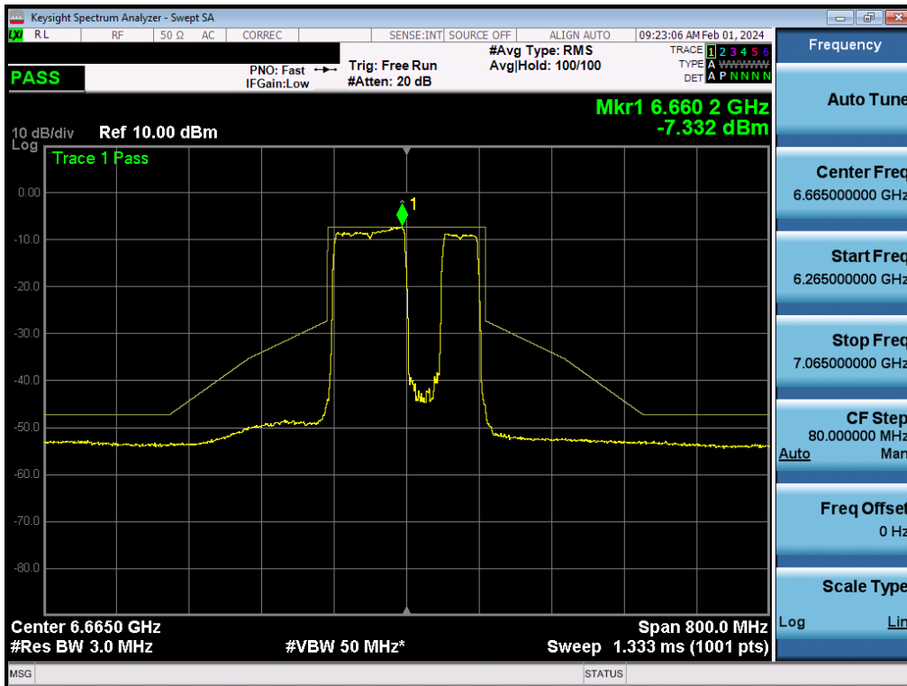
Plot 7-353. In-Band Emission Plot MIMO ANT2 (160MHz BW 802.11be (996+484 Tone) (UNII Band 7) – Ch. 143) - LPI
