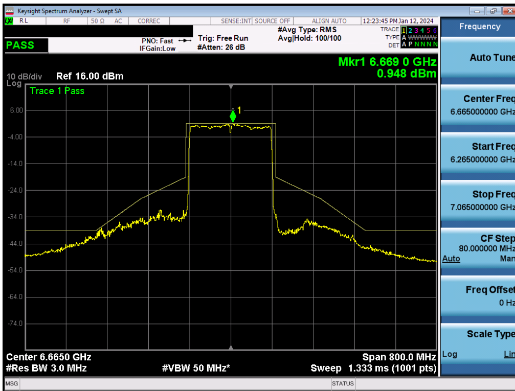
Plot 7-375. In-Band Emission Plot MIMO ANT2 (160MHz BW 802.11be (Full Tone) (UNII Band 7) – Ch. 143) – SP
