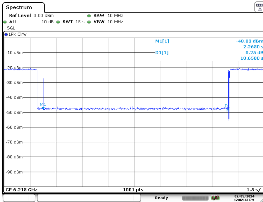
Plot 7-382. Contention Based Protocol Timing Plot (20MHz (UNII Band 5) – Ch. 53)
