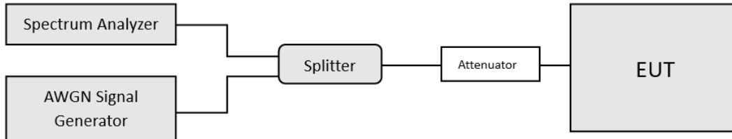
Figure 7-5. Contention-based protocol test setup, conducted method
