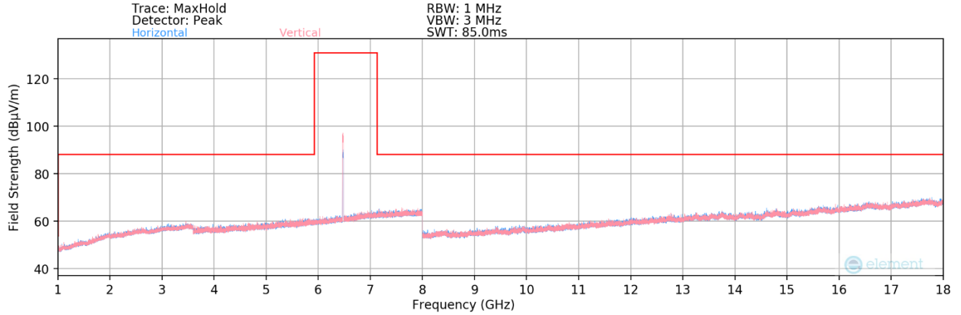
Plot 7-408. Radiated Spurious Plot 1GHz – 18GHz MIMO (802.11be – UNII Band 6 Ch. 105) – LPI
