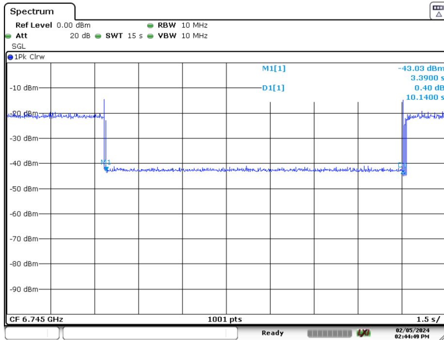
Plot 7-392. Contention Based Protocol Timing Plot (320MHz (UNII Band 7) – Ch. 159 Mid)
