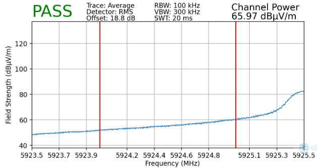
Plot 7-417. Radiated Lower Band Edge Plot MIMO (Average – UNII Band 5 – 242T)
