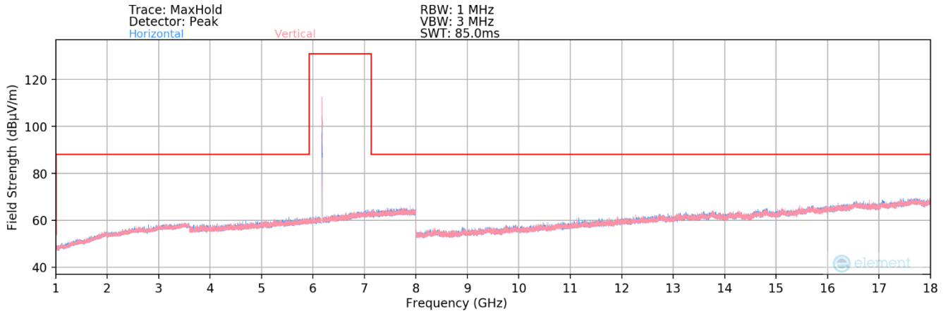
Plot 7-401. Radiated Spurious Plot 1GHz – 18GHz MIMO (802.11be – UNII Band 5 Ch. 45) – SP & LPI
