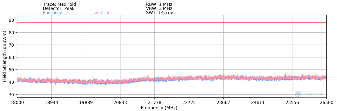
Plot 7-411. Radiated Spurious Plot 18GHz - 26.5GHz (802.11be)
