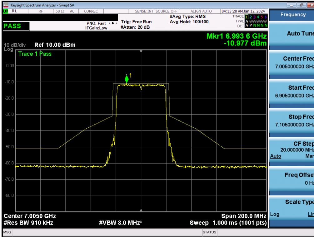
Plot 7-342. In-Band Emission Plot MIMO ANT2 (40MHz BW 802.11be (Full Tone) (UNII Band 8) – Ch. 211) - LPI
