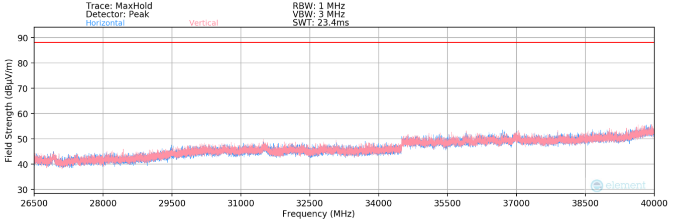
Plot 7-412. Radiated Spurious Plot 26.5GHz - 40GHz (802.11be)
