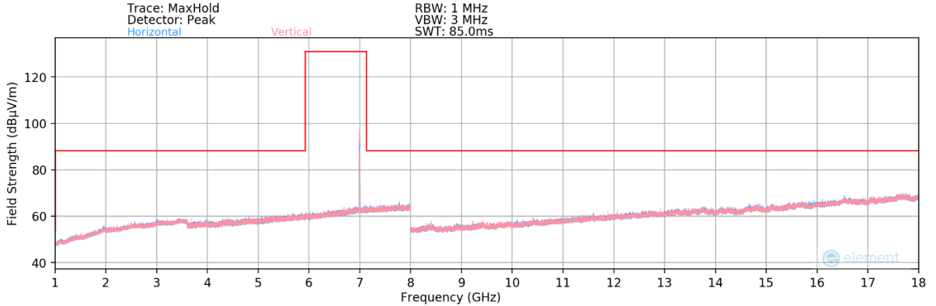
Plot 7-410. Radiated Spurious Plot 1GHz – 18GHz MIMO (802.11be – U Band 8 Ch. 209) – LPI
