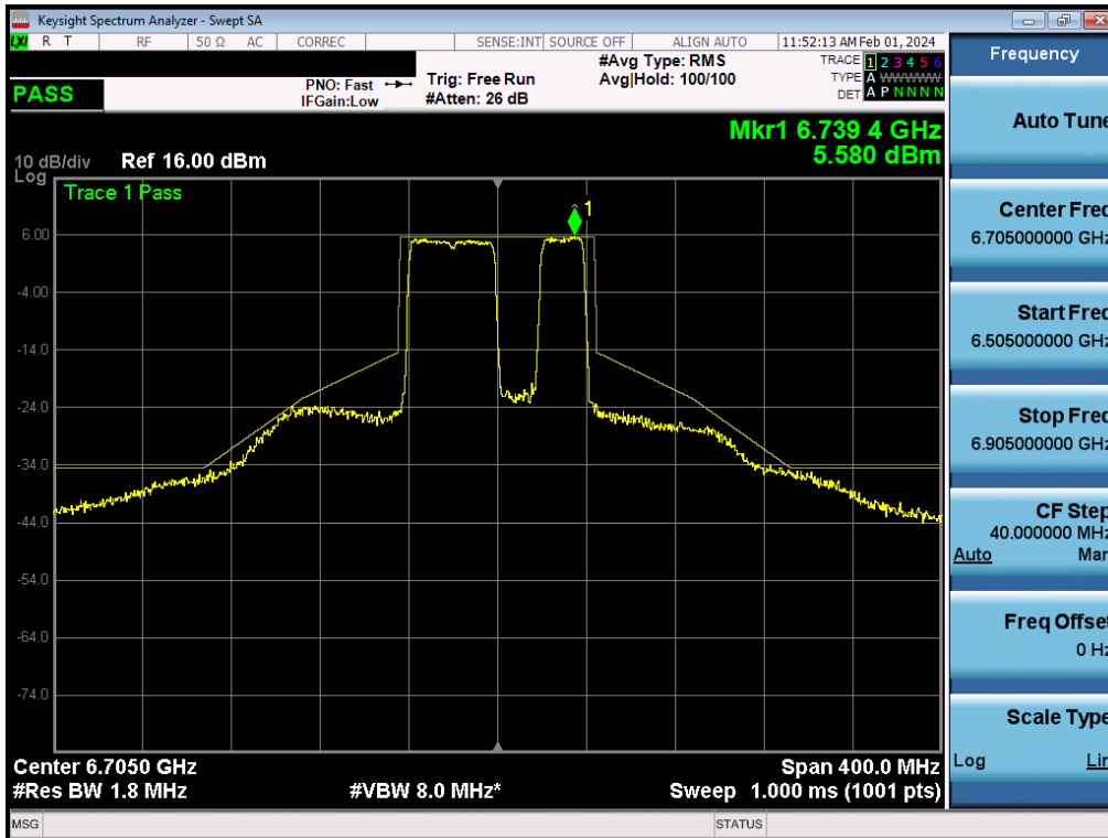
Plot 7-379. In-Band Emission Plot MIMO ANT2 (80MHz BW 802.11be (484+242 Tone) (UNII Band 7) – Ch. 151) - SP
