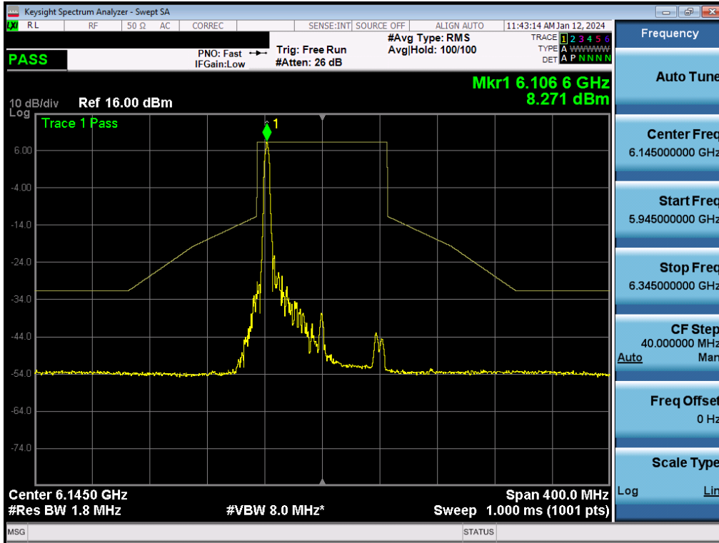
Plot 7-360. In-Band Emission Plot MIMO ANT2 (80MHz BW 802.11be (26 Tones) (UNII Band 5) – Ch. 39) - SP
