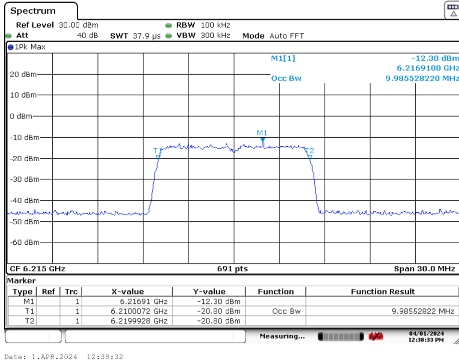
Plot 7-381. AWGN Signal (Demonstration)
