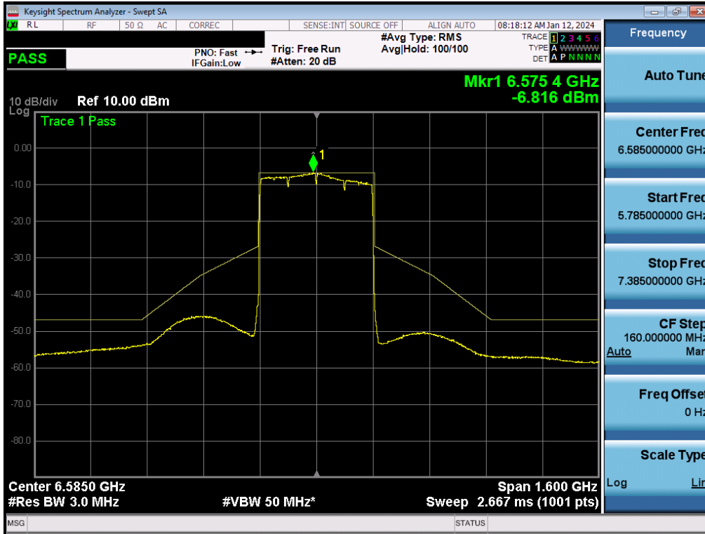
Plot 7-340. In-Band Emission Plot MIMO ANT2 (320MHz BW 802.11be (Full Tone) (UNII Band 7) – Ch. 127) - LPI
