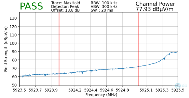
Plot 7-418. Radiated Lower Band Edge Plot MIMO (Peak – UNII Band 5 – 242T)
