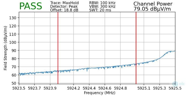
Plot 7-414. Radiated Lower Band Edge Plot MIMO (Peak – UNII Band 5 – 106T)
