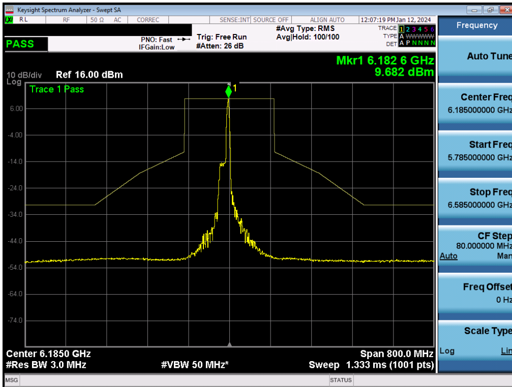
Plot 7-361. In-Band Emission Plot MIMO ANT2 (160MHz BW 802.11be (26 Tones) (UNII Band 5) – Ch. 47) - SP
