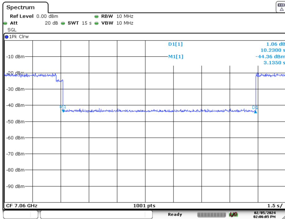
Plot 7-396. Contention Based Protocol Timing Plot (320MHz (UNII Band 8) – Ch. 191 Mid)
