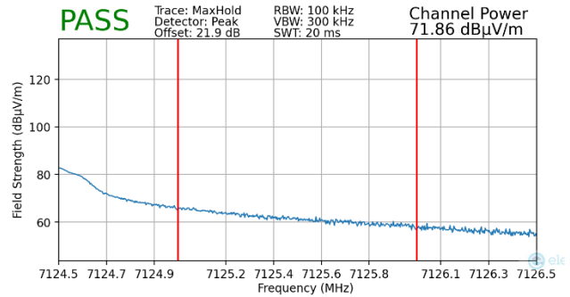
Plot 7-420. Radiated Upper Band Edge Plot MIMO (Peak – UNII Band 8 – 242T)
