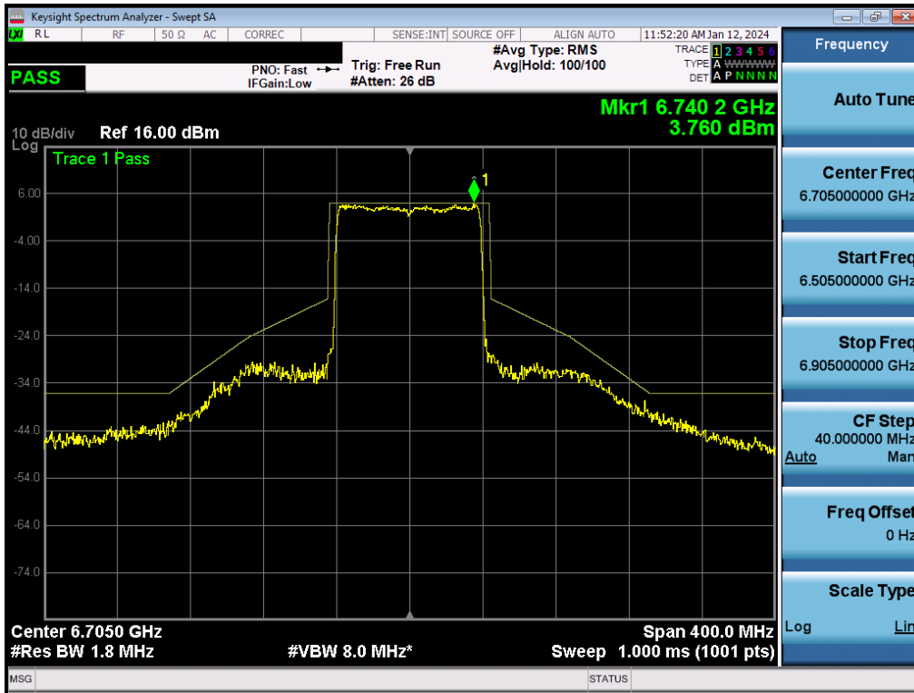
Plot 7-374. In-Band Emission Plot MIMO ANT2 (80MHz BW 802.11be (Full Tone) (UNII Band 7) – Ch. 151) – SP
