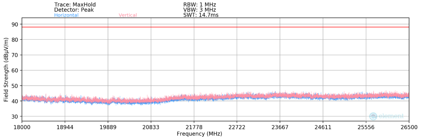
Plot 7-405. Radiated Spurious Plot 18GHz - 26.5GHz (802.11be)
