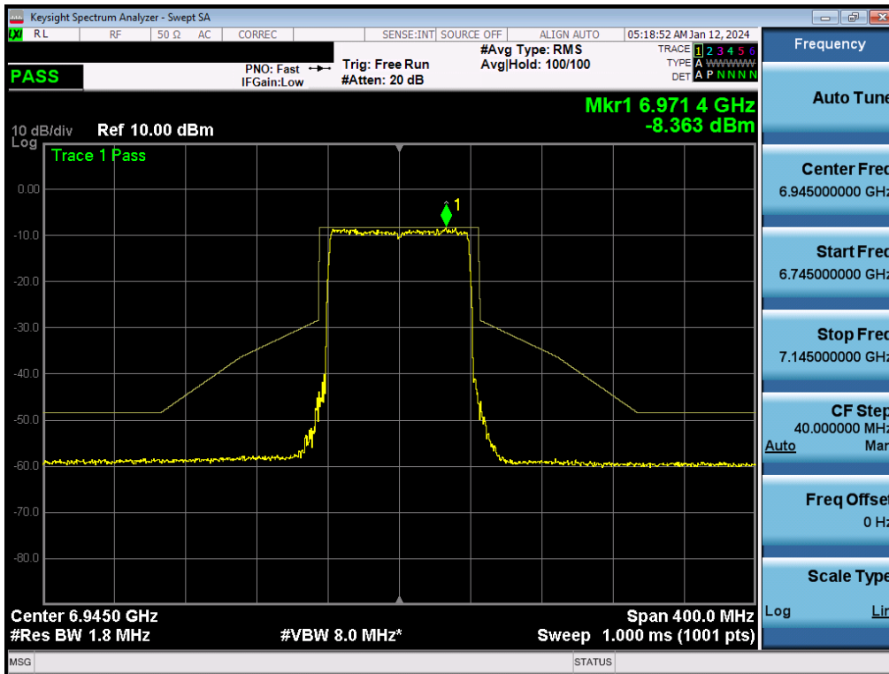
Plot 7-343. In-Band Emission Plot MIMO ANT2 (80MHz BW 802.11be (Full Tone) (UNII Band 8) – Ch. 199) - LPI
