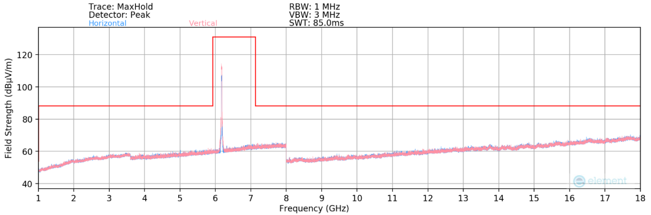
Plot 7-407. Radiated Spurious Plot 1GHz – 18GHz MIMO (802.11be – UNII Band 5 Ch. 45) - SP & LPI
