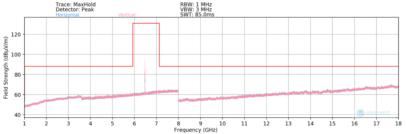
Plot 7-402. Radiated Spurious Plot 1GHz – 18GHz MIMO (802.11be – UNII Band 6 Ch. 105) – LPI
