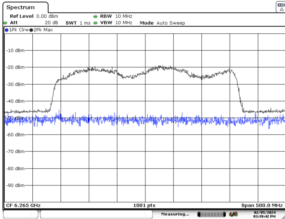
Plot 7-398. CBP 320MHz Channel - Injection Lower Edge – [6110 MHz]
