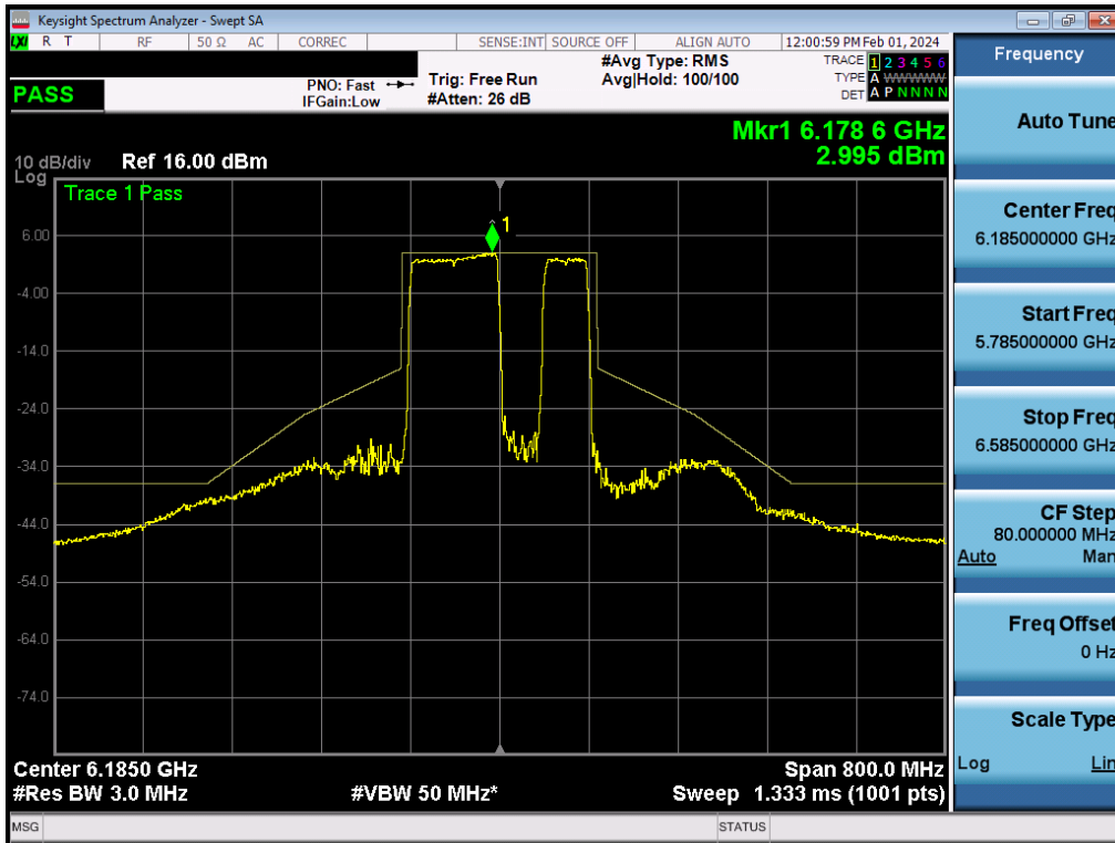
Plot 7-377. In-Band Emission Plot MIMO ANT2 (160MHz BW 802.11be (996+484 Tone) (UNII Band 5) – Ch. 47) - SP
