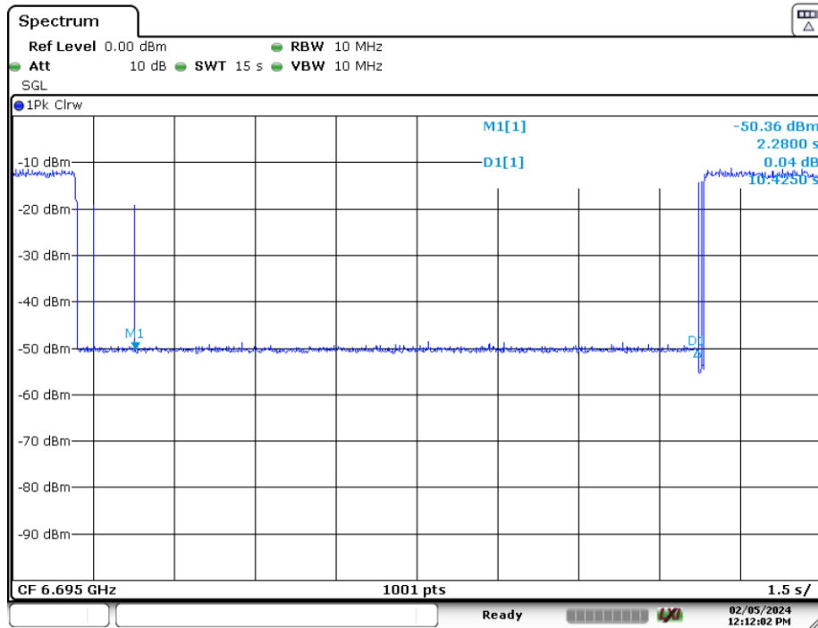
Plot 7-390. Contention Based Protocol Timing Plot (20MHz (UNII Band 7) – Ch. 149)
