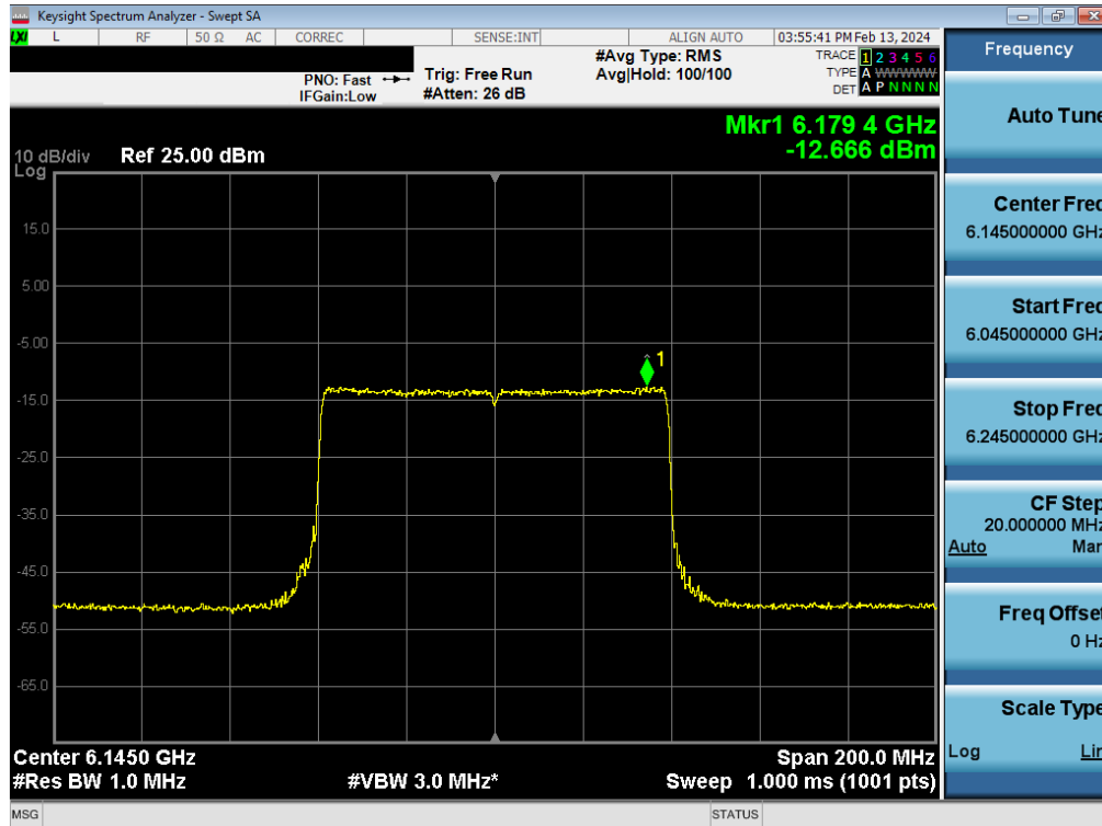
Plot 7-103. Power Spectral Density Plot MIMO ANT1 (80MHz BW 802.11be (Full Tone) (UNII Band 5) – Ch. 39) - LPI
