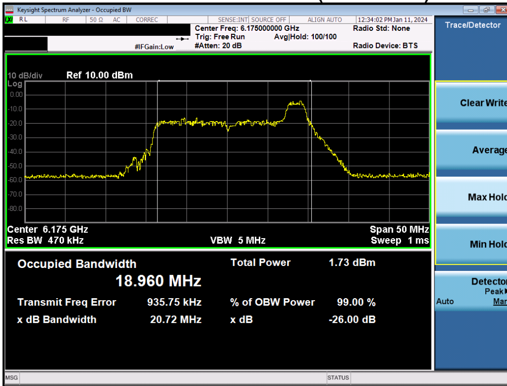
Plot 7-41. Occupied Bandwidth Plot MIMO ANT2 (20MHz BW 802. 11be (26 Tones) (UNII Band 5) – Ch. 45)
