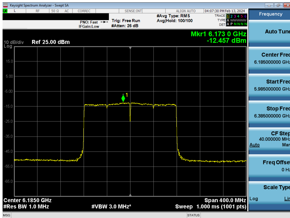
Plot 7-104. Power Spectral Density Plot MIMO ANT1 (160MHz BW 802.11be (Full Tone) (UNII Band 5) – Ch. 47) - LPI
