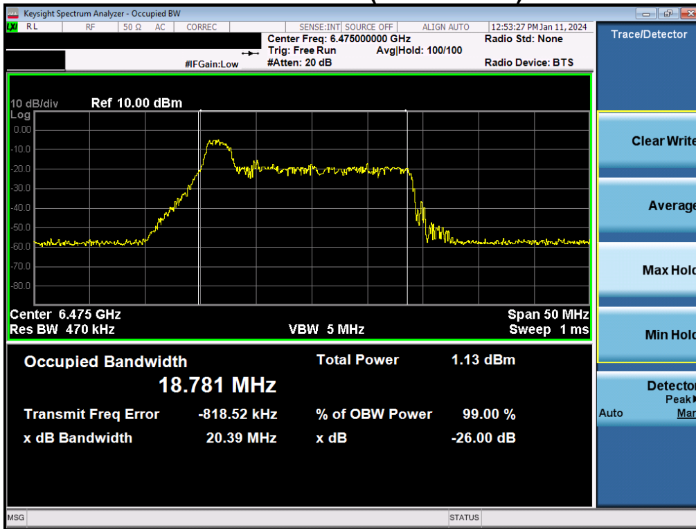
Plot 7-46. Occupied Bandwidth Plot MIMO ANT2 (20MHz BW 802. 11be (26 Tones) (UNII Band 6) – Ch. 105)
