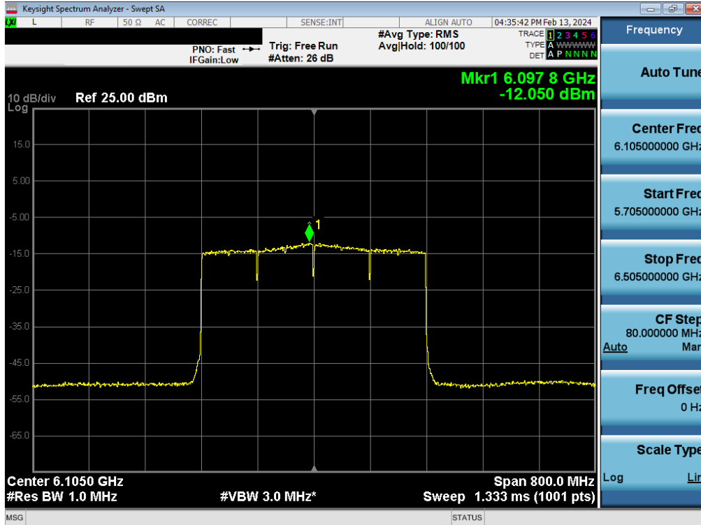
Plot 7-105. Power Spectral Density Plot MIMO ANT1 (320MHz BW 802.11be (Full Tone) (UNII Band 5) – Ch. 31) - LPI
