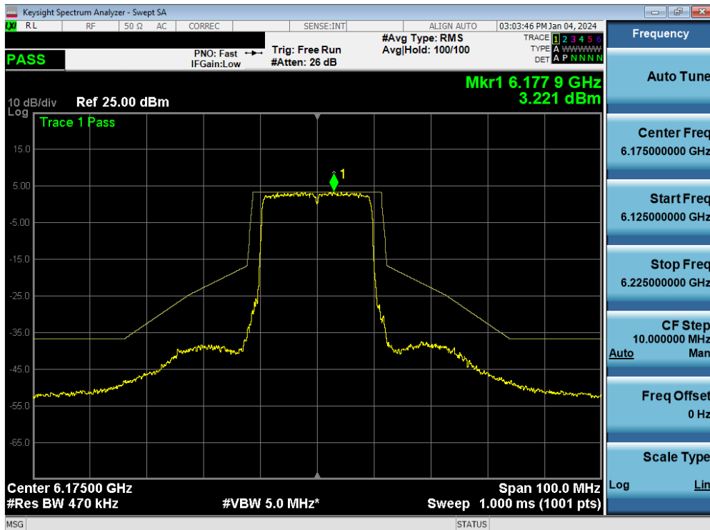
Plot 7-126. In-Band Emission MIMO ANT1 (20MHz 802.11ax/be (UNII Band 5) – Ch. 45) - SP
