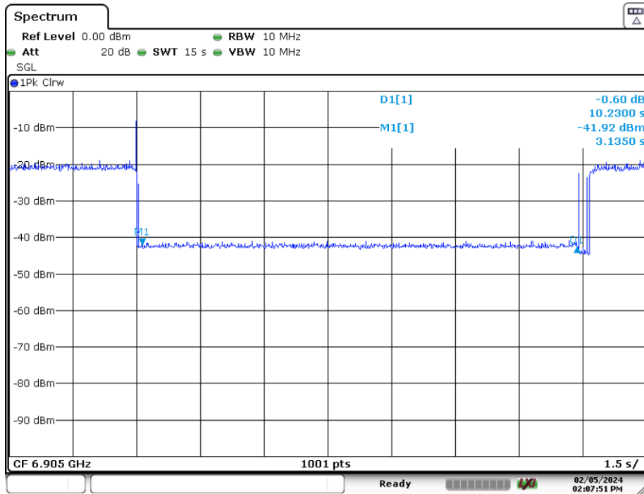
Plot 7-205. Contention Based Protocol Timing Plot (320MHz (UNII Band 8) – Ch. 191 Mid)
