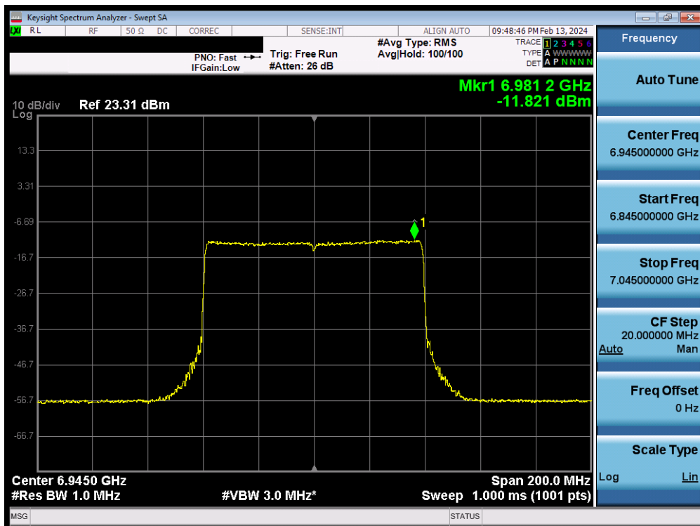
Plot 7-116. Power Spectral Density MIMO ANT2 (80MHz 802.11ax/be (UNII Band 8) – Ch. 199) - LPI
