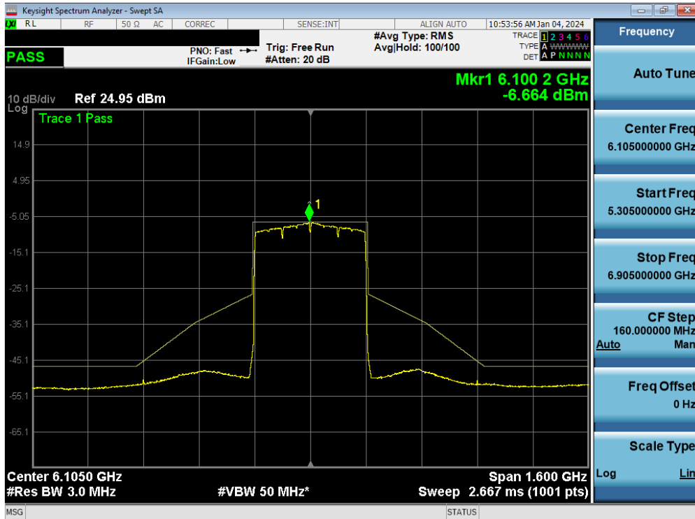
Plot 7-124. In-Band Emission MIMO ANT1 (320MHz 802.11ax/be (UNII Band 5) – Ch.31)
