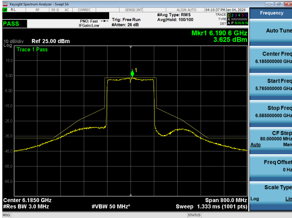
Plot 7-129. In-Band Emission MIMO ANT1 (160MHz 802.11ax/be (UNII Band 5) – Ch. 47) – SP
