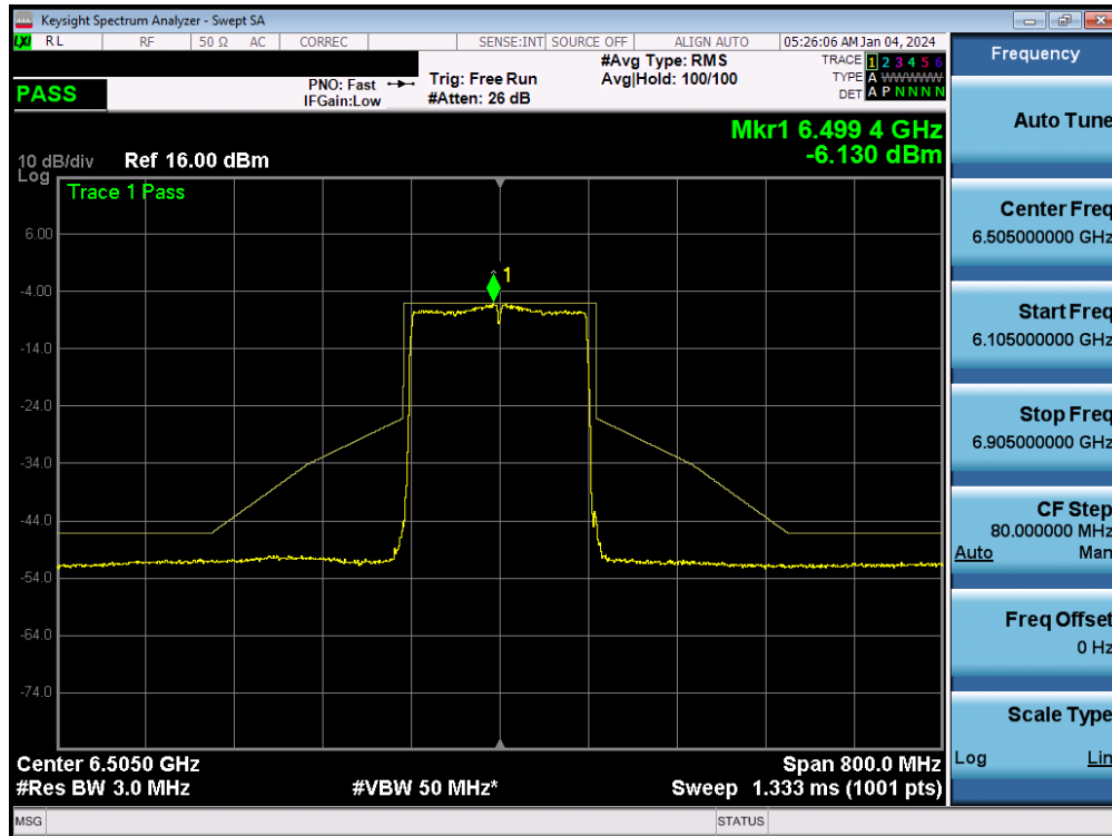
Plot 7-171. In-Band Emission MIMO ANT2 (160MHz 802.11ax/be (UNII Band 6) – Ch. 111)
