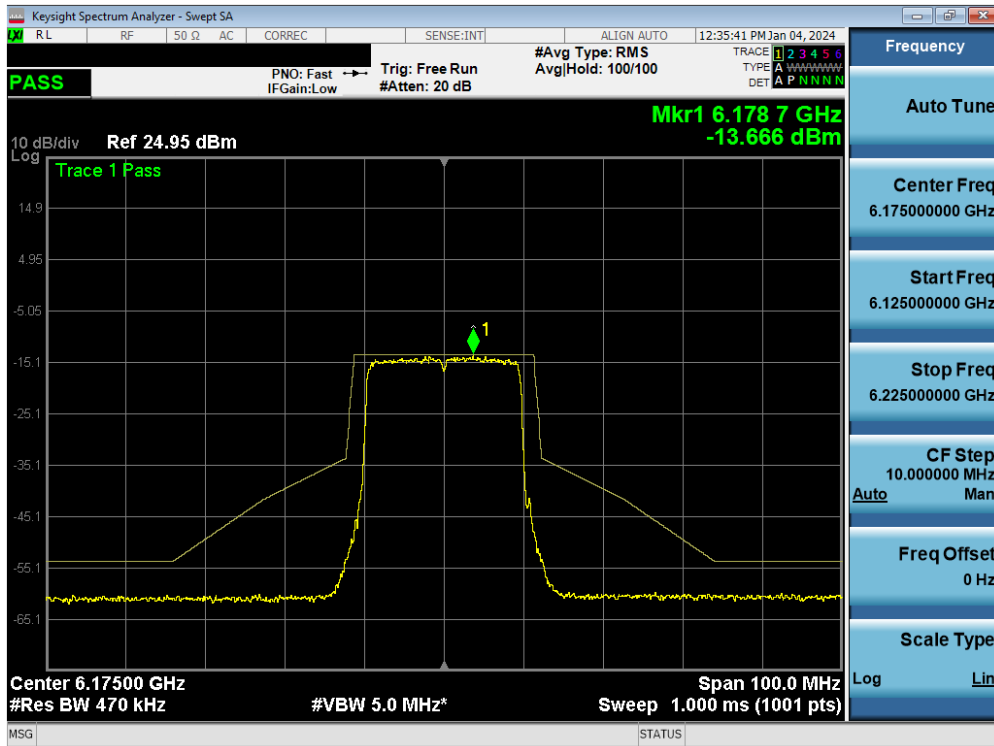
Plot 7-120. In-Band Emission MIMO ANT1 (20MHz 802.11ax/be (UNII Band 5) – Ch. 45)
