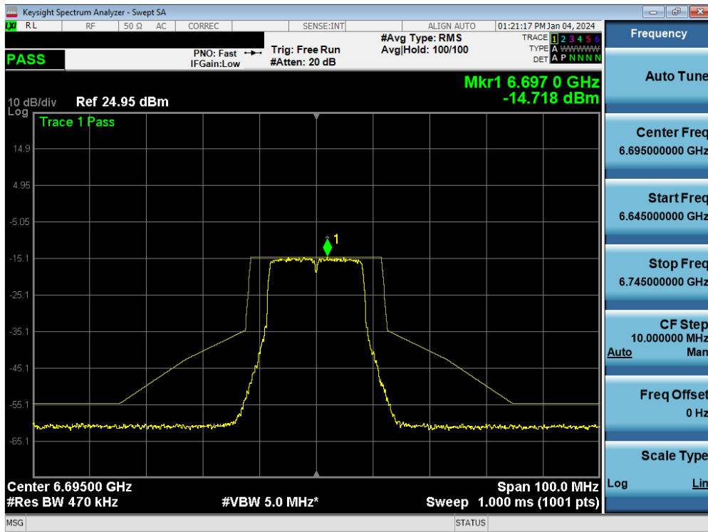
Plot 7-137. In-Band Emission MIMO ANT1 (20MHz 802.11a (UNII Band 7) – Ch. 149)
