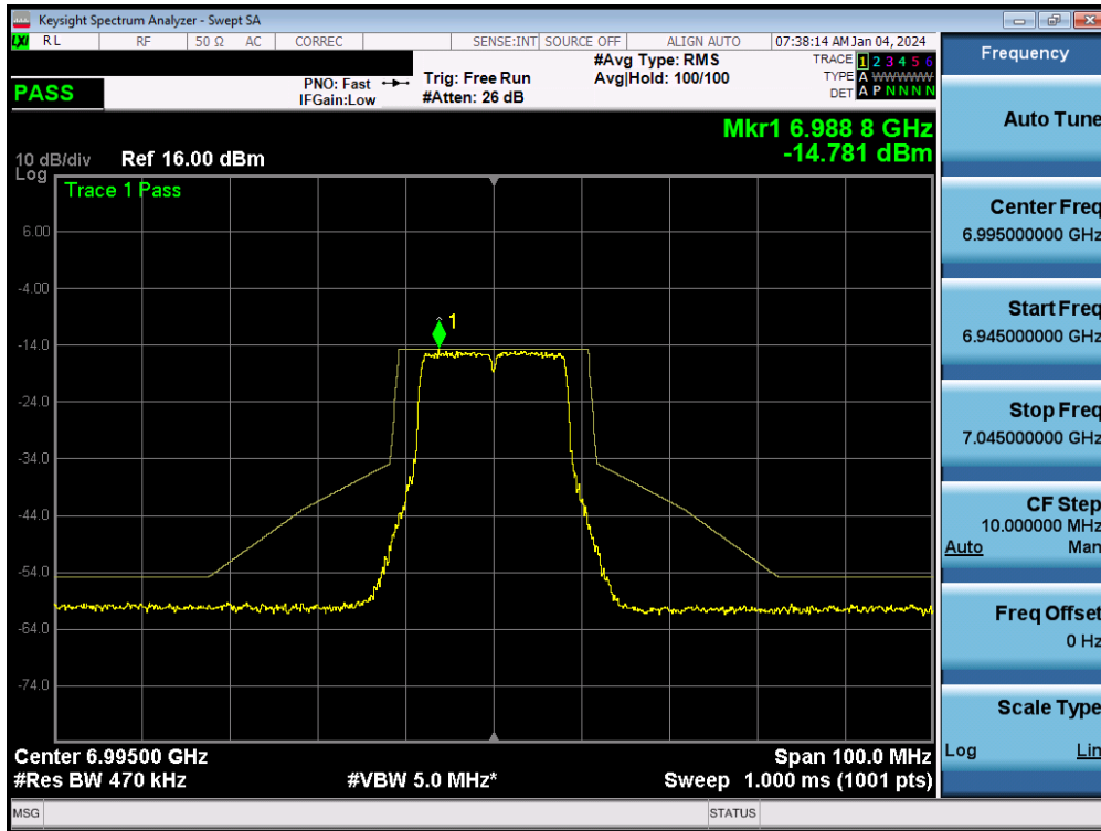
Plot 7-184. In-Band Emission MIMO ANT2 (20MHz 802.11a (UNII Band 8) – Ch. 209)
