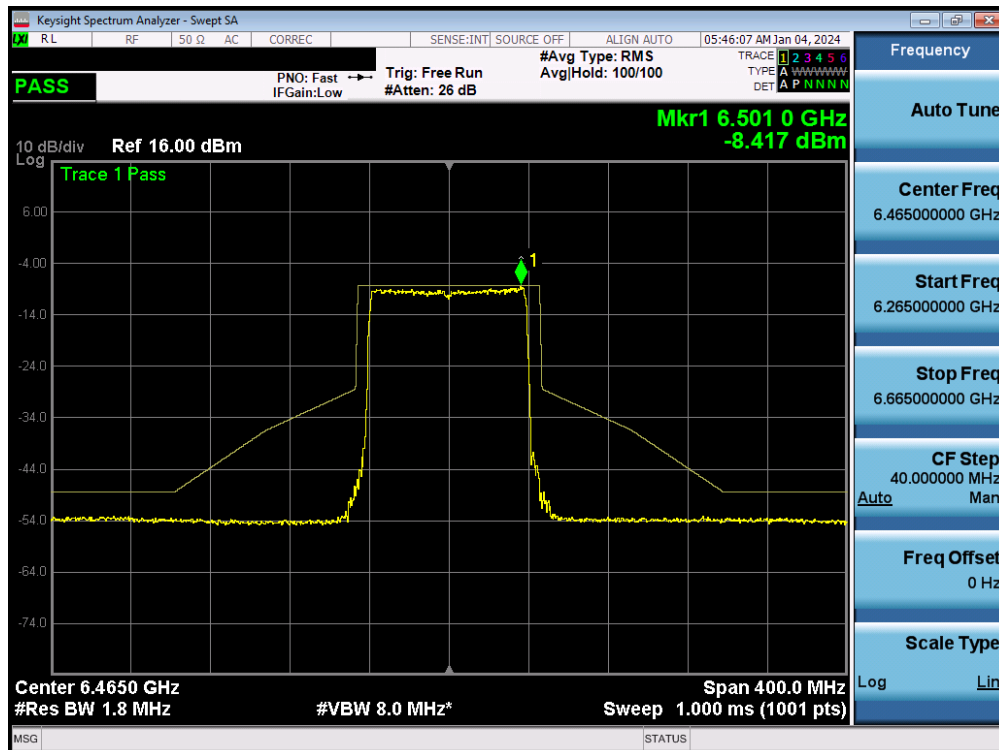
Plot 7-170. In-Band Emission MIMO ANT2 (80MHz 802.11ax/be (UNII Band 6) – Ch. 103)
