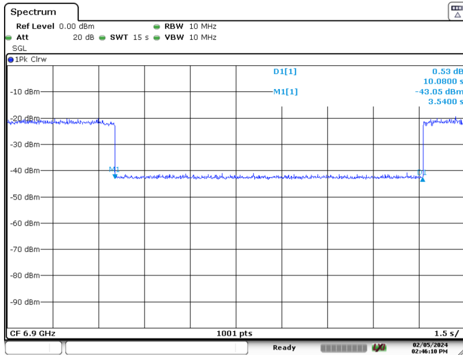
Plot 7-201. Contention Based Protocol Timing Plot (320MHz (UNII Band 7) – Ch. 159 Mid)
