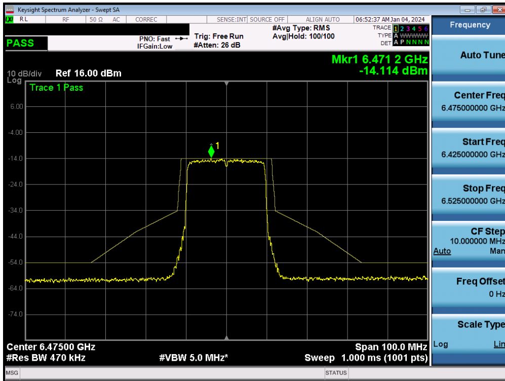
Plot 7-168. In-Band Emission MIMO ANT2 (20MHz 802.11ax/be (UNII Band 6) – Ch. 105)
