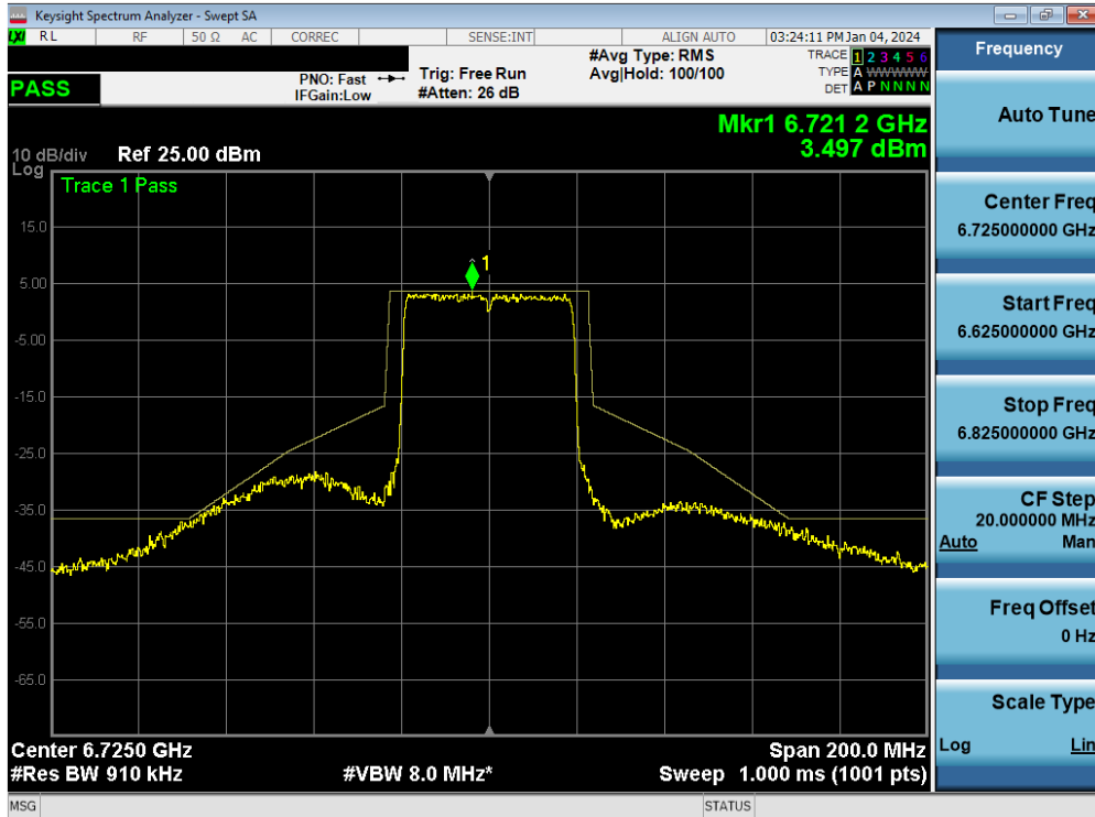
Plot 7-157. In-Band Emission MIMO ANT1 (40MHz 802.11ax/be (UNII Band 7) – Ch. 155) – SP
