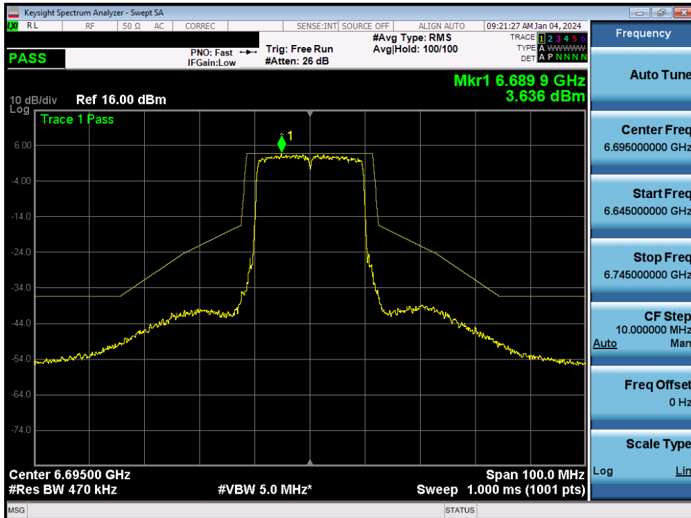
Plot 7-180. In-Band Emission MIMO ANT2 (20MHz 802.11ax/be (UNII Band 7) – Ch. 149) - SP
