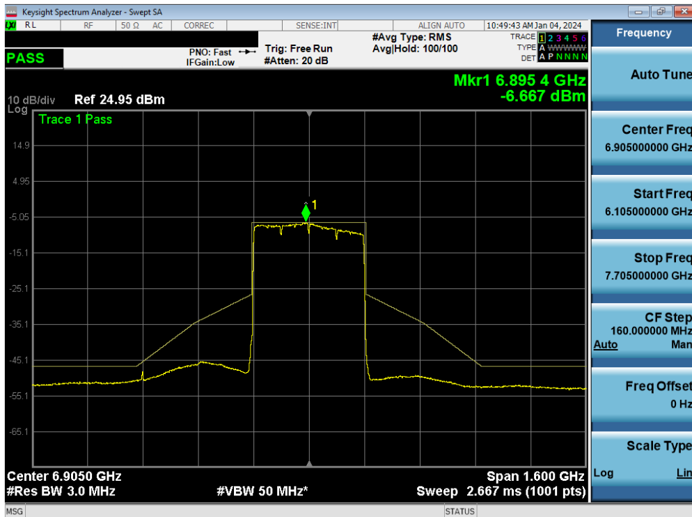
Plot 7-148. In-Band Emission MIMO ANT1 (320MHz 802.11ax/be (UNII Band 7/8) – Ch. 191)
