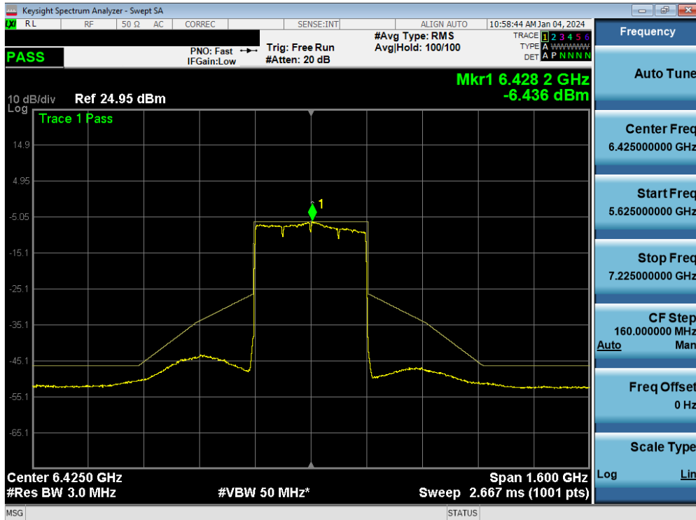
Plot 7-136. In-Band Emission MIMO ANT1 (320MHz 802.11ax/be (UNII Band 5/6/7) – Ch. 95)
