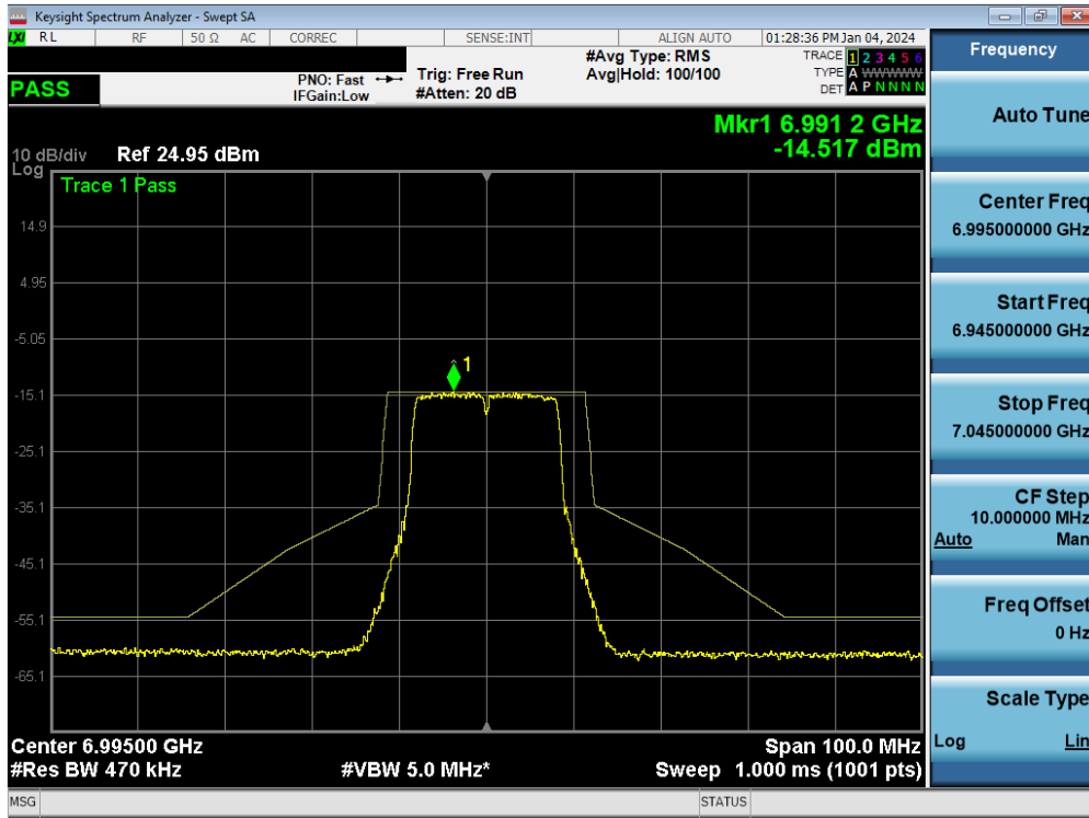
Plot 7-143. In-Band Emission MIMO ANT1 (20MHz 802.11a (UNII Band 8) – Ch. 209)
