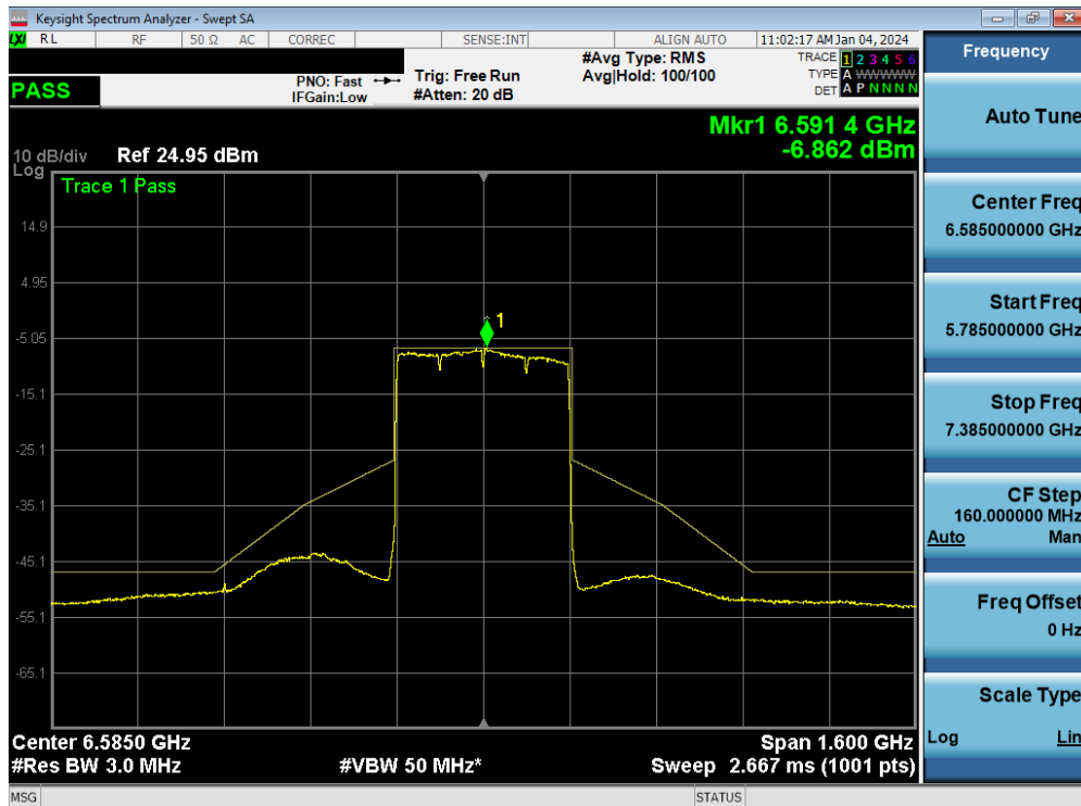
Plot 7-142. In-Band Emission MIMO ANT1 (320MHz 802.11ax/be (UNII Band 6/7) – Ch. 127)
