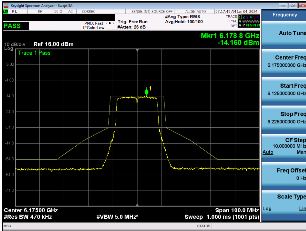
Plot 7-149. In-Band Emission MIMO ANT2 (20MHz 802.11a (UNII Band 5) – Ch. 45)
