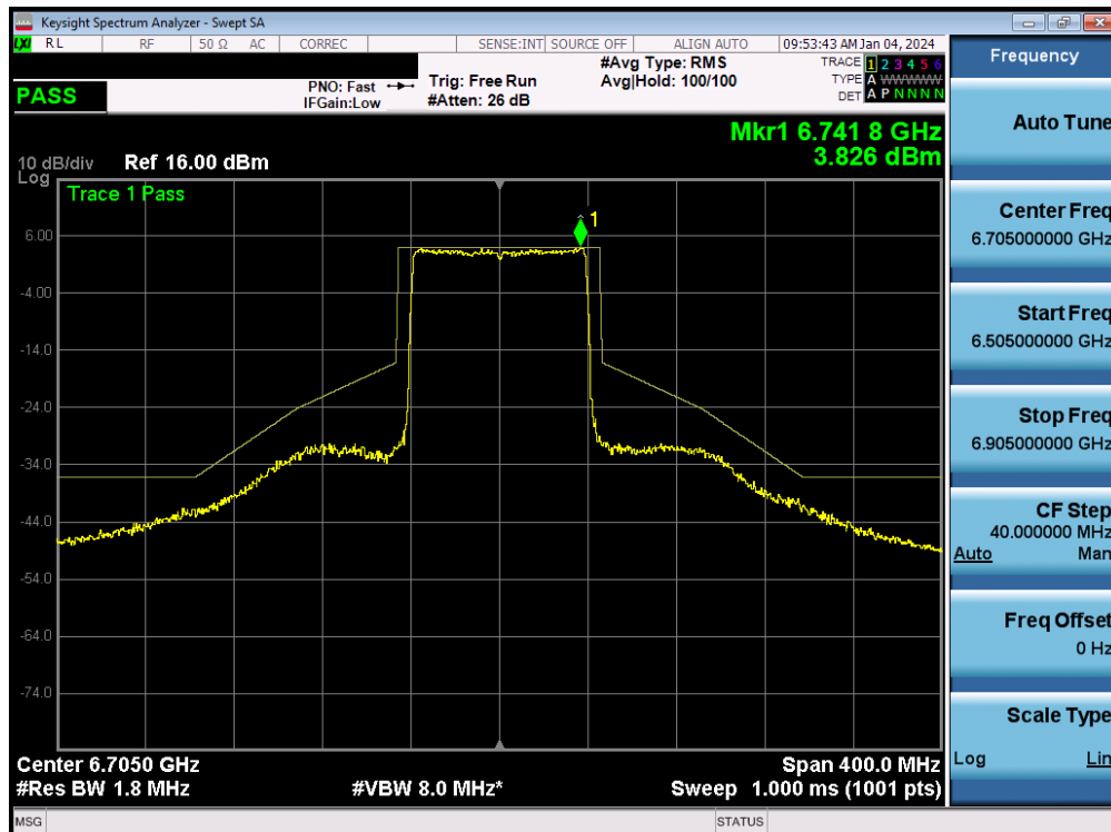
Plot 7-182. In-Band Emission MIMO ANT2 (80MHz 802.11ax/be (UNII Band 7) – Ch. 151) – SP
