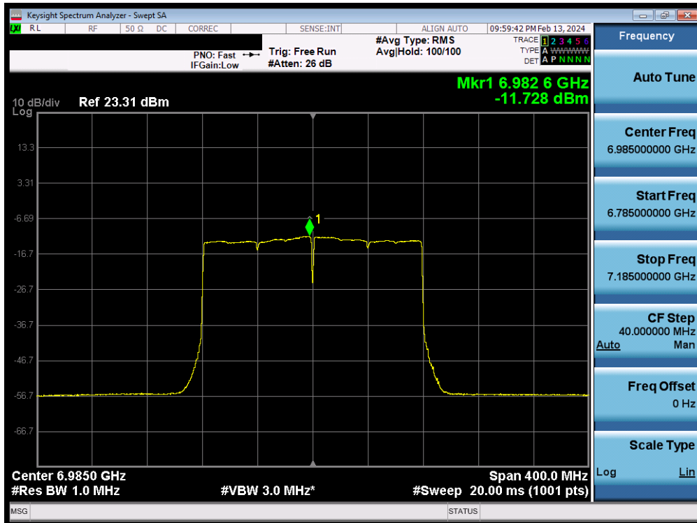
Plot 7-117. Power Spectral Density MIMO ANT2 (160MHz 802.11ax/be (UNII Band 8) – Ch. 207) - LPI
