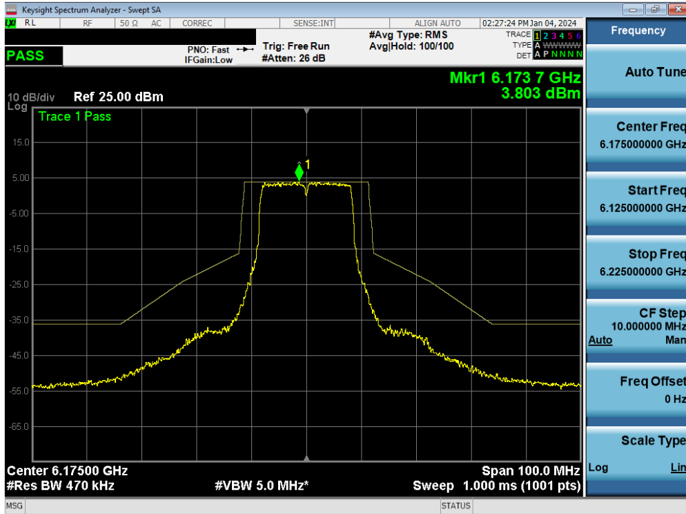
Plot 7-125. In-Band Emission MIMO ANT1 (20MHz 802.11a (UNII Band 5) – Ch. 45) - SP
