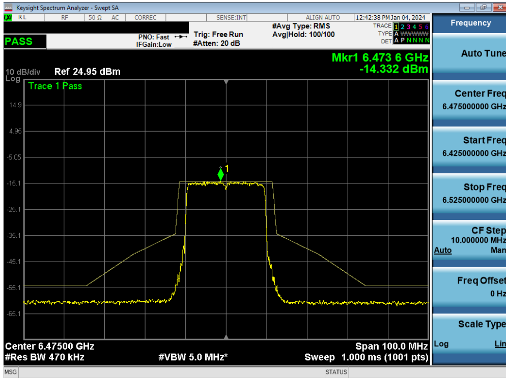
Plot 7-132. In-Band Emission MIMO ANT1 (20MHz 802.11ax/be (UNII Band 6) – Ch. 105)
