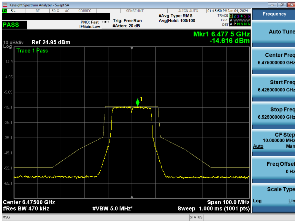
Plot 7-131. In-Band Emission MIMO ANT1 (20MHz 802.11a (UNII Band 6) – Ch. 105)
