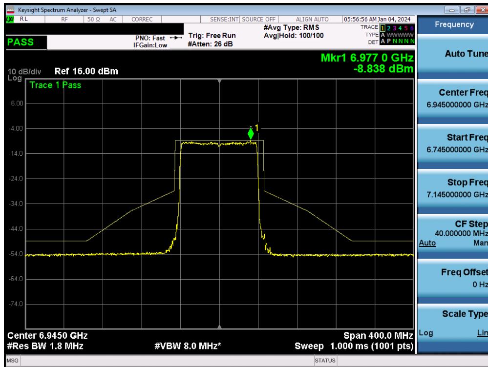
Plot 7-187. In-Band Emission MIMO ANT2 (80MHz 802.11ax/be (UNII Band 8) – Ch. 199)
