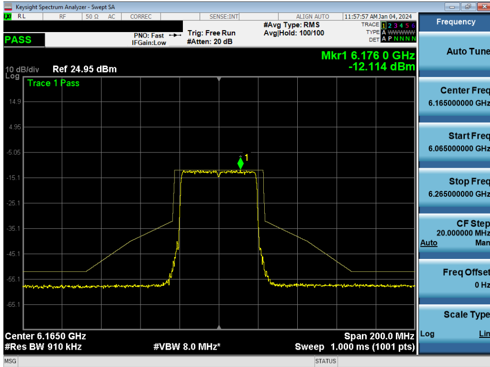
Plot 7-121. In-Band Emission MIMO ANT1 (40MHz 802.11ax/be (UNII Band 5) – Ch. 43)
