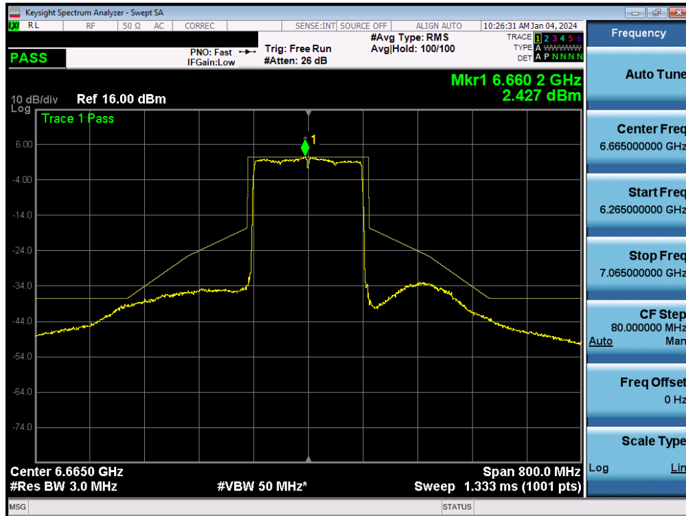
Plot 7-183. In-Band Emission MIMO ANT2 (160MHz 802.11ax/be (UNII Band 7) – Ch. 143) - SP
