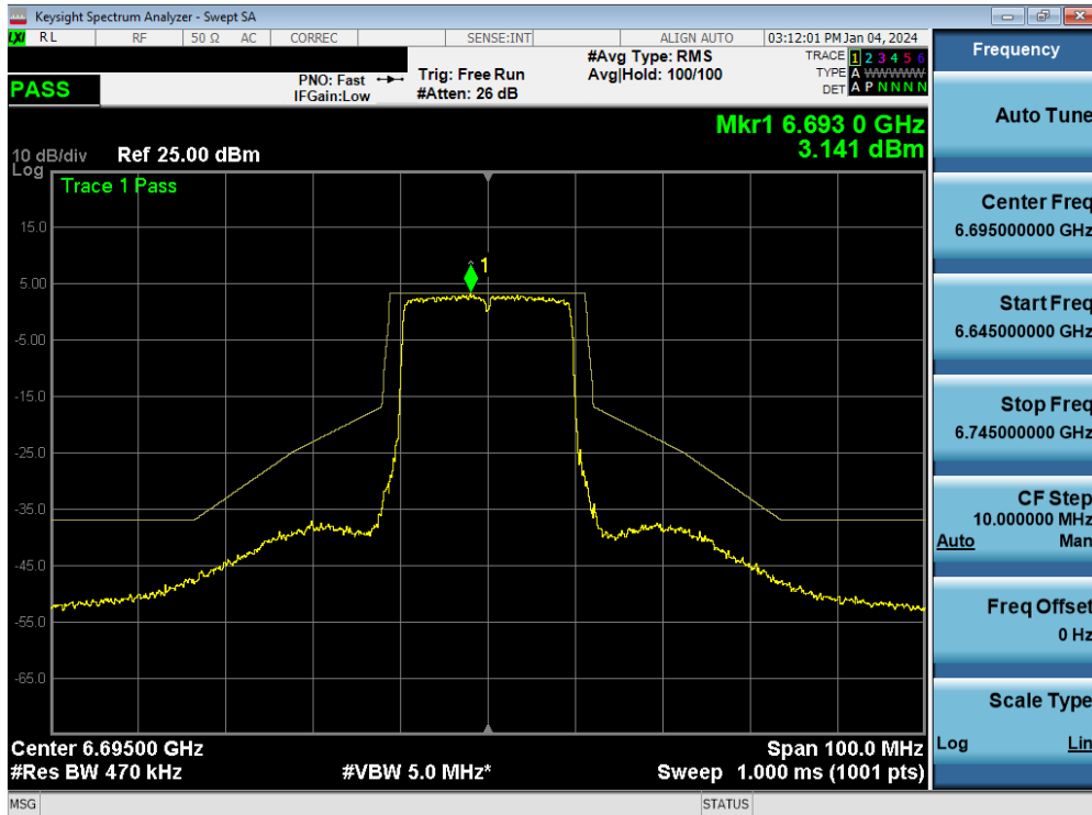
Plot 7-156. In-Band Emission MIMO ANT1 (20MHz 802.11ax/be (UNII Band 7) – Ch. 149) - SP
