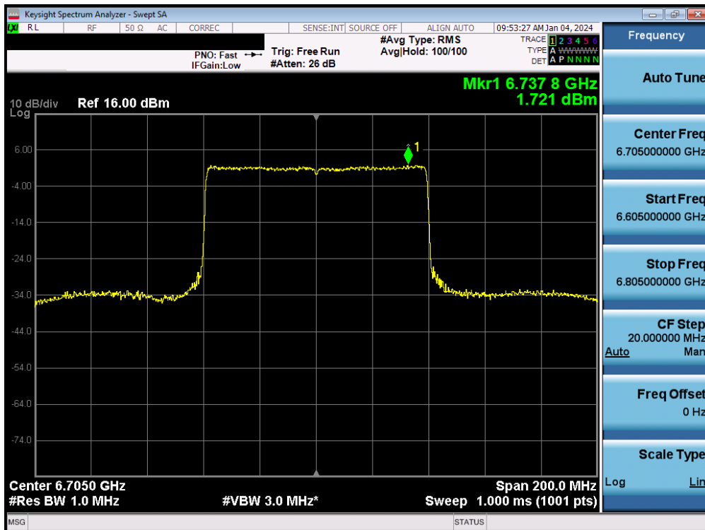
Plot 7-111. Power Spectral Density MIMO ANT2 (80MHz 802.11ax/be (UNII Band 7) – Ch. 151) - SP
