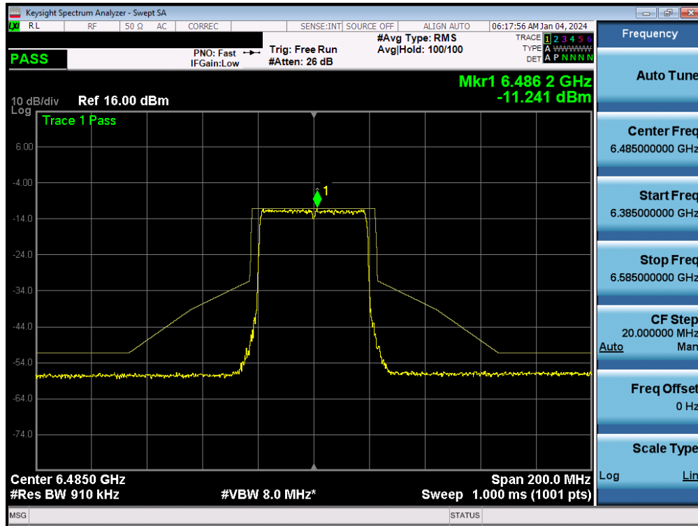
Plot 7-169. In-Band Emission MIMO ANT2 (40MHz 802.11ax/be (UNII Band 6) – Ch. 107)
