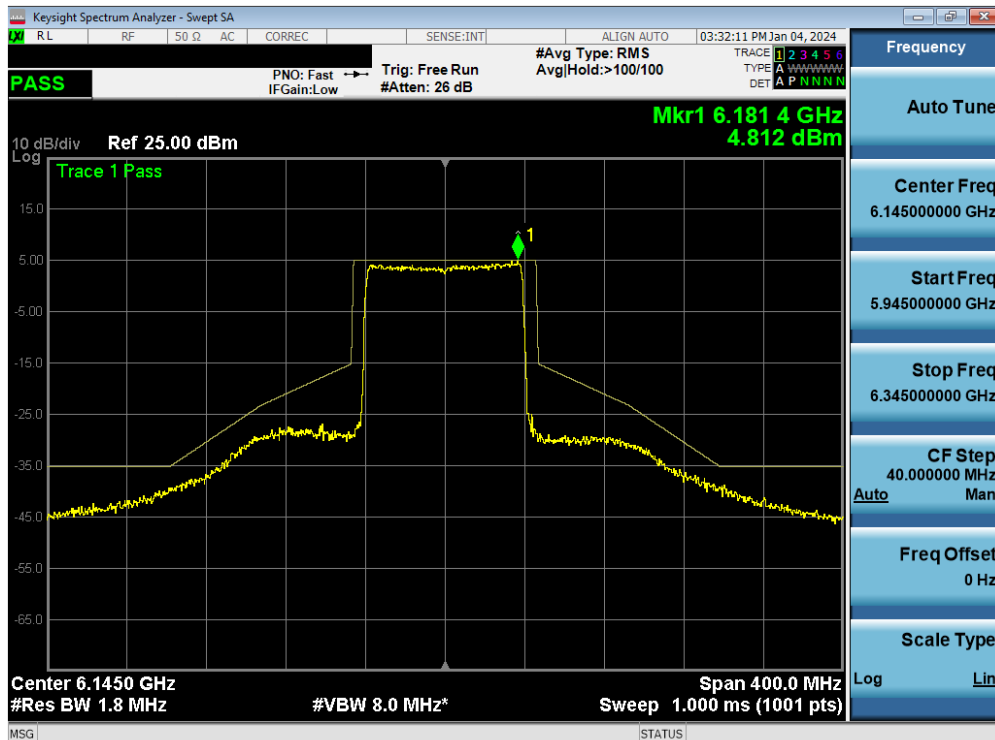
Plot 7-128. In-Band Emission MIMO ANT1 (80MHz 802.11ax/be (UNII Band 5) – Ch. 39) - SP
