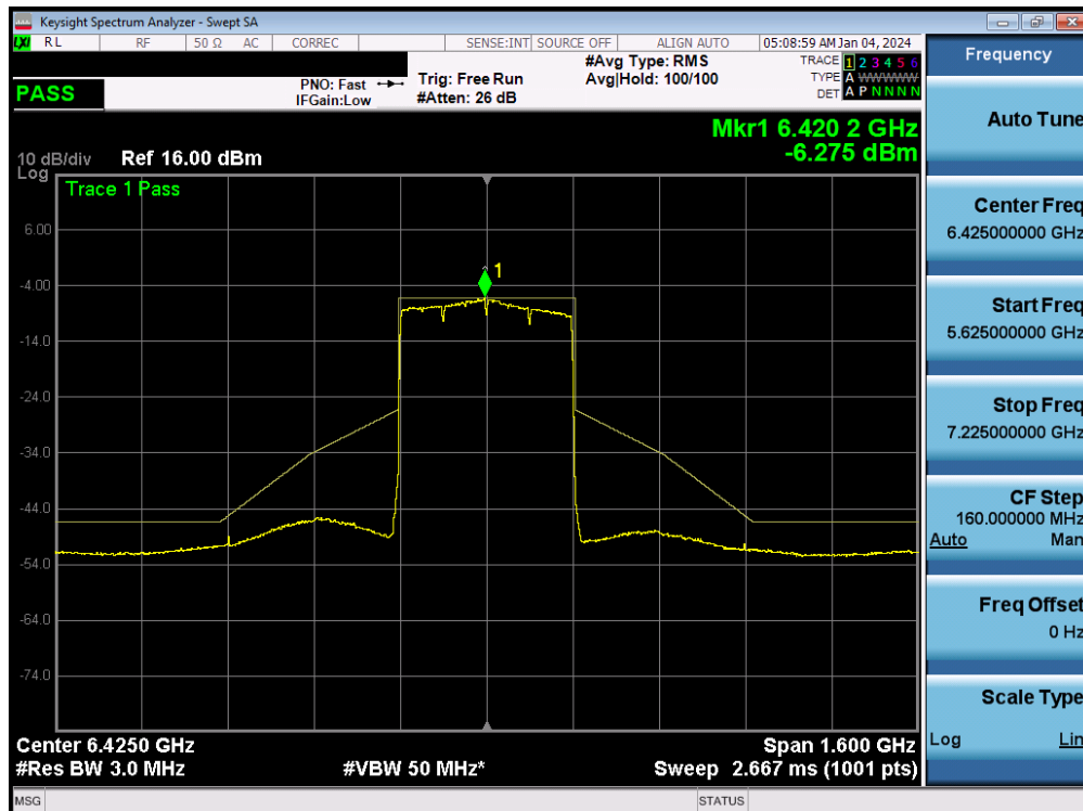
Plot 7-172. In-Band Emission MIMO ANT2 (320MHz 802.11ax/be (UNII Band 5/6/7) – Ch. 95)
