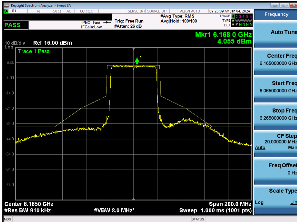
Plot 7-163. In-Band Emission MIMO ANT2 (40MHz 802.11ax/be (UNII Band 5) – Ch. 43) - SP
