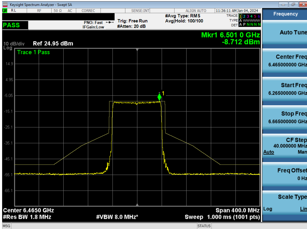
Plot 7-134. In-Band Emission MIMO ANT1 (80MHz 802.11ax/be (UNII Band 6) – Ch. 103)
