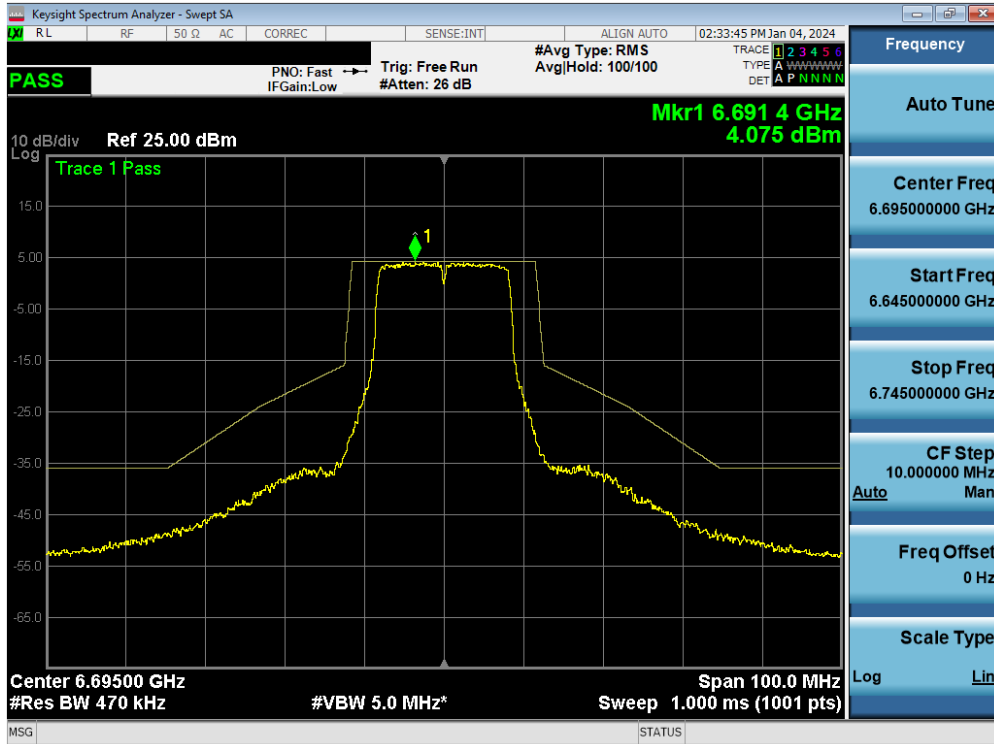
Plot 7-155. In-Band Emission MIMO ANT1 (20MHz 802.11a (UNII Band 7) – Ch. 149) - SP
