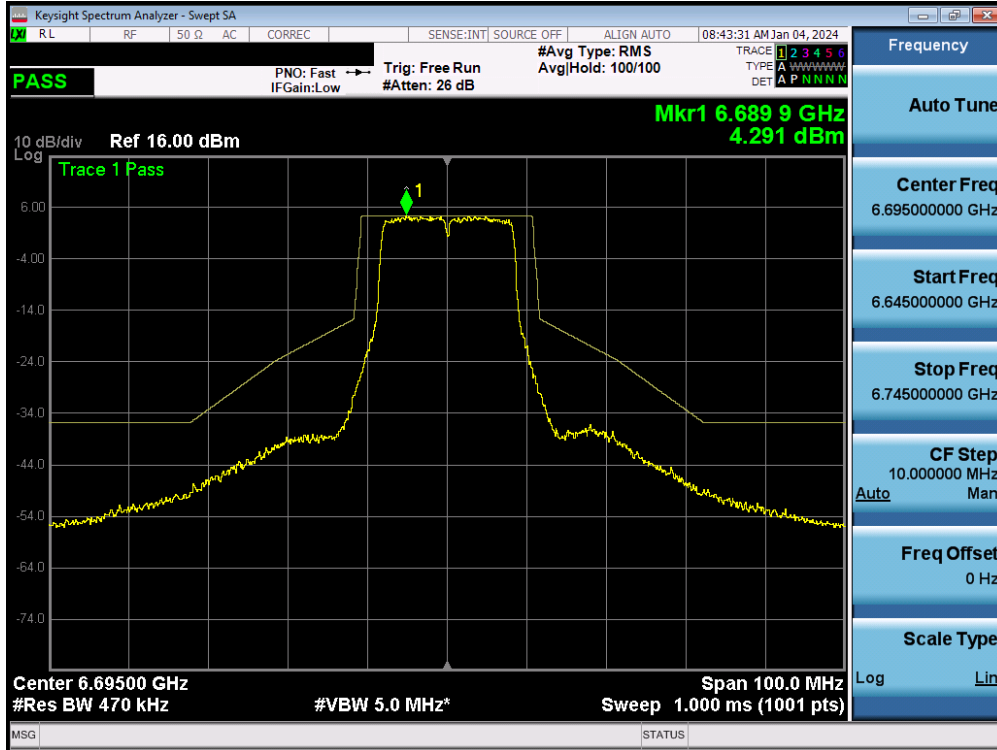
Plot 7-179. In-Band Emission MIMO ANT2 (20MHz 802.11a (UNII Band 7) – Ch. 149) - SP
