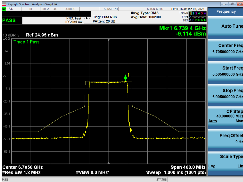
Plot 7-140. In-Band Emission MIMO ANT1 (80MHz 802.11ax/be (UNII Band 7) – Ch. 151)
