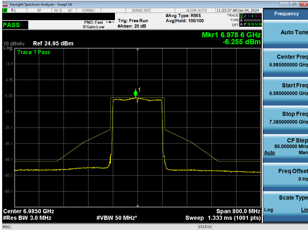
Plot 7-147. In-Band Emission MIMO ANT1 (160MHz 802.11ax/be (UNII Band 8) – Ch. 207)
