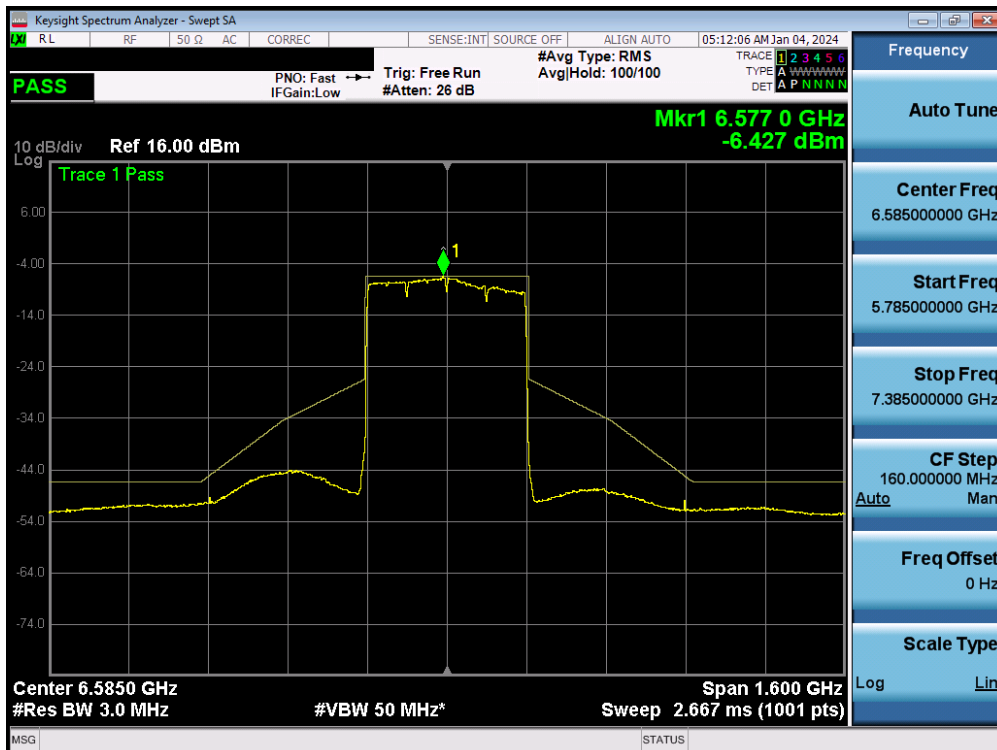
Plot 7-178. In-Band Emission MIMO ANT2 (320MHz 802.11ax/be (UNII Band 6/7) – Ch. 127)
