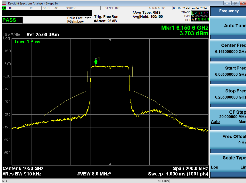
Plot 7-127. In-Band Emission MIMO ANT1 (40MHz 802.11ax/be (UNII Band 5) – Ch. 43) - SP
