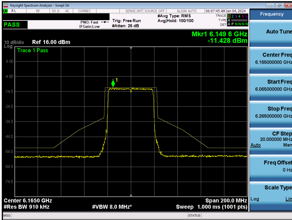
Plot 7-151. In-Band Emission MIMO ANT2 (40MHz 802.11ax/be (UNII Band 5) – Ch. 43)
