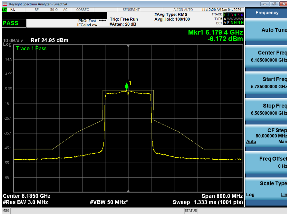
Plot 7-123. In-Band Emission MIMO ANT1 (160MHz 802.11ax/be (UNII Band 5) – Ch. 47)
