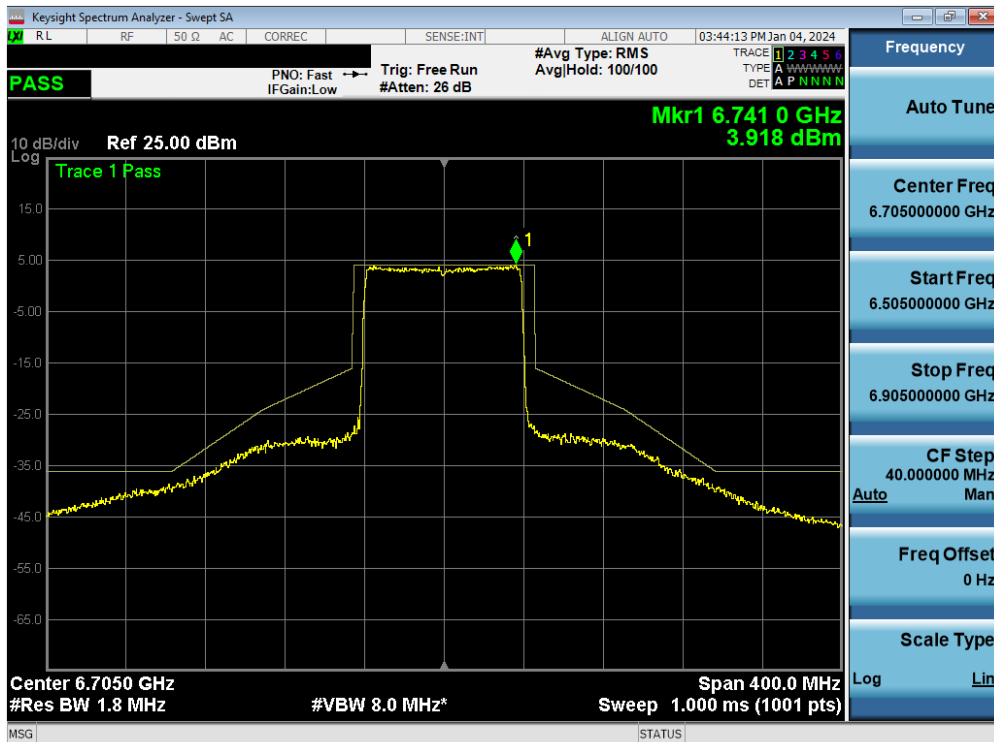
Plot 7-158. In-Band Emission MIMO ANT1 (80MHz 802.11ax/be (UNII Band 7) – Ch. 151) – SP
