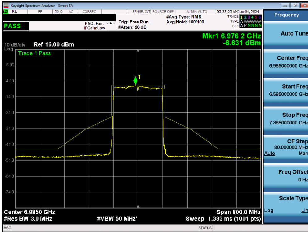
Plot 7-188. In-Band Emission MIMO ANT2 (160MHz 802.11ax/be (UNII Band 8) – Ch. 207)
