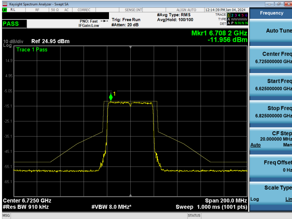
Plot 7-139. In-Band Emission MIMO ANT1 (40MHz 802.11ax/be (UNII Band 7) – Ch. 155)
