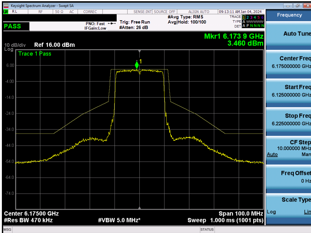
Plot 7-162. In-Band Emission MIMO ANT2 (20MHz 802.11ax/be (UNII Band 5) – Ch. 45) - SP
