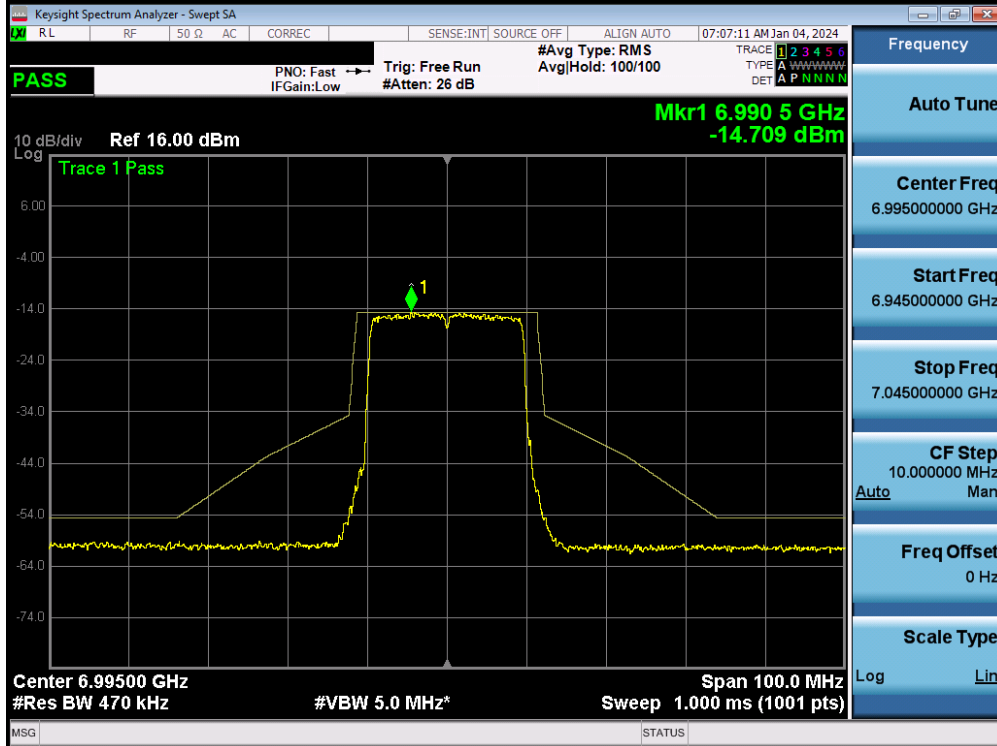
Plot 7-185. In-Band Emission MIMO ANT2 (20MHz 802.11ax/be (UNII Band 8) – Ch. 209)
