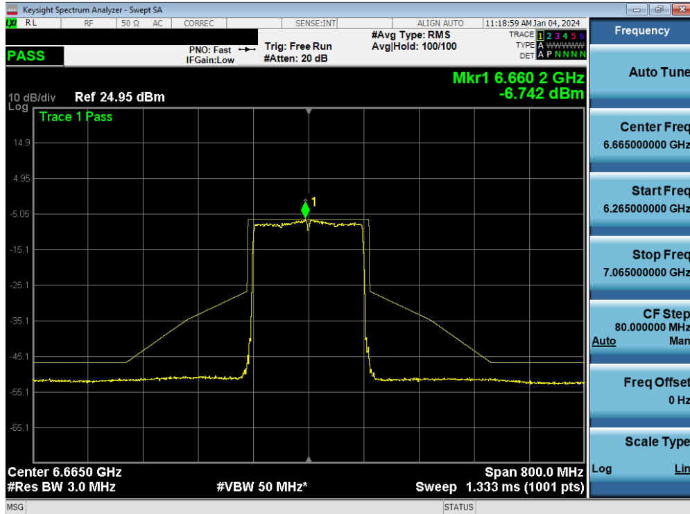
Plot 7-141. In-Band Emission MIMO ANT1 (160MHz 802.11ax/be (UNII Band 7) – Ch. 143)
