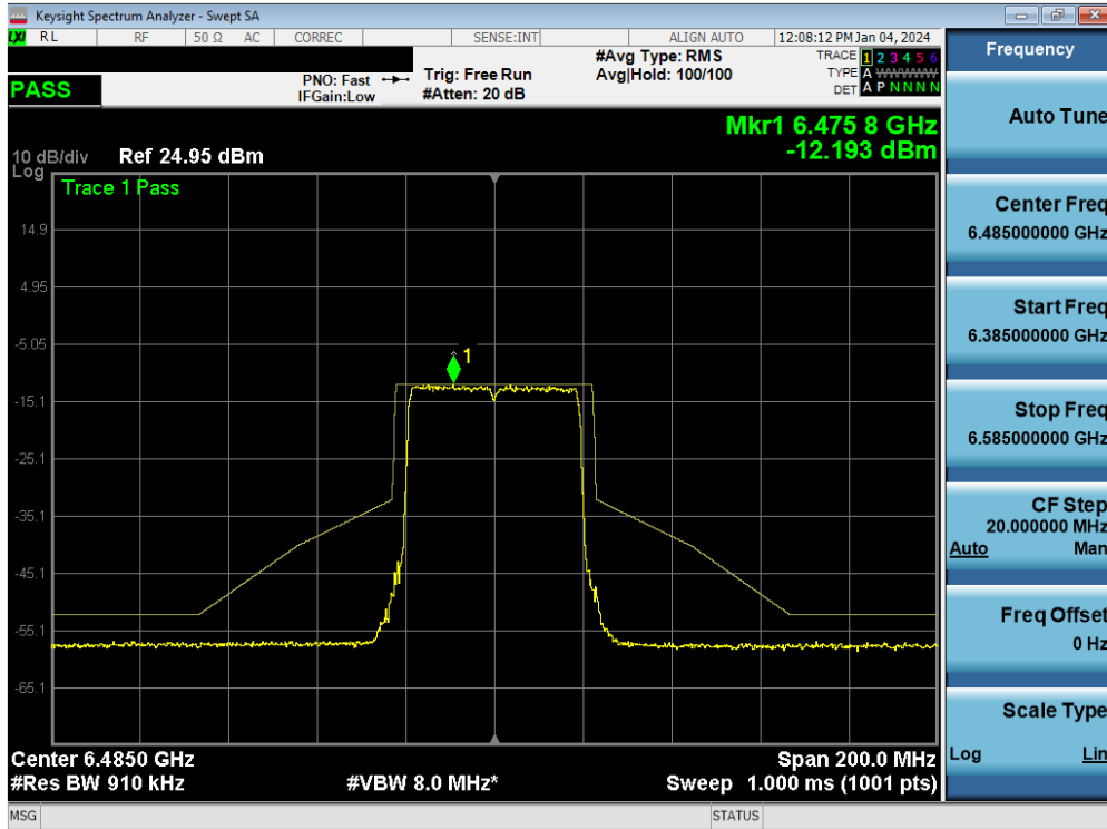
Plot 7-133. In-Band Emission MIMO ANT1 (40MHz 802.11ax/be (UNII Band 6) – Ch. 107)
