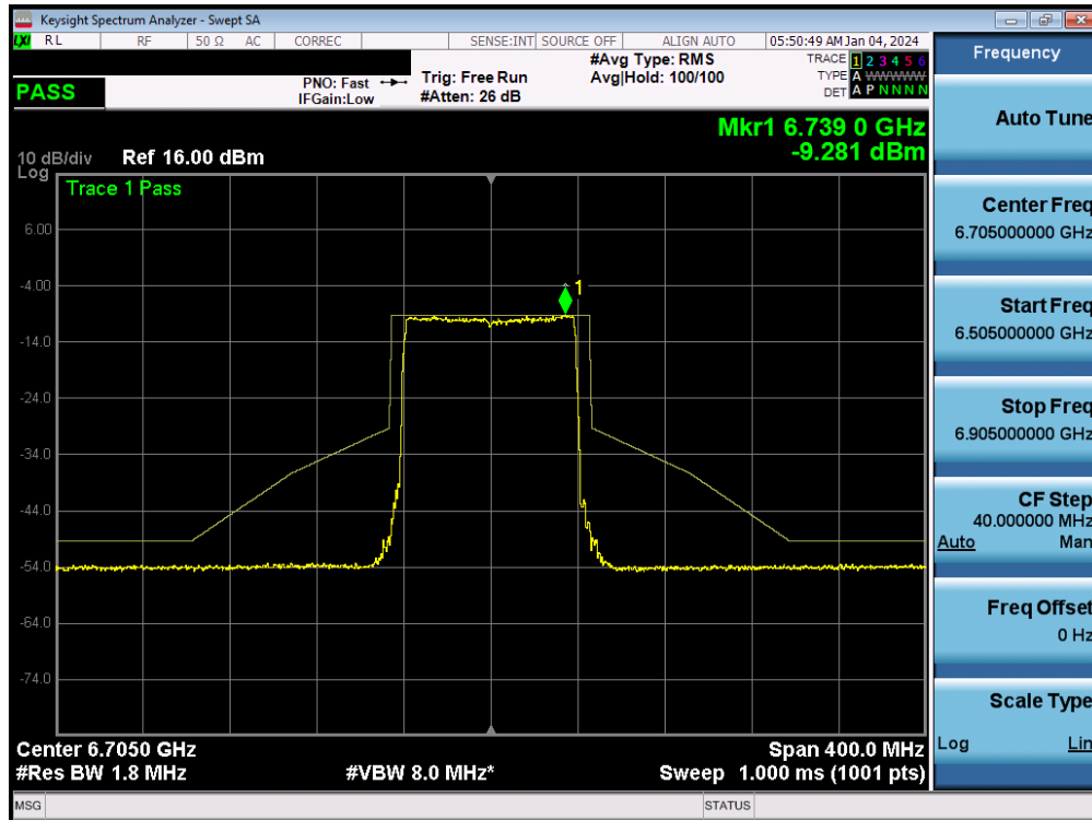
Plot 7-176. In-Band Emission MIMO ANT2 (80MHz 802.11ax/be (UNII Band 7) – Ch. 151)
