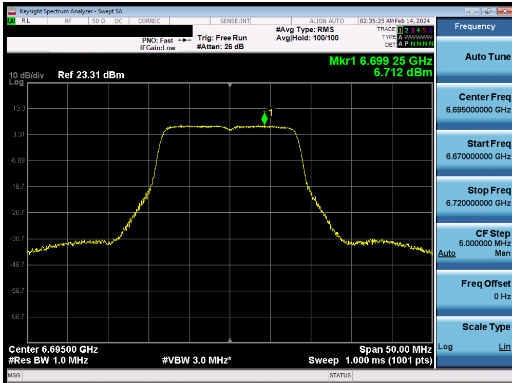
Plot 7-108. Power Spectral Density MIMO ANT2 (20MHz 802.11a (UNII Band 7) – Ch. 149) - SP
