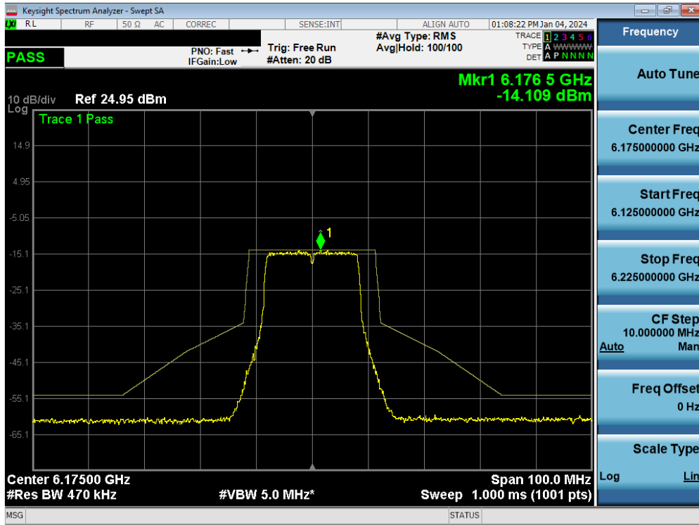
Plot 7-119. In-Band Emission MIMO ANT1 (20MHz 802.11a (UNII Band 5) – Ch. 45)
