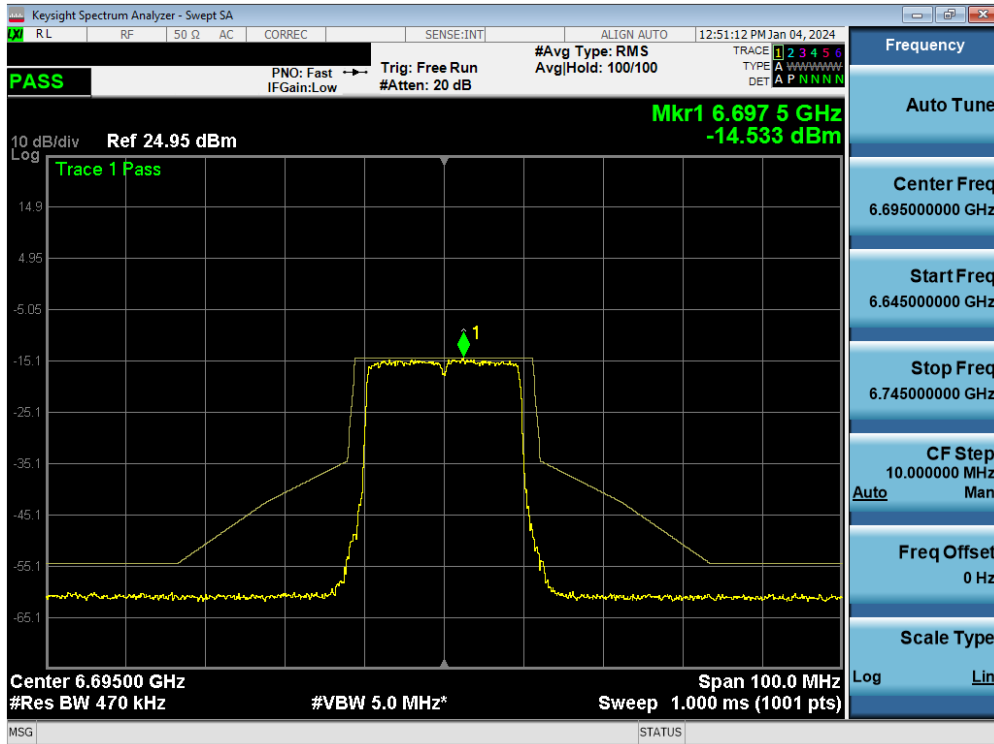
Plot 7-138. In-Band Emission MIMO ANT1 (20MHz 802.11ax/be (UNII Band 7) – Ch. 149)
