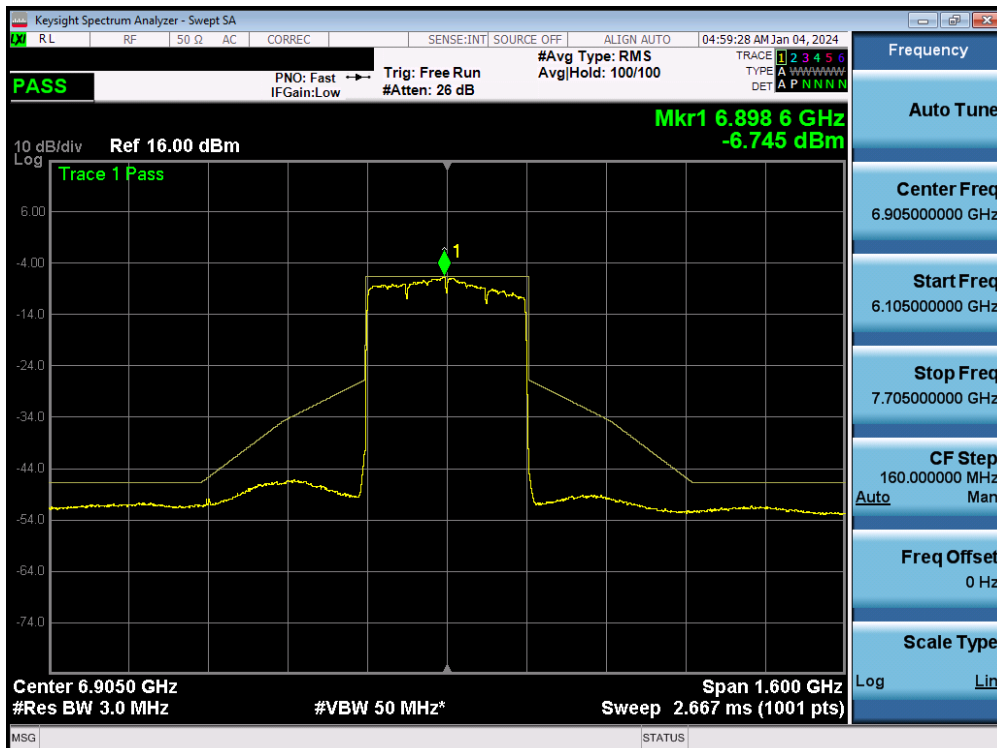
Plot 7-189. In-Band Emission MIMO ANT2 (320MHz 802.11ax/be (UNII Band 7/8) – Ch. 191)
