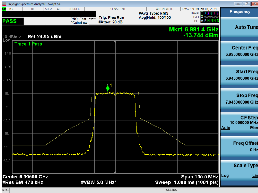
Plot 7-144. In-Band Emission MIMO ANT1 (20MHz 802.11ax/be (UNII Band 8) – Ch. 209)
