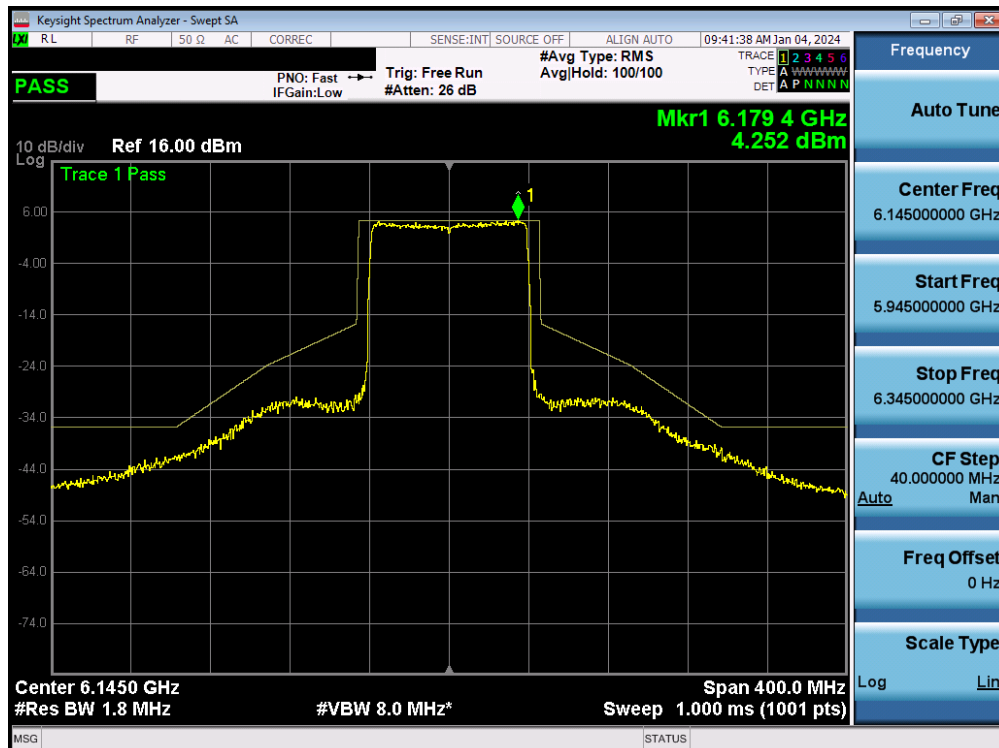
Plot 7-164. In-Band Emission MIMO ANT2 (80MHz 802.11ax/be (UNII Band 5) – Ch. 39) - SP
