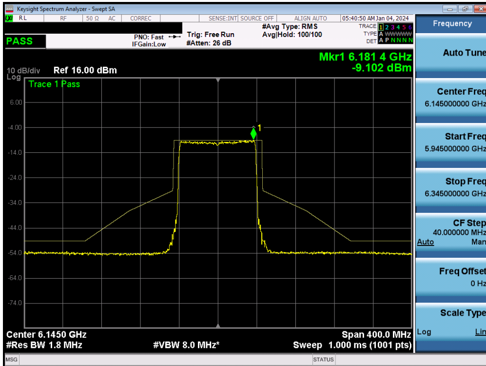
Plot 7-152. In-Band Emission MIMO ANT2 (80MHz 802.11ax/be (UNII Band 5) – Ch. 39)
