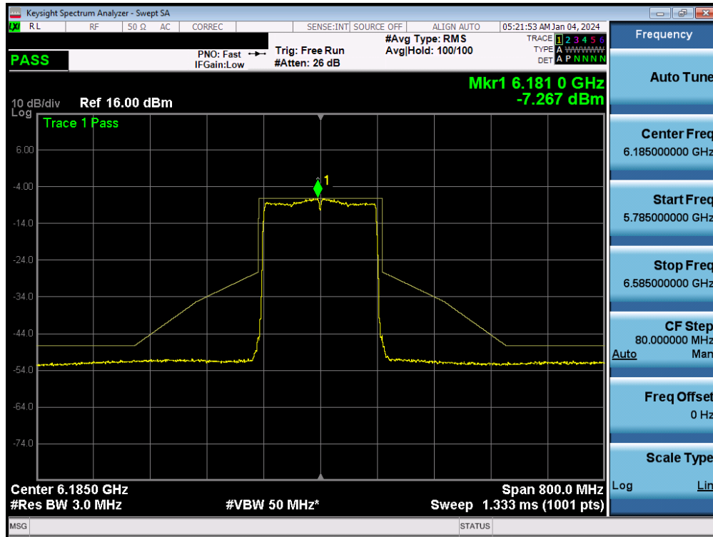
Plot 7-153. In-Band Emission MIMO ANT2 (160MHz 802.11ax/be (UNII Band 5) – Ch. 47)
