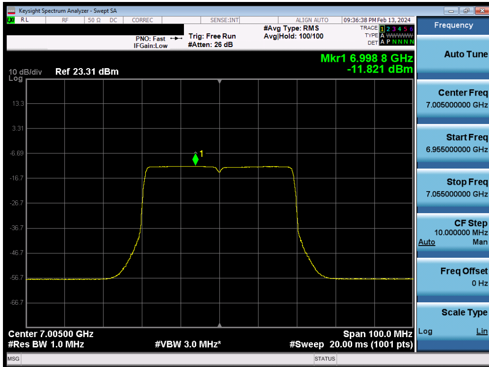
Plot 7-115. Power Spectral Density MIMO ANT2 (40MHz 802.11ax/be (UNII Band 8) – Ch. 211) - LPI
