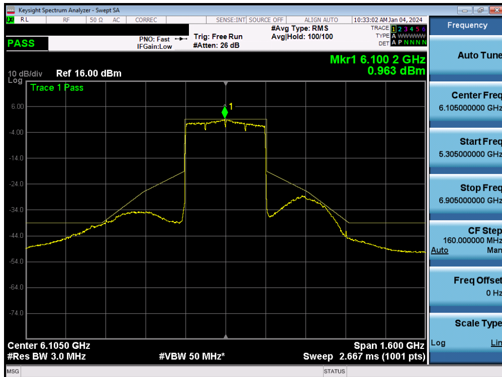
Plot 7-166. In-Band Emission MIMO ANT2 (320MHz 802.11ax/be (UNII Band 5) – Ch.31) - SP
