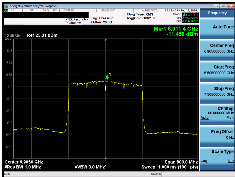
Plot 7-118. Power Spectral Density MIMO ANT2 (320MHz 802.11ax/be (UNII Band 7/8) – Ch. 191) - LPI
