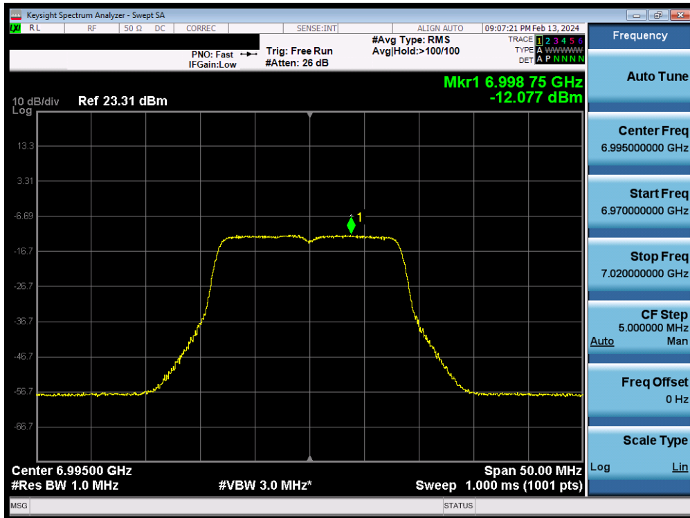
Plot 7-113. Power Spectral Density MIMO ANT2 (20MHz 802.11a (UNII Band 8) – Ch. 209) - LPI
