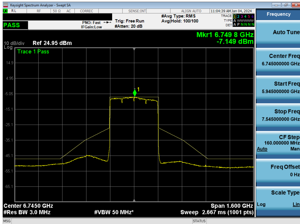
Plot 7-160. In-Band Emission MIMO ANT1 (320MHz 802.11ax/be (UNII Band 6/7) – Ch. 159) - SP
