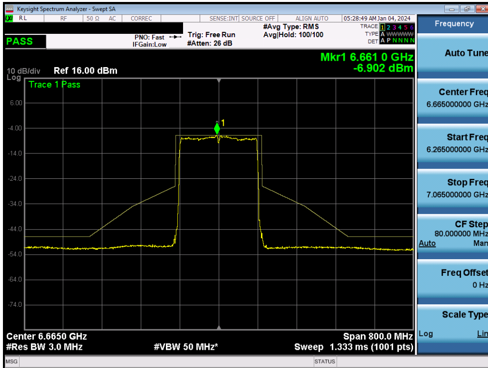
Plot 7-177. In-Band Emission MIMO ANT2 (160MHz 802.11ax/be (UNII Band 7) – Ch. 143)
