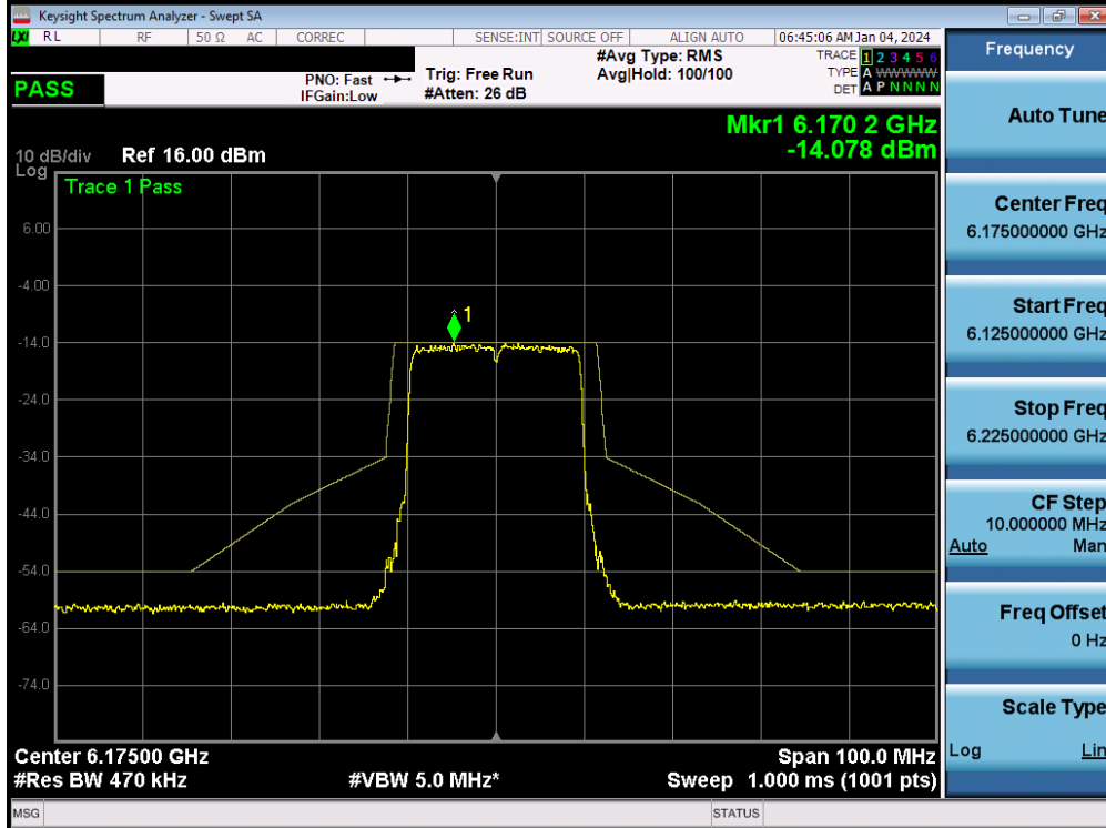
Plot 7-150. In-Band Emission MIMO ANT2 (20MHz 802.11ax/be (UNII Band 5) – Ch. 45)
