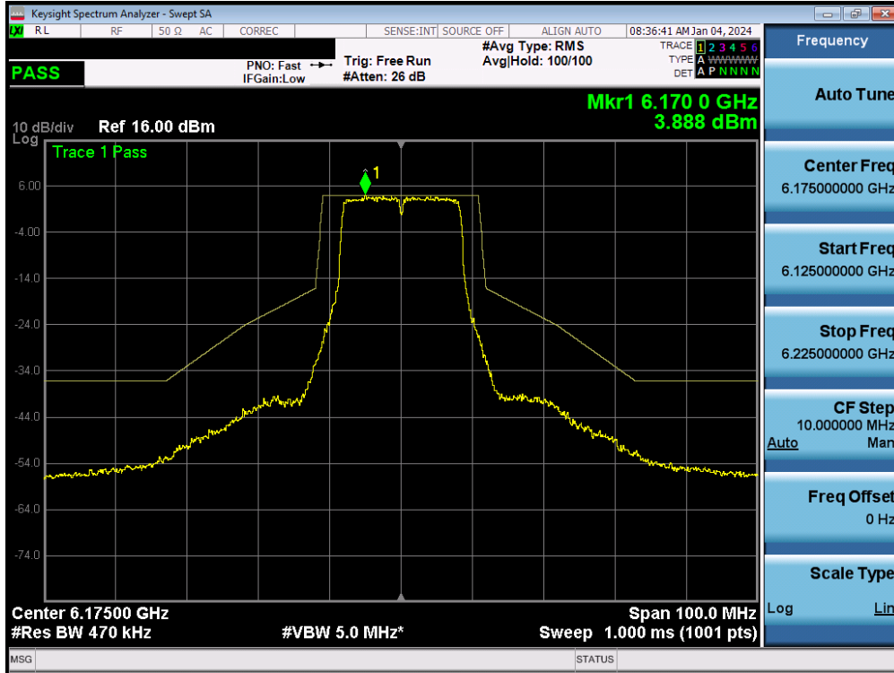
Plot 7-161. In-Band Emission MIMO ANT2 (20MHz 802.11a (UNII Band 5) – Ch. 45) - SP
