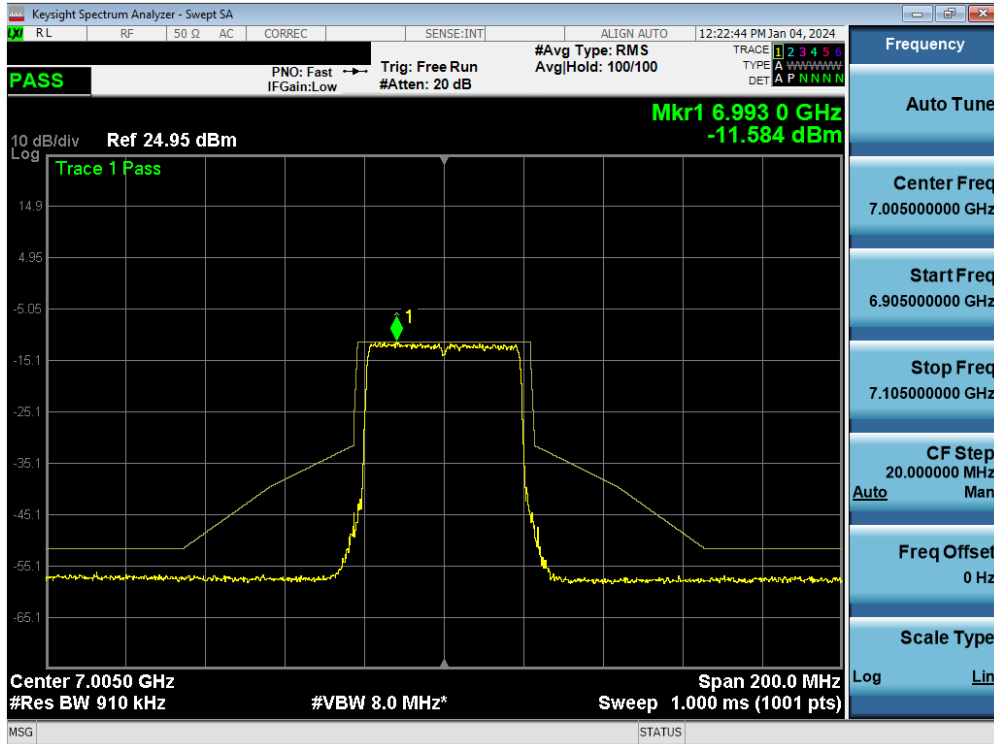
Plot 7-145. In-Band Emission MIMO ANT1 (40MHz 802.11ax/be (UNII Band 8) – Ch. 211)
