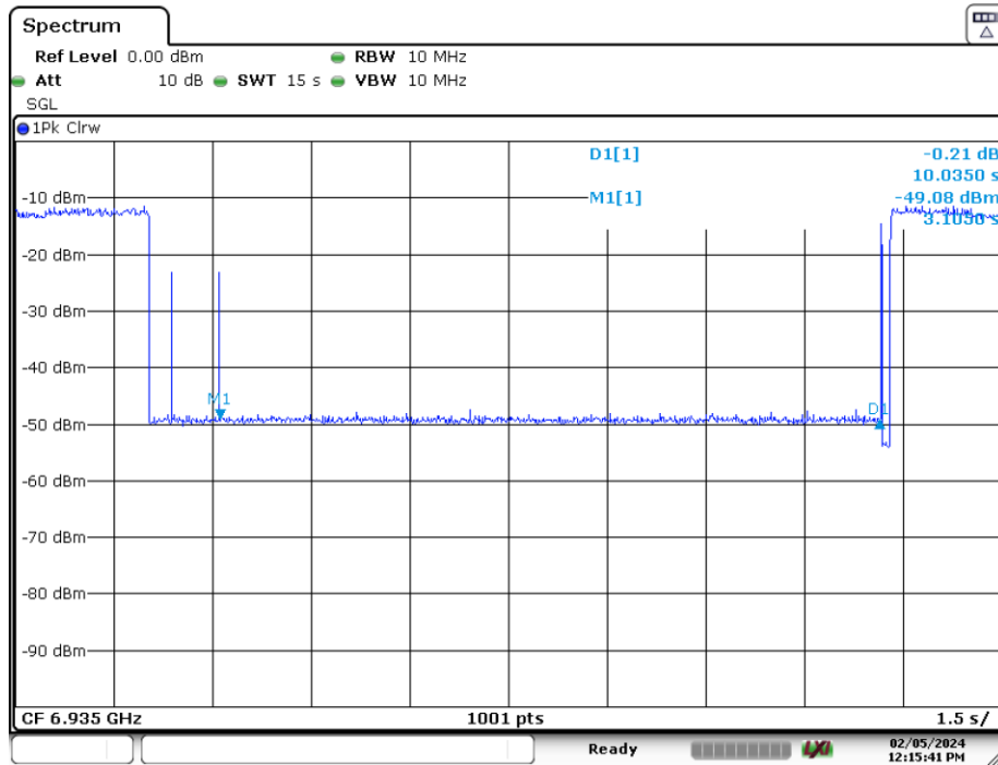
Plot 7-203. Contention Based Protocol Timing Plot (20MHz (UNII Band 8) – Ch. 197)
