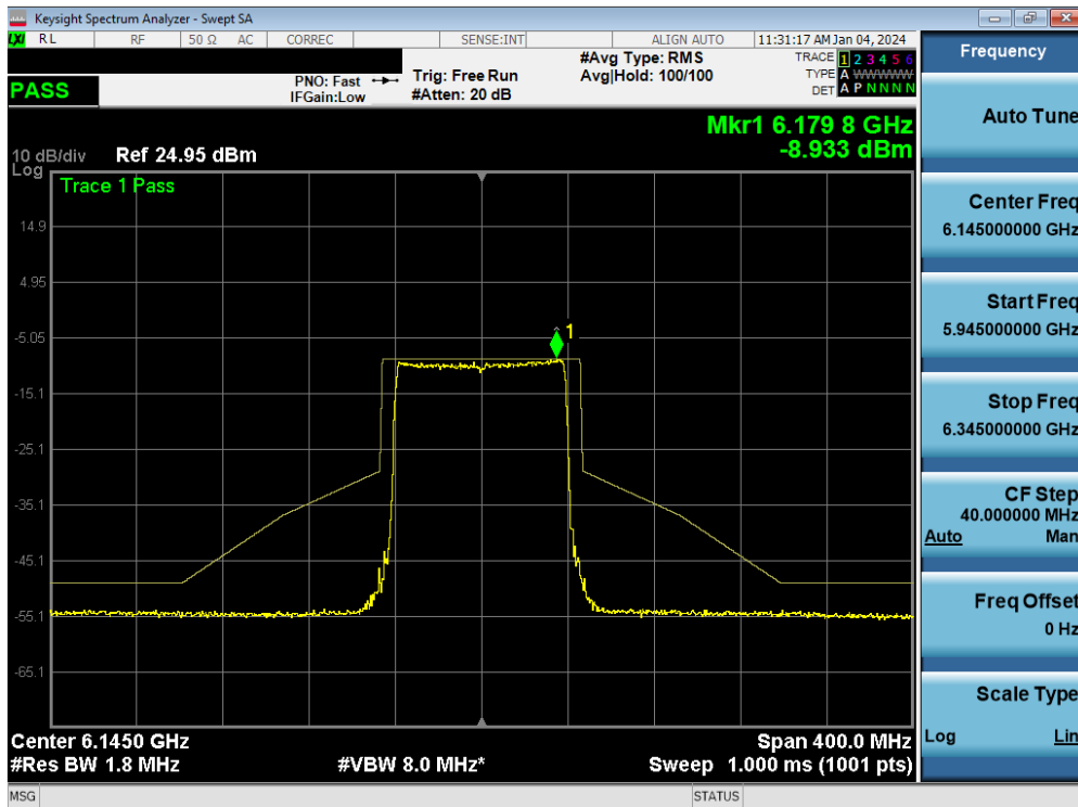
Plot 7-122. In-Band Emission MIMO ANT1 (80MHz 802.11ax/be (UNII Band 5) – Ch. 39)
