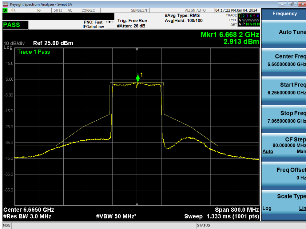
Plot 7-159. In-Band Emission MIMO ANT1 (160MHz 802.11ax/be (UNII Band 7) – Ch. 143) - SP
