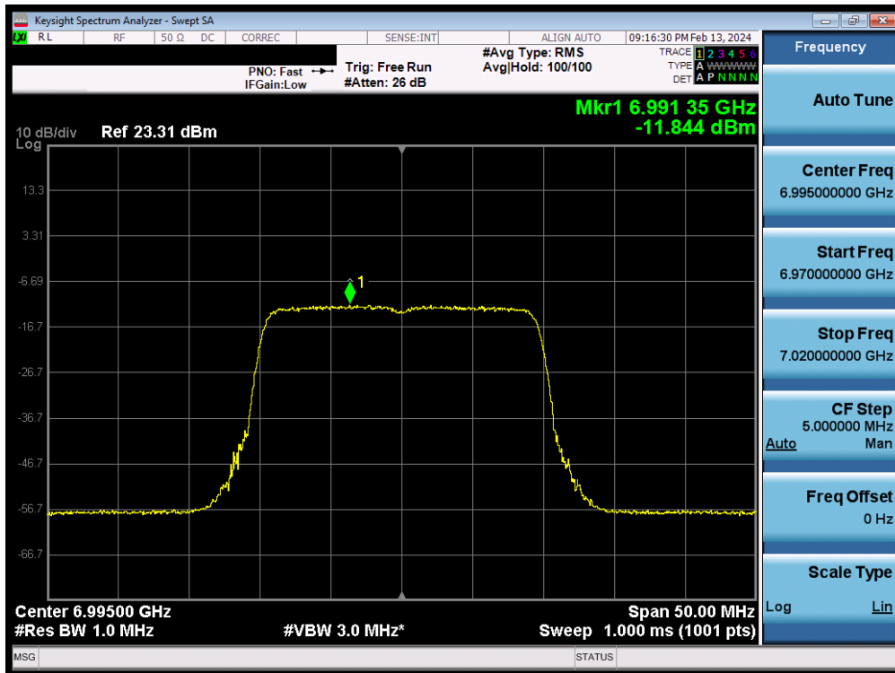
Plot 7-114. Power Spectral Density MIMO ANT2 (20MHz 802.11ax/be (UNII Band 8) – Ch. 209) - LPI
