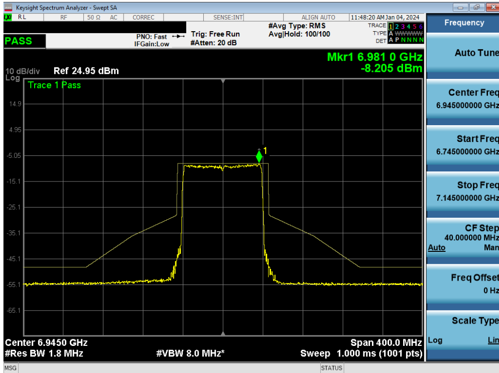
Plot 7-146. In-Band Emission MIMO ANT1 (80MHz 802.11ax/be (UNII Band 8) – Ch. 199)
