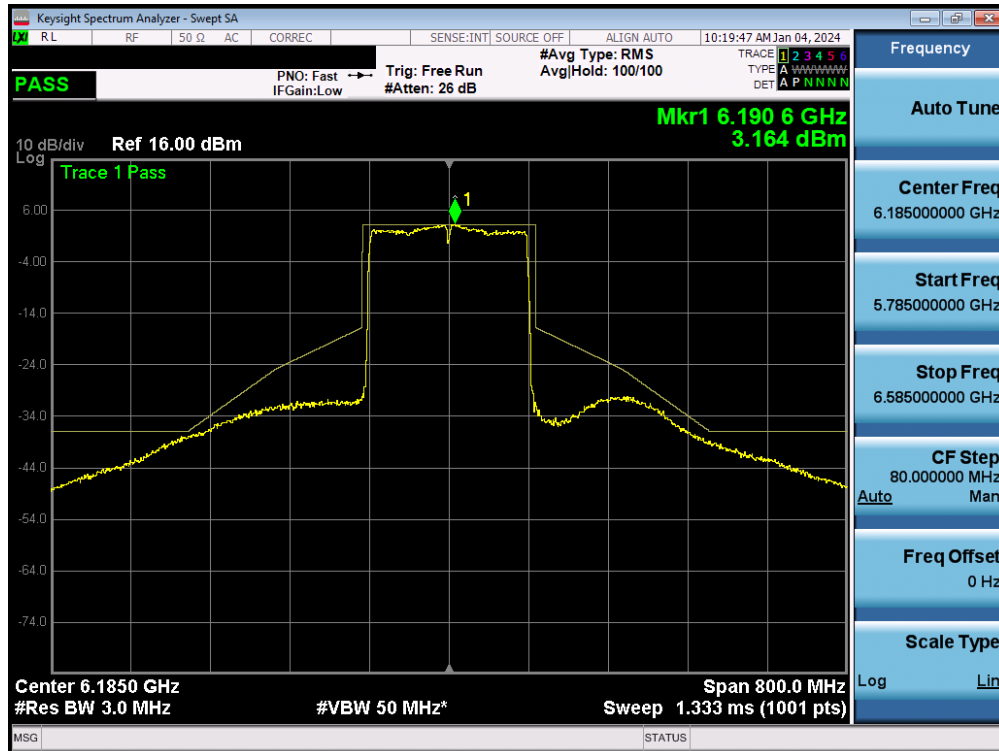
Plot 7-165. In-Band Emission MIMO ANT2 (160MHz 802.11ax/be (UNII Band 5) – Ch. 47) - SP
