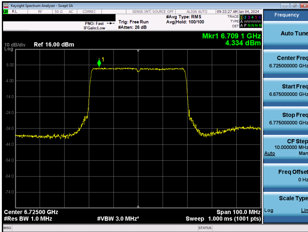
Plot 7-110. Power Spectral Density MIMO ANT2 (40MHz 802.11ax/be (UNII Band 7) – Ch. 155) - SP
