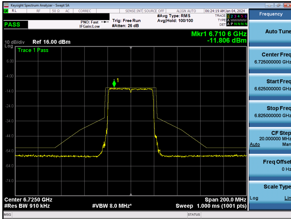
Plot 7-175. In-Band Emission MIMO ANT2 (40MHz 802.11ax/be (UNII Band 7) – Ch. 155)
