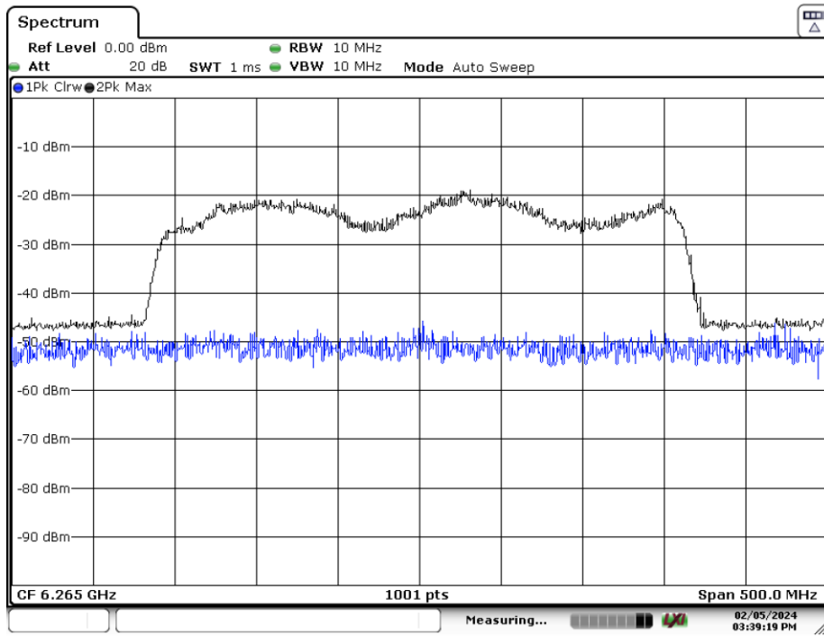
Plot 7-208. CBP 320MHz Channel - Injection Center – [6265 MHz]
