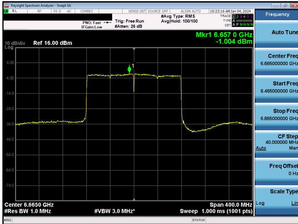
Plot 7-112. Power Spectral Density MIMO ANT2 (160MHz 802.11ax/be (UNII Band 7) – Ch. 143) - SP
