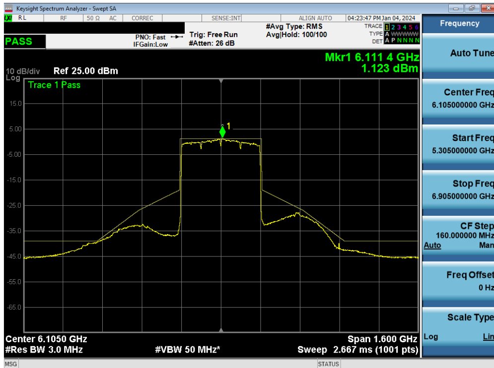
Plot 7-130. In-Band Emission MIMO ANT1 (320MHz 802.11ax/be (UNII Band 5) – Ch.31) – SP
