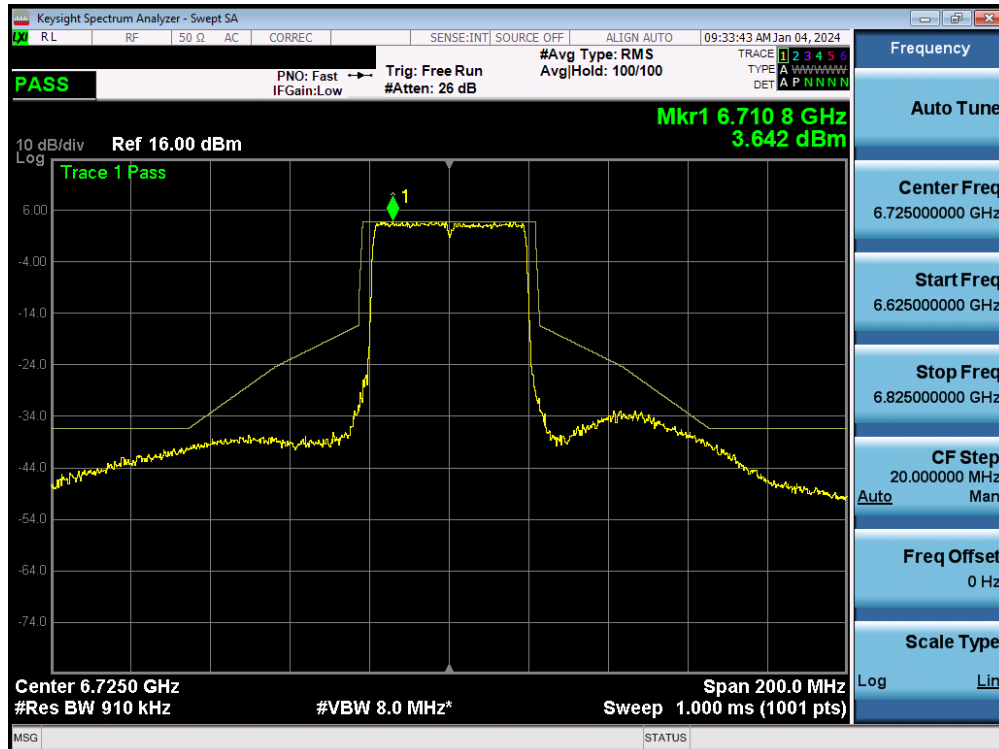
Plot 7-181. In-Band Emission MIMO ANT2 (40MHz 802.11ax/be (UNII Band 7) – Ch. 155) – SP
