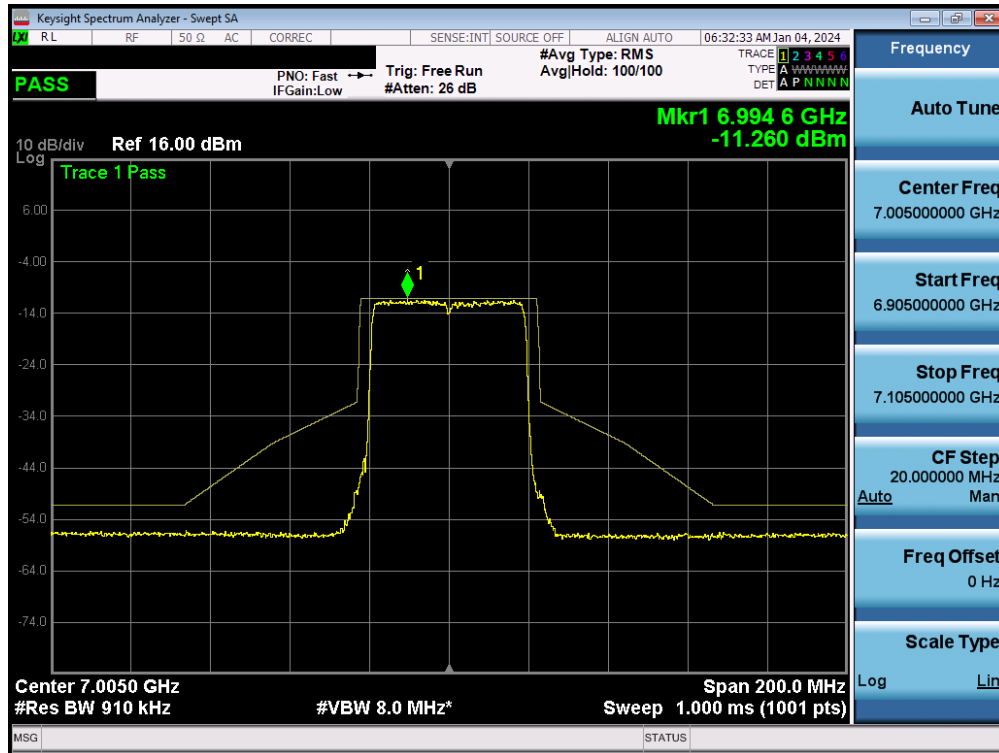
Plot 7-186. In-Band Emission MIMO ANT2 (40MHz 802.11ax/be (UNII Band 8) – Ch. 211)
