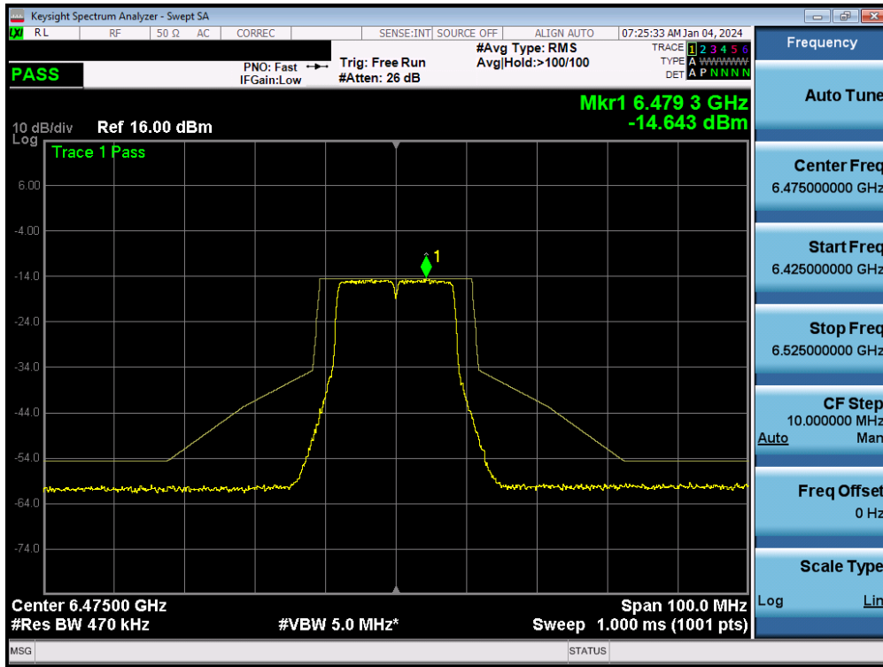
Plot 7-167. In-Band Emission MIMO ANT2 (20MHz 802.11a (UNII Band 6) – Ch. 105)
