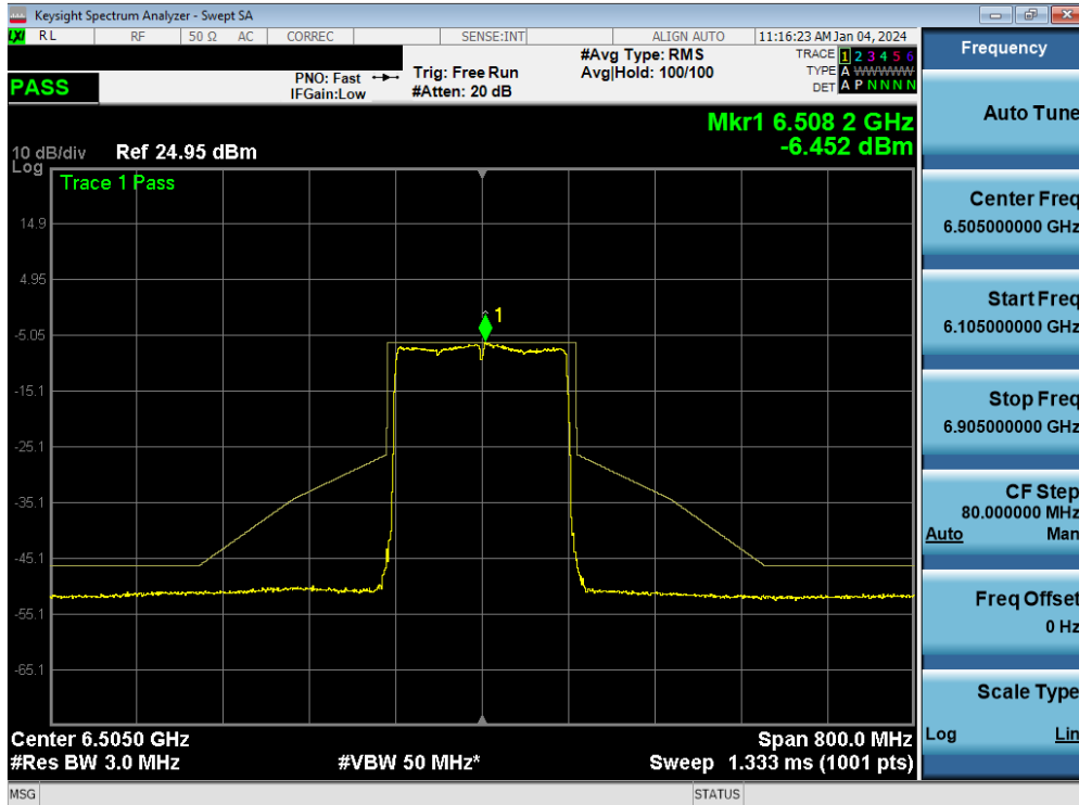
Plot 7-135. In-Band Emission MIMO ANT1 (160MHz 802.11ax/be (UNII Band 6) – Ch. 111)
