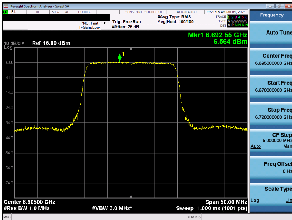
Plot 7-109. Power Spectral Density MIMO ANT2 (20MHz 802.11ax/be (UNII Band 7) – Ch. 149) - SP
